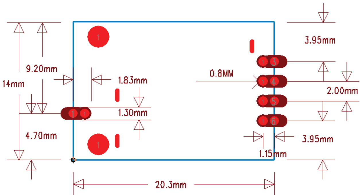
Figure 6 Module dimension
