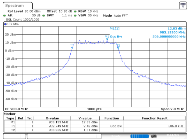
Lora 500k_Low_Channel
