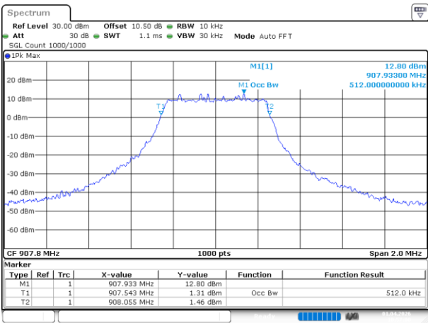
Lora 500k_Middle_Channel
