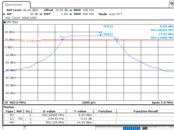
Lora 500k_Low_Channel
