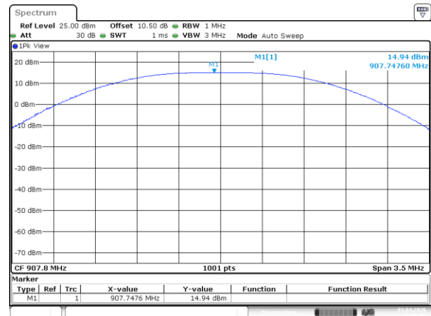
Lora 500k_Middle_Channel
