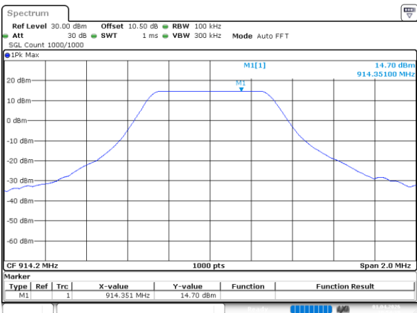
Lora 500k_High_Channel
