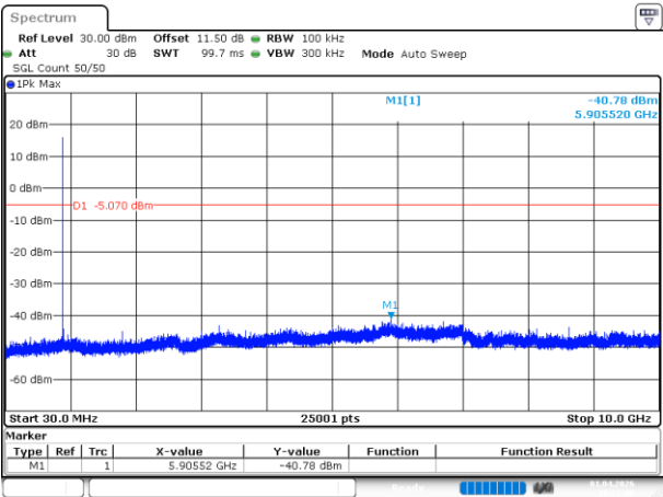
Lora 500k_Low_Channel
