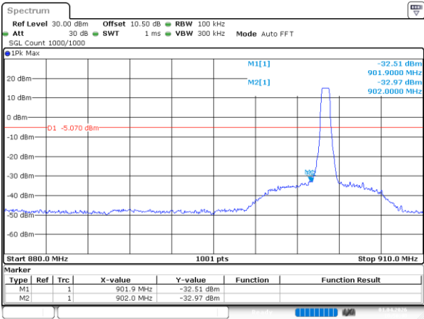
Lora 500k_Low_Channel
