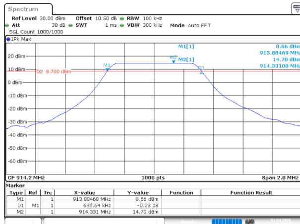
Lora 500k_High_Channel
