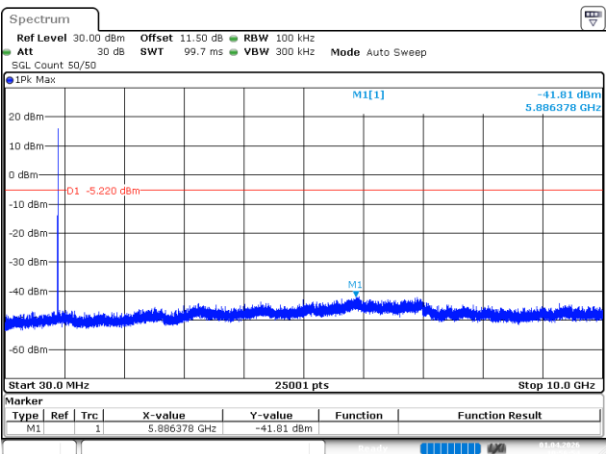
Lora 500k_Middle_Channel
