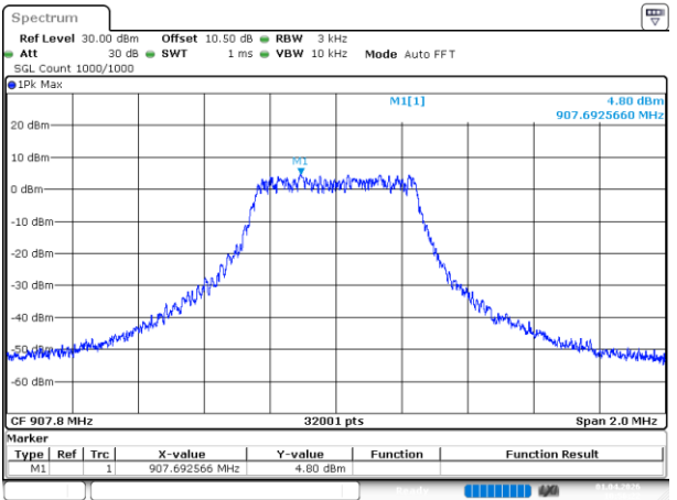
Lora 500k_Middle_Channel
