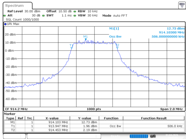
Lora 500k_High_Channel
