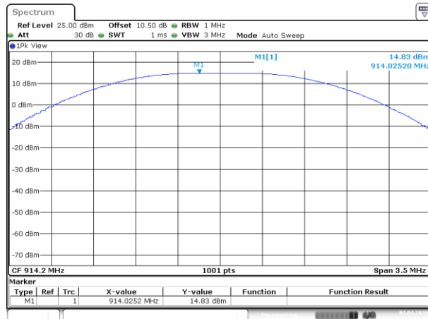
Lora 500k_High_Channel
