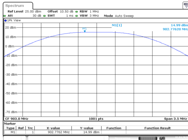
Lora 500k_Low_Channel
