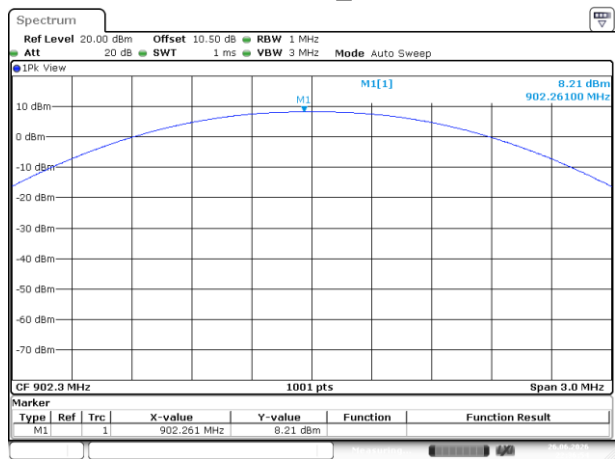
Lora 125k_Low
