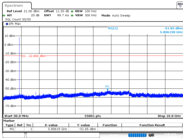
Lora 125k_High
