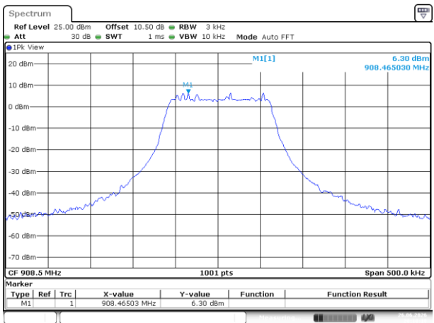
Lora 125k_Middle
