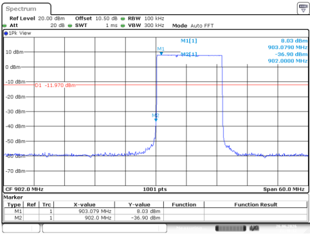
Lora 125k_Hopping_Lower
