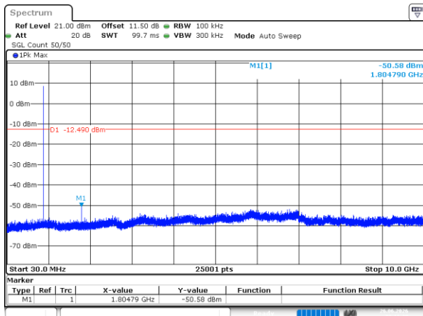
Lora 125k_Low
