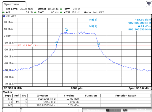
Lora 125k_Low
