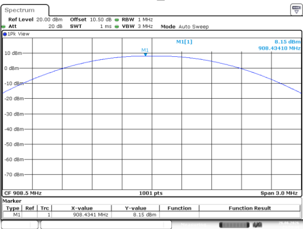
Lora 125k_Middle
