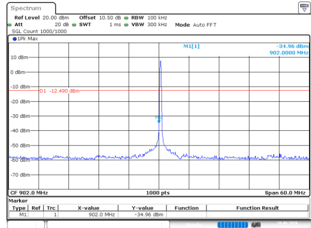
Lora 125k_Low
