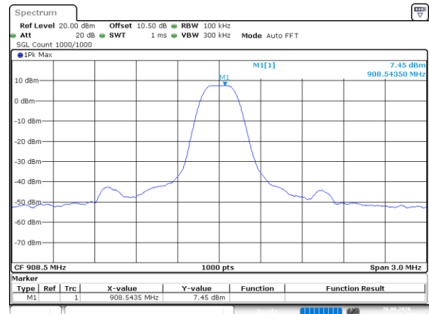
Lora 125k_Middle
