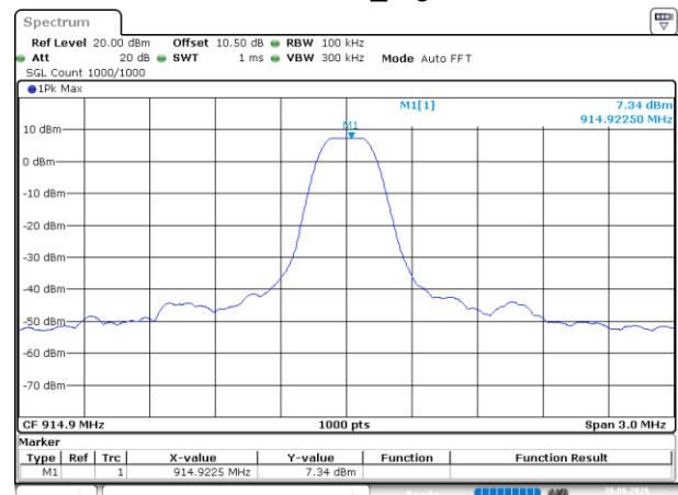
Lora 125k_High
