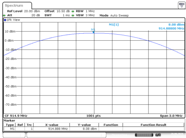
Lora 125k_High
