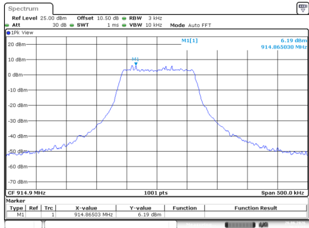
Lora 125k_High
