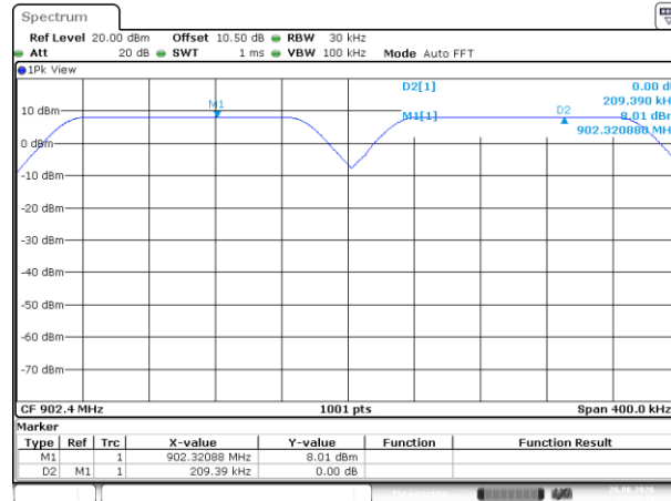
Lora 125k_Middle
