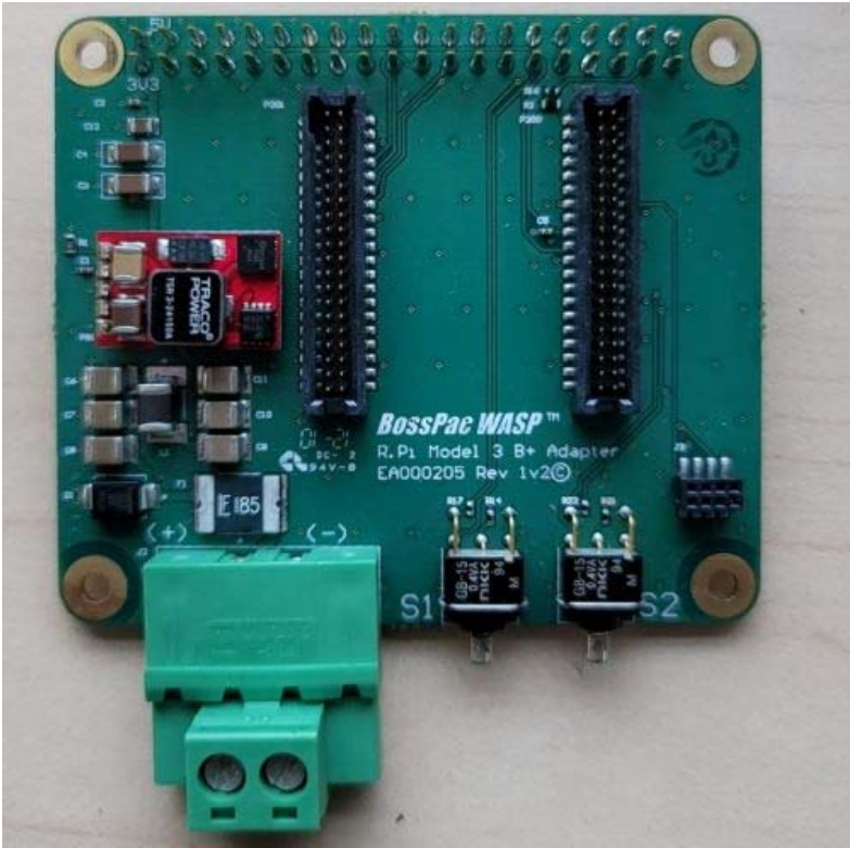
Figure E23.2 – Internal, Top PCB, Top, Module Removed
