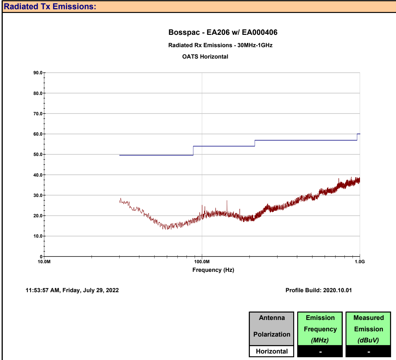
Plot 10.3 – Radiated Rx Emissions, 30 - 1000MHz, EA000406, Horizontal
