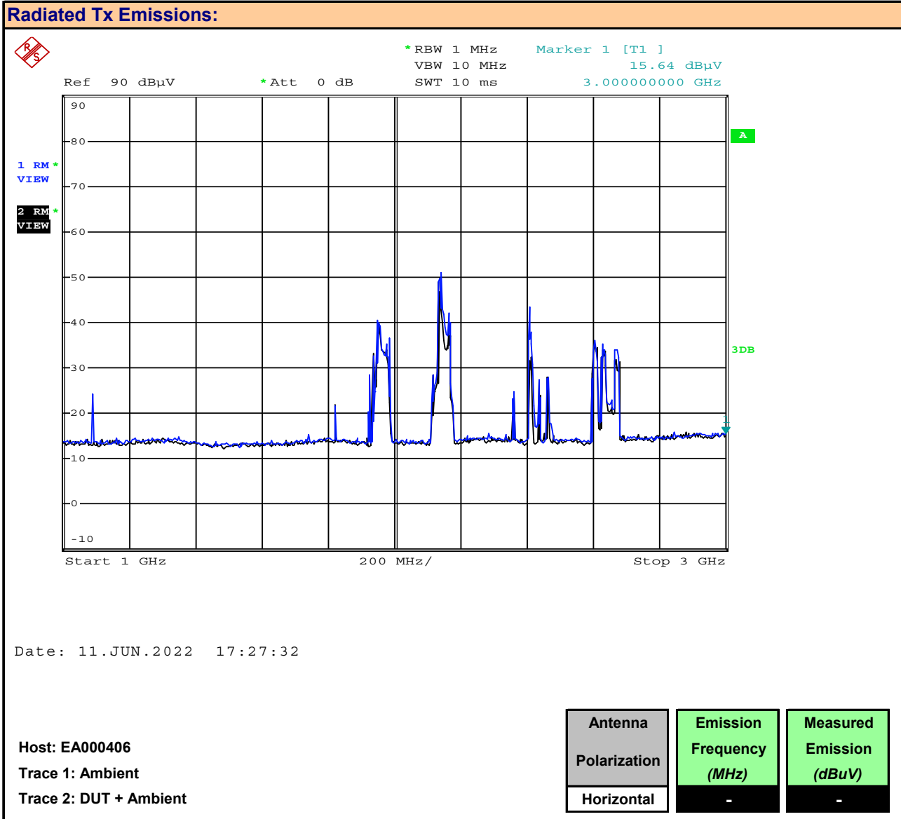
Plot 9.11 – Radiated Tx Emissions, 1 – 3GHz, EA000406, Horizontal
