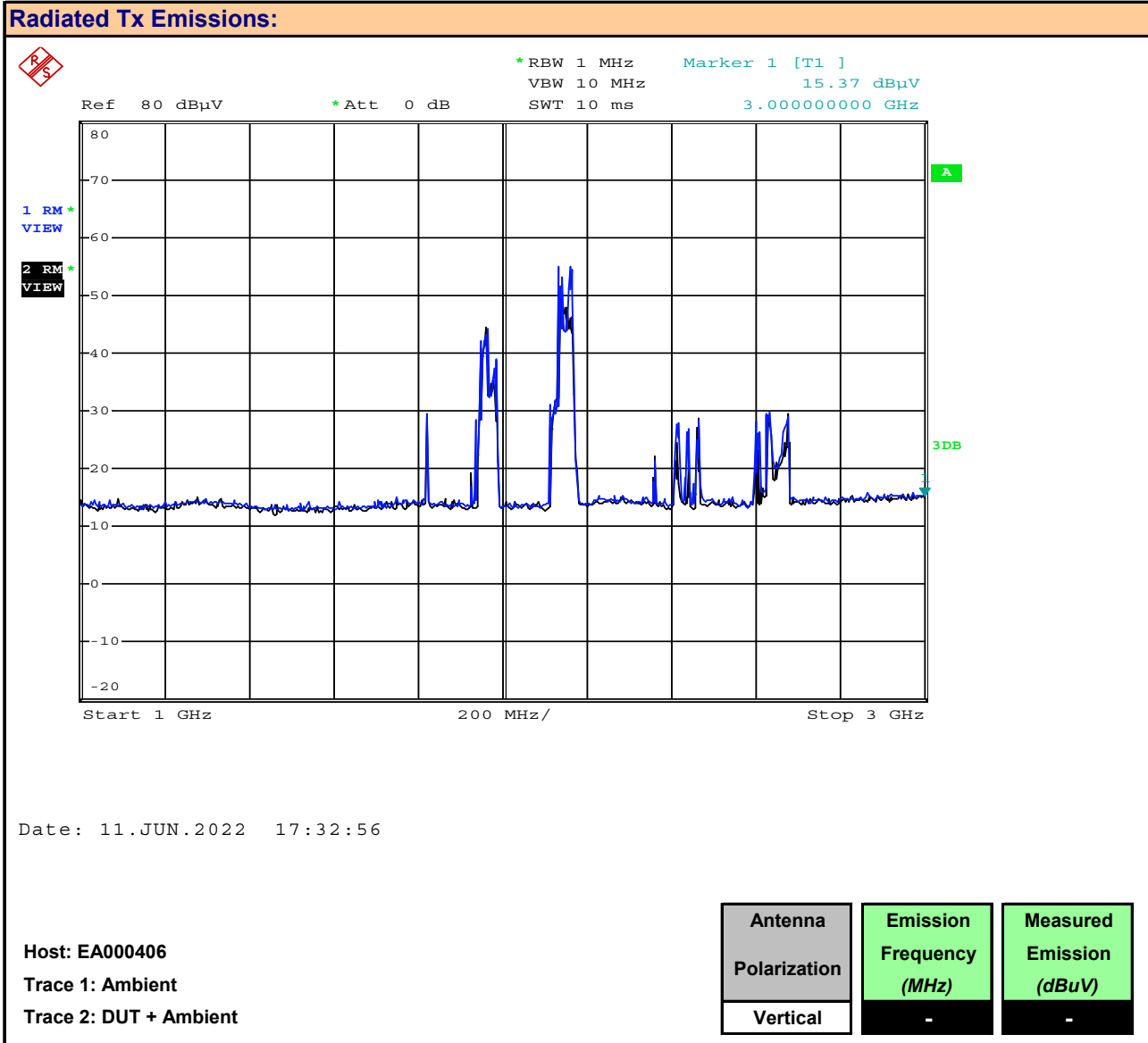
Plot 9.12 – Radiated Tx Emissions, 1 – 3GHz, EA000406, Vertical
