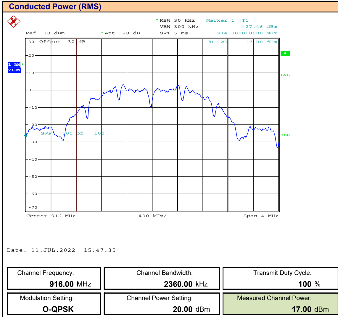
Plot 8.2 – Conducted Power, 916 MHz
