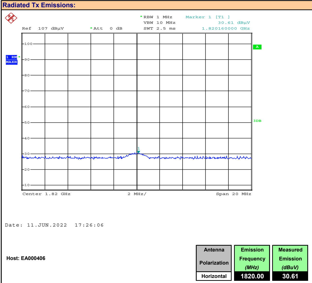
Plot 9.15 – Radiated Tx Emissions, 2 nd Harmonic, EA000406, Horizontal
