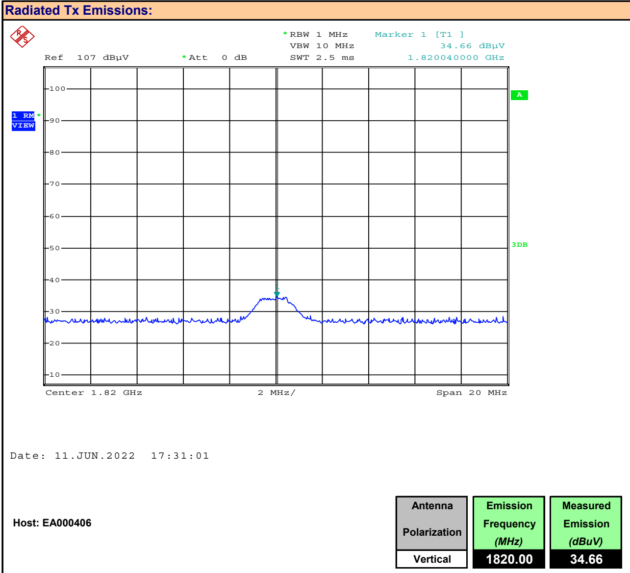
Plot 9.16 – Radiated Tx Emissions, 2 nd Harmonic, EA000406, Vertical
