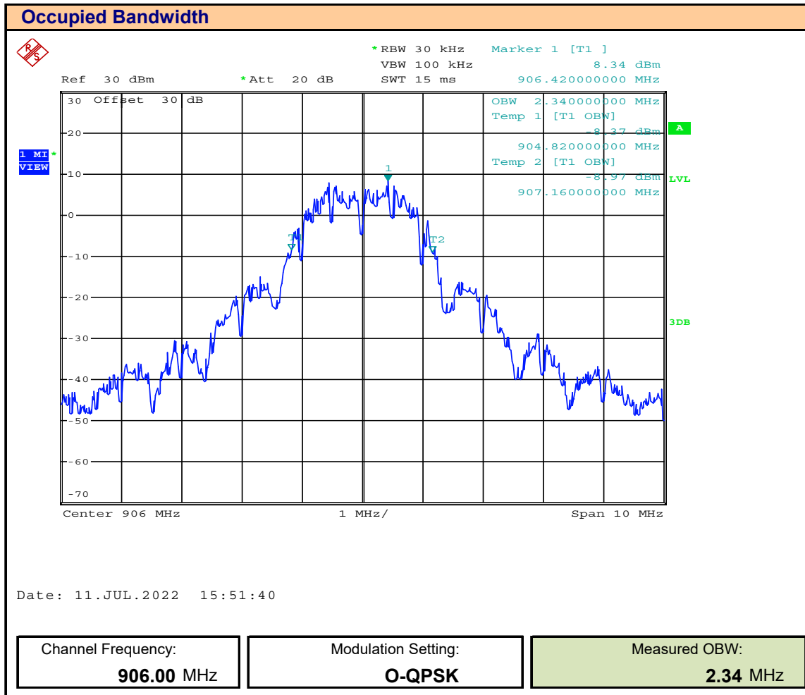
Plot 7.1 – Occupied Bandwidth, 906MHz
