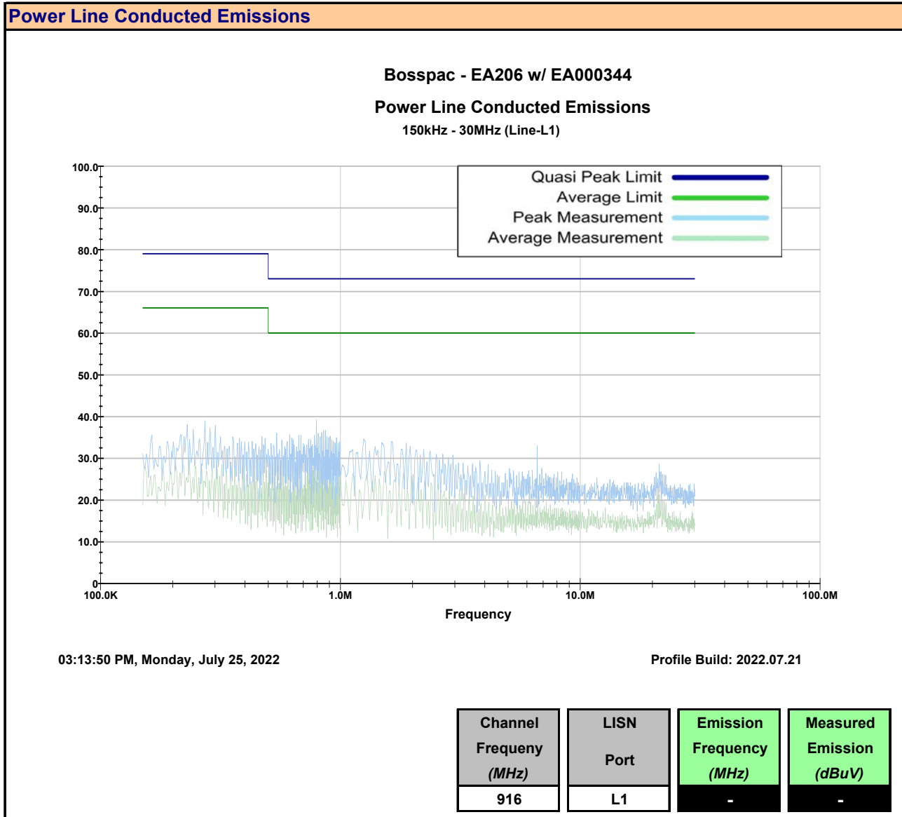
Plot 11.1 – Line Conducted Emissions, EA000344, L1
