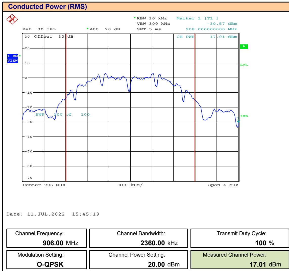
Plot 8.1 – Conducted Power, 906 MHz
