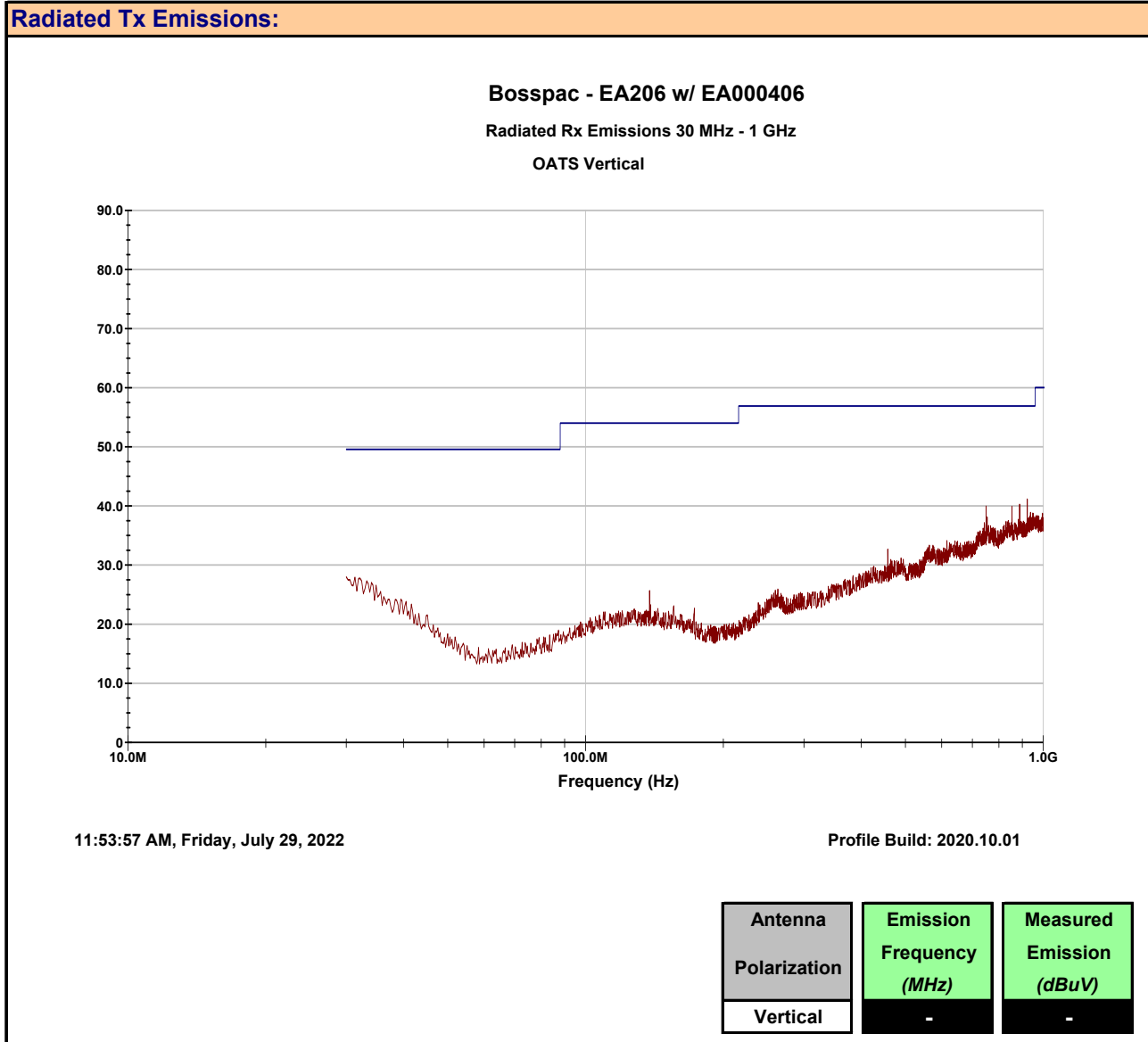
Plot 10.4 – Radiated Rx Emissions, 30 - 1000MHz, EA000406, Vertical
