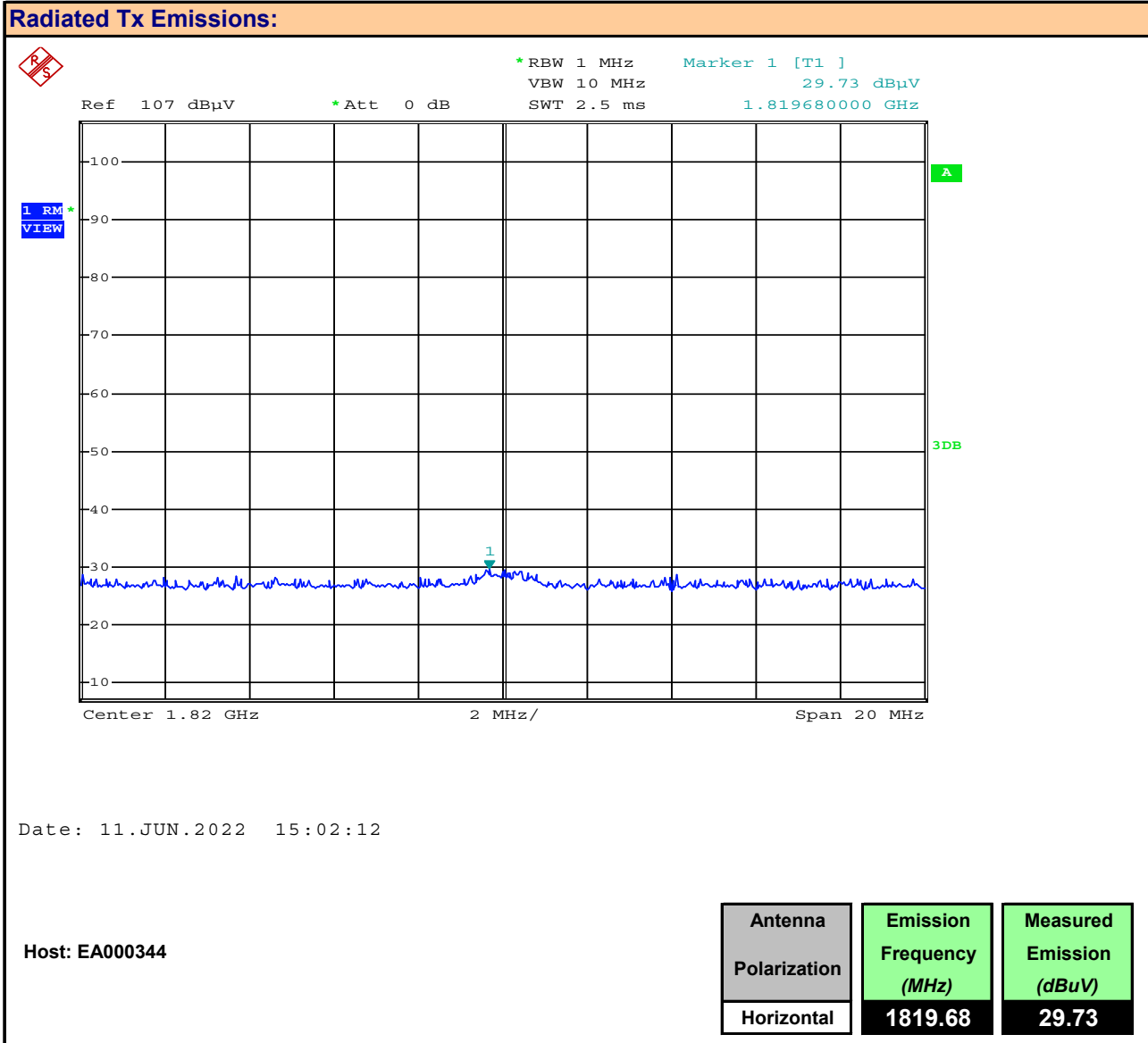
Plot 9.9 – Radiated Tx Emissions, 2 nd Harmonic, EA000344, Horizontal
