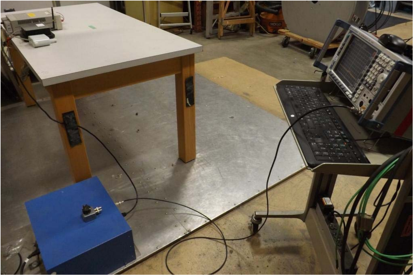
Figure E12.5 – Setup, Line Conducted
