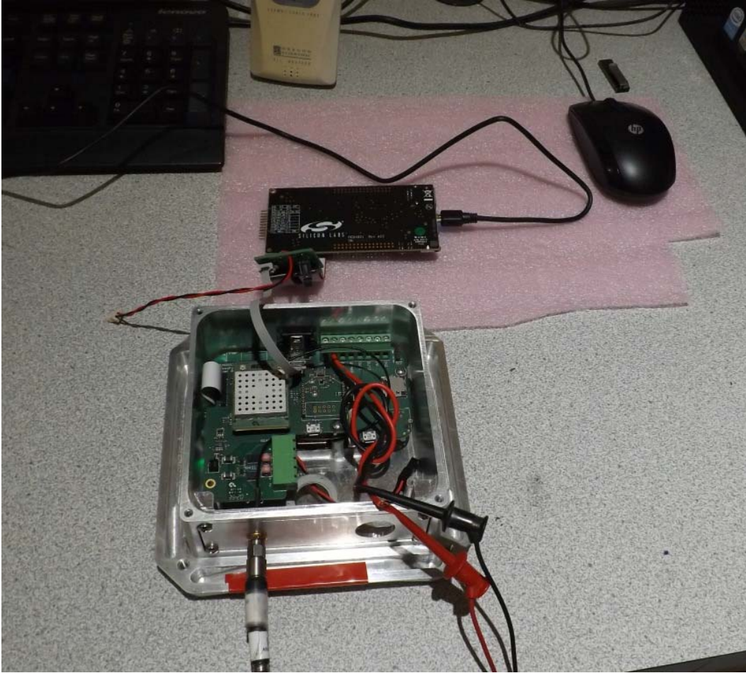
Figure E25.2 – Conducted Measurements w/ Controller
