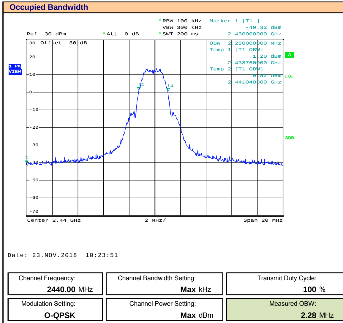
Plot 8.2 – Occupied Bandwidth - 2440MHz - Host 1
