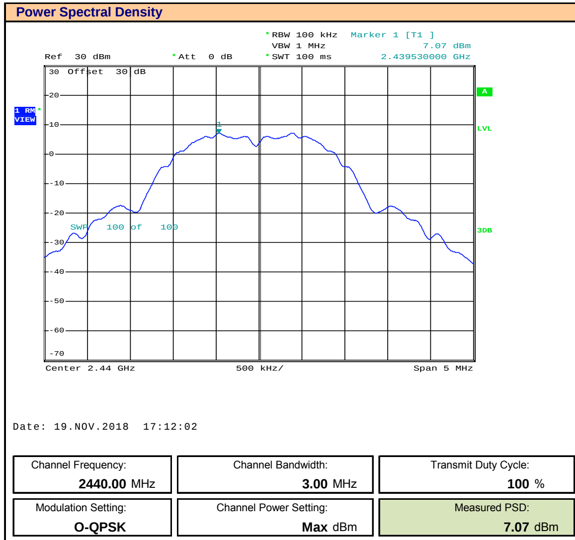
Plot 11.5 – Power Spectral Density – 2440MHz – Host 2
