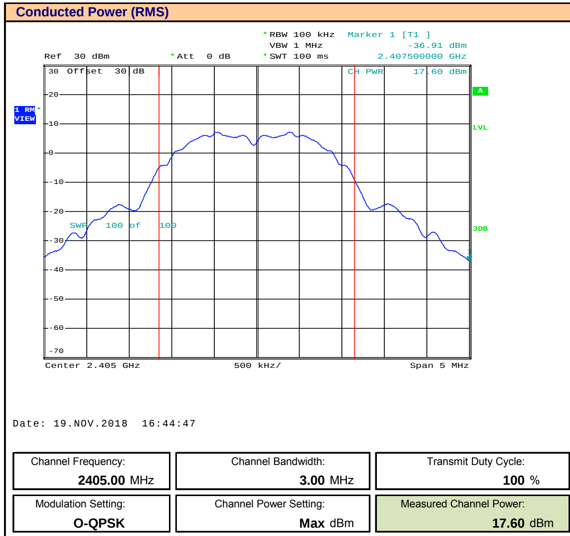
Plot 10.4 – Maximum Conducted Power - 2405MHz - Host 2
