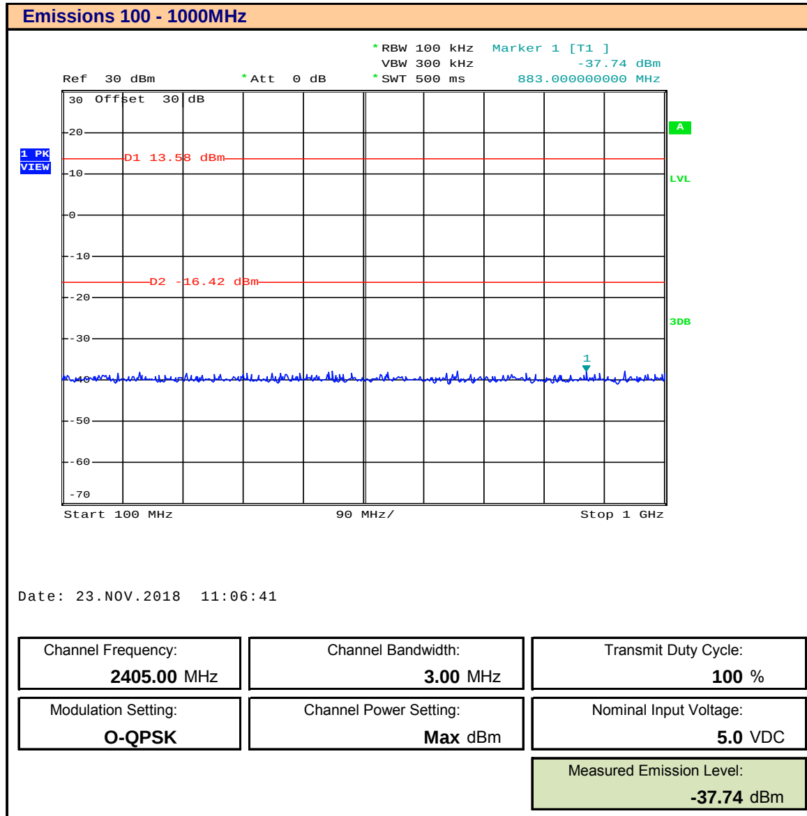
Plot 12.6 – Conducted Spurious Emissions – 100MHz - 1000MHz – Host 1
