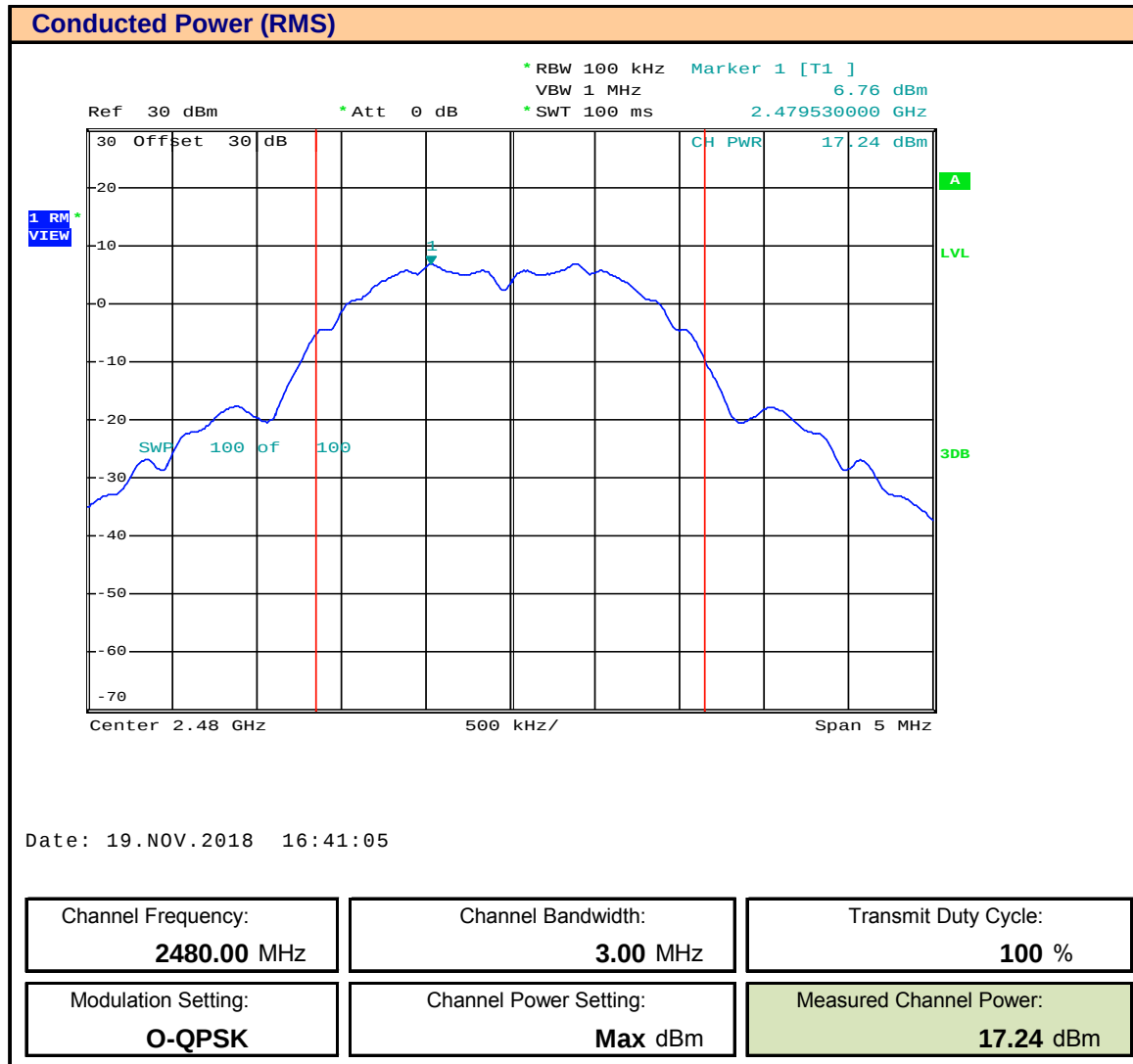
Plot 10.6 – Maximum Conducted Power – 2480MHz - Host 2
