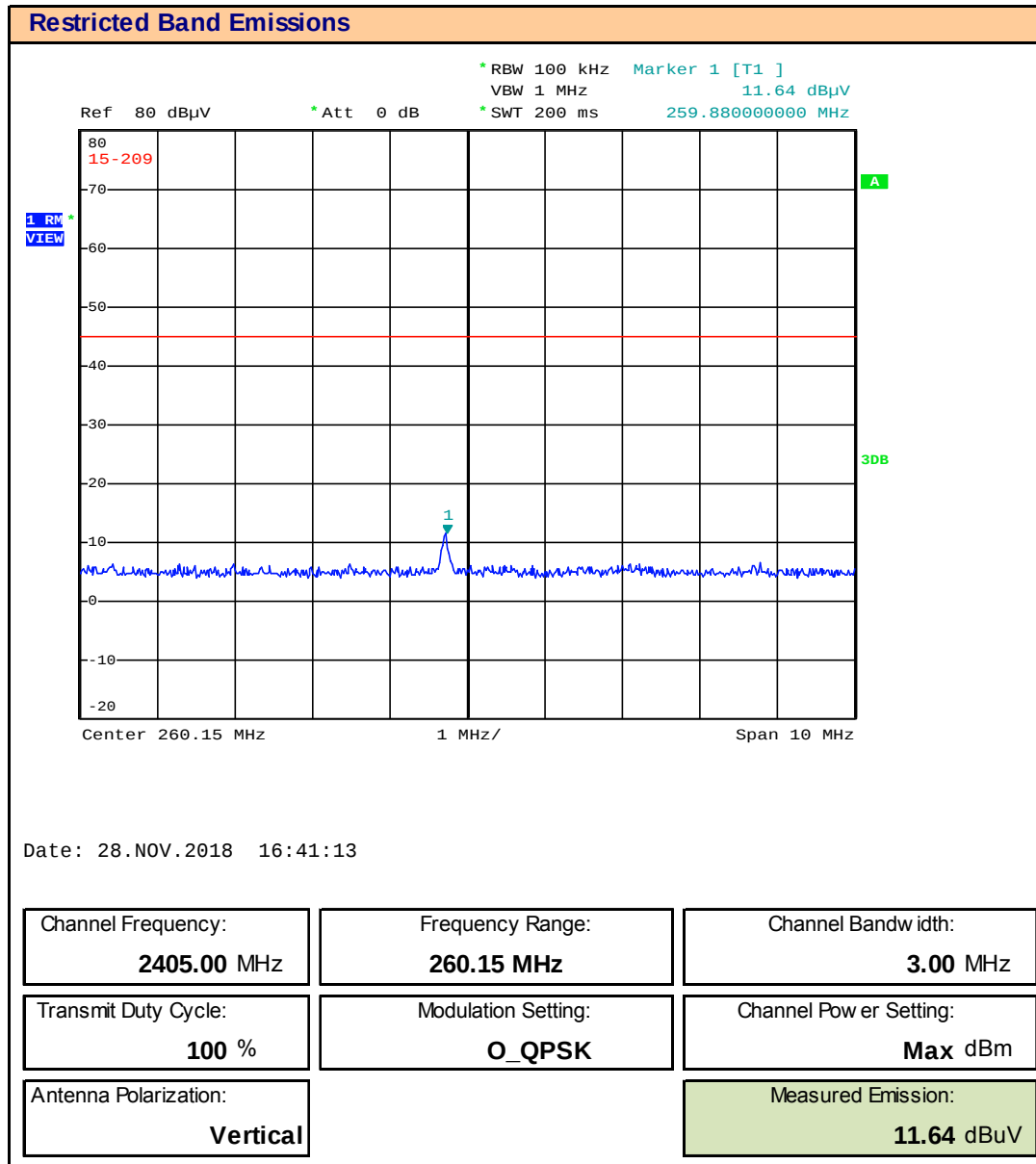
Plot 14.13 – Restricted Band – 260.15MHz – Vertical - Host 1
