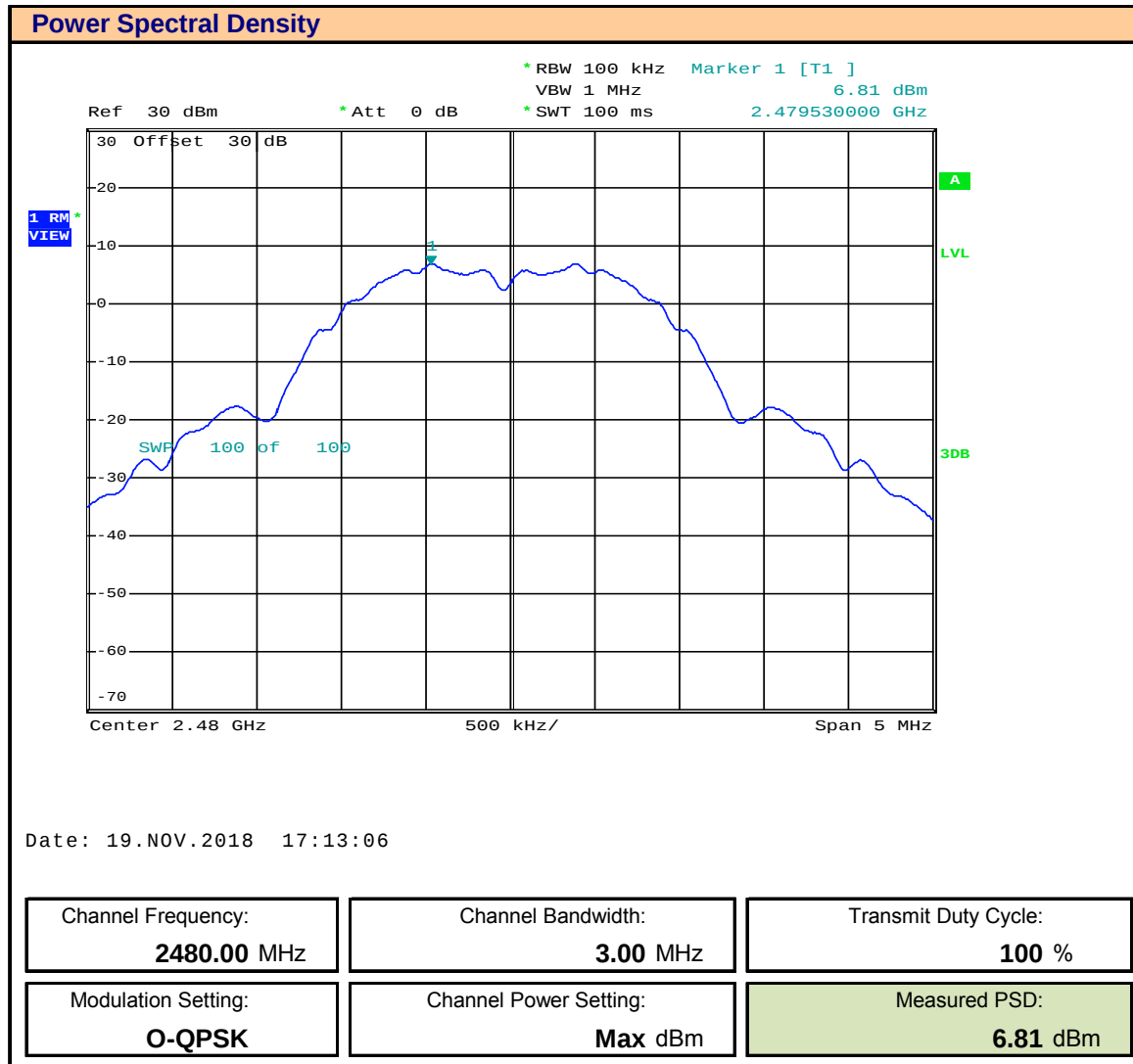
Plot 11.6 – Power Spectral Density - 2480MHz - Host 2
