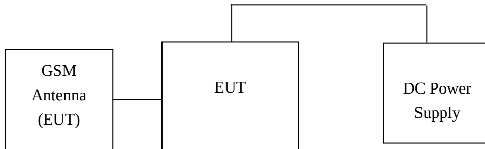
Fig. 2-1 Configuration of Tested System (Fixed Channel)
