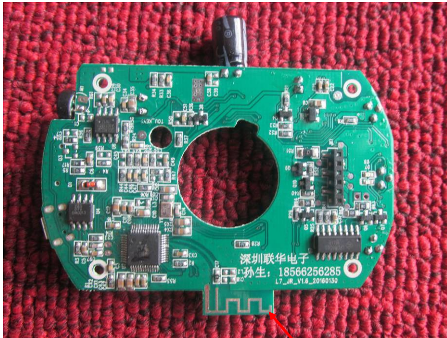
BT Antenna
