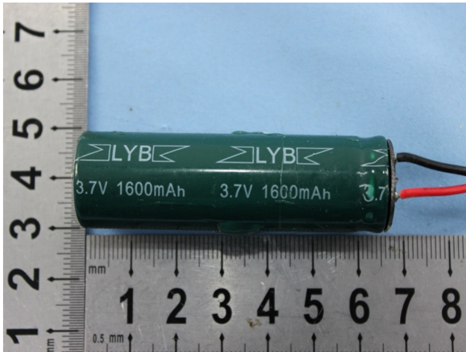
3.7V lithium battery 1600mAh
