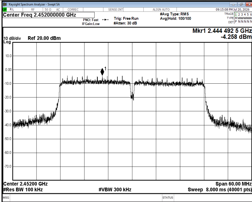
Tx. Spurious NVNT ax40 2452MHz Ant2 Ref
