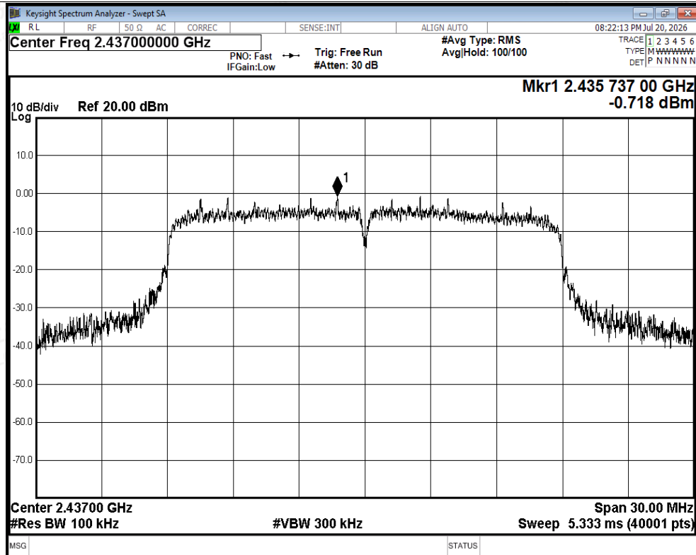
Tx. Spurious NVNT ax20 2437MHz Ant1 Ref
