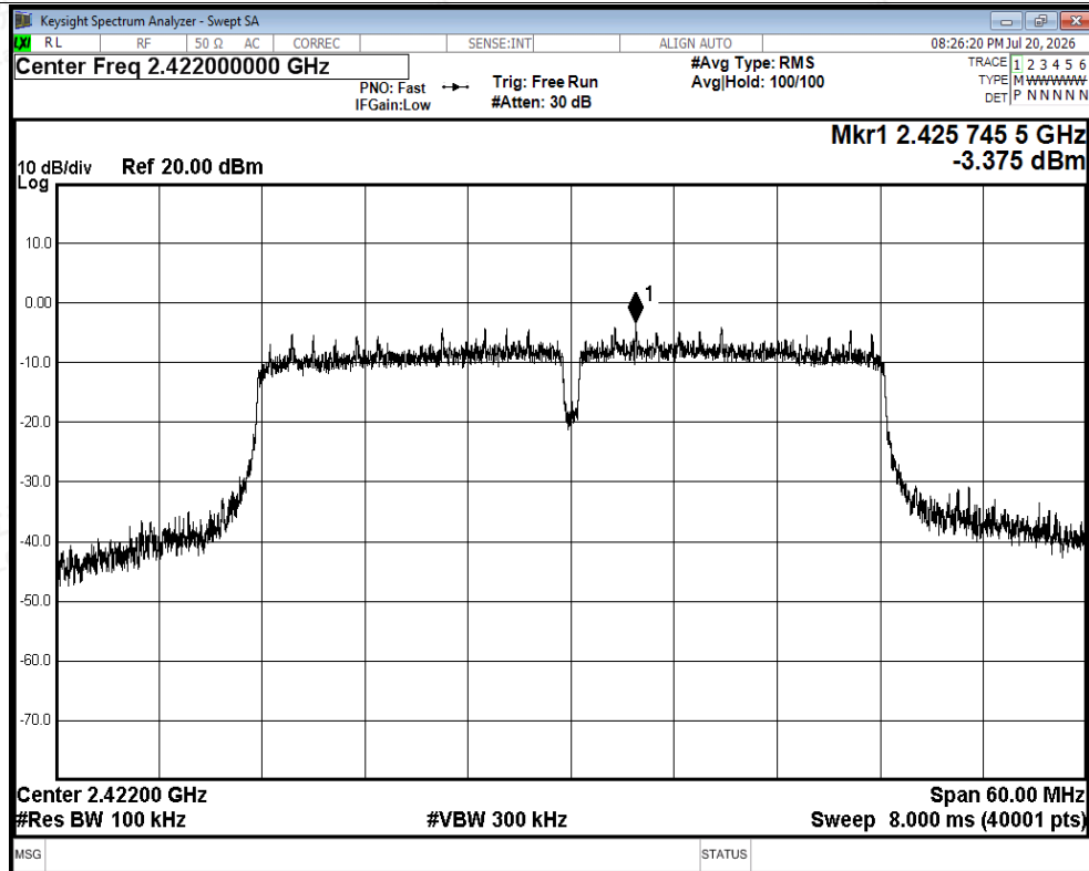
Tx. Spurious NVNT ax40 2422MHz Ant1 Ref
