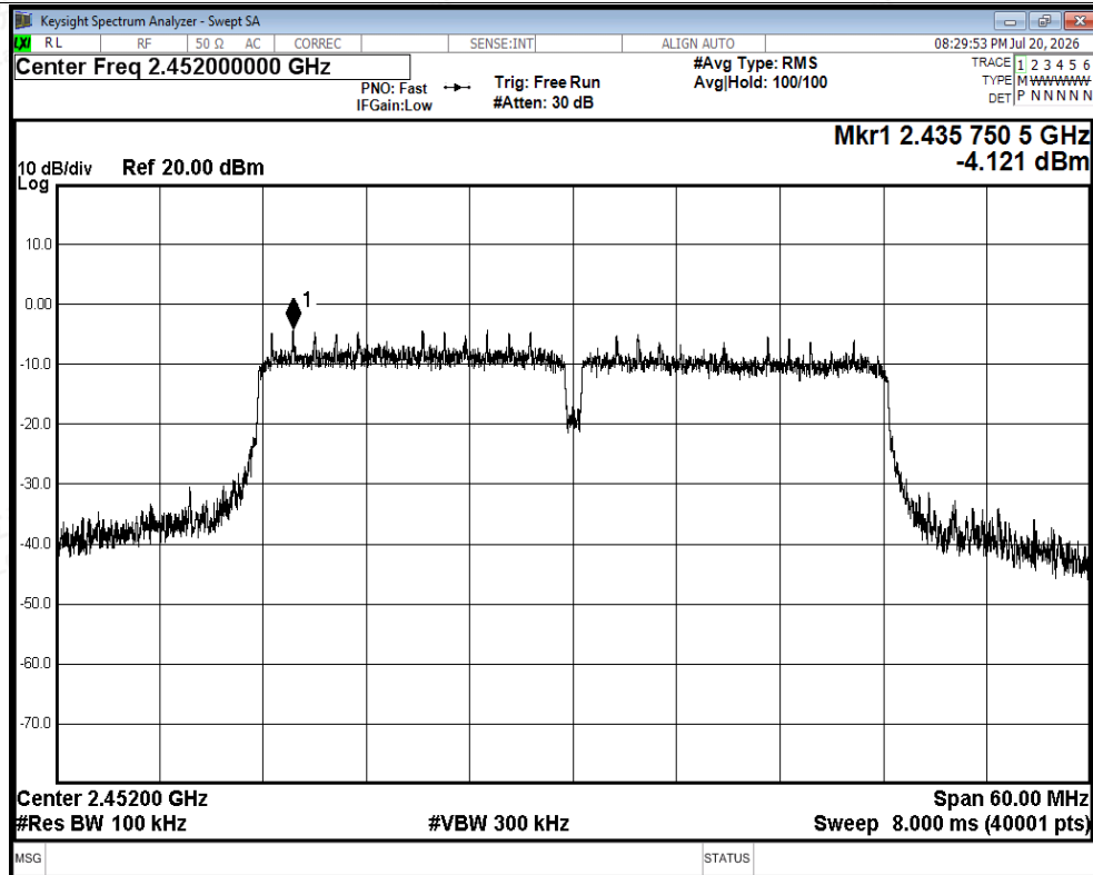
Tx. Spurious NVNT ax40 2452MHz Ant1 Ref
