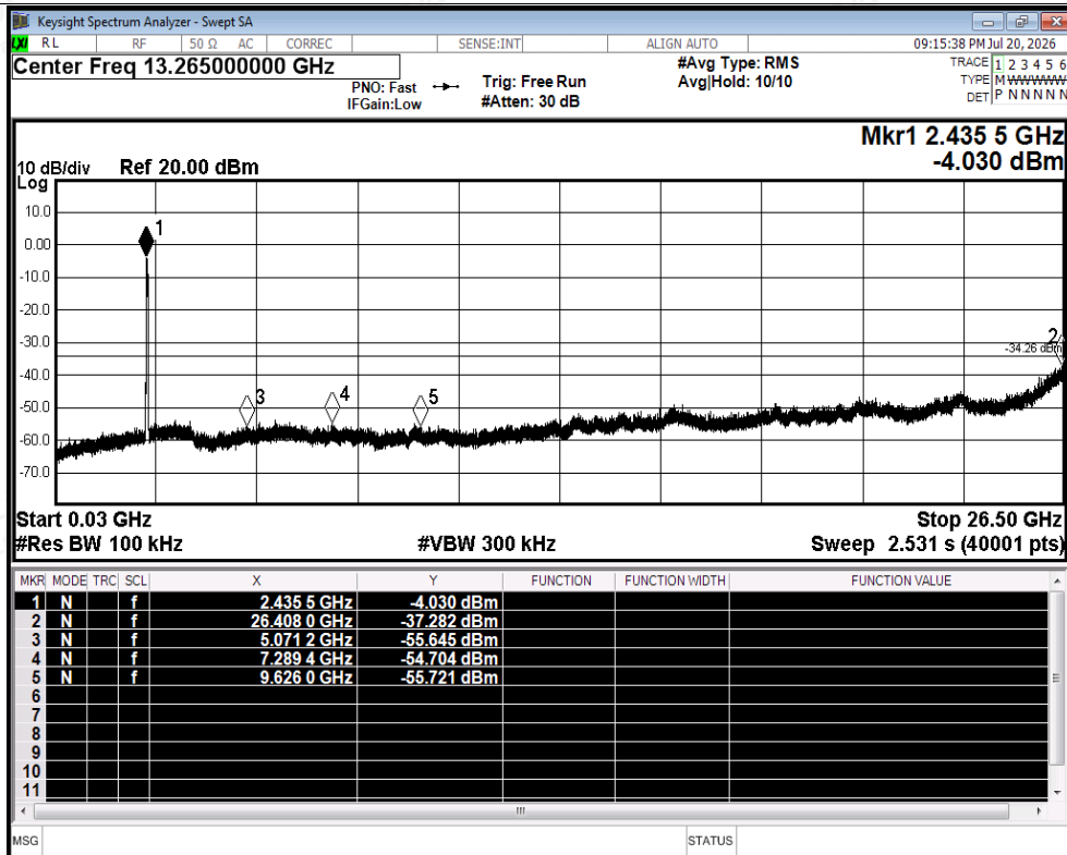
Tx. Spurious NVNT ax40 2452MHz Ant2 Emission
