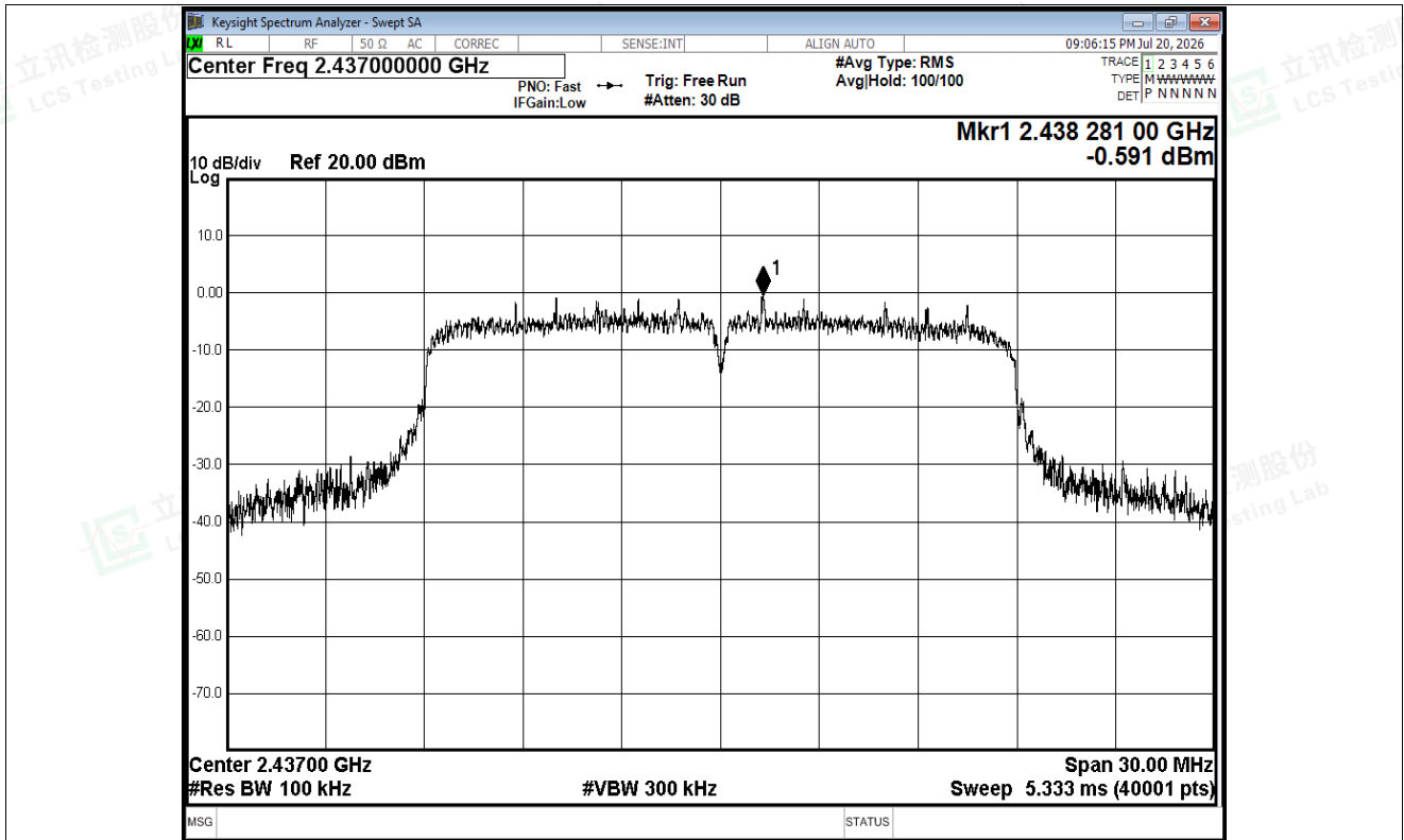
Tx. Spurious NVNT ax20 2437MHz Ant2 Ref
