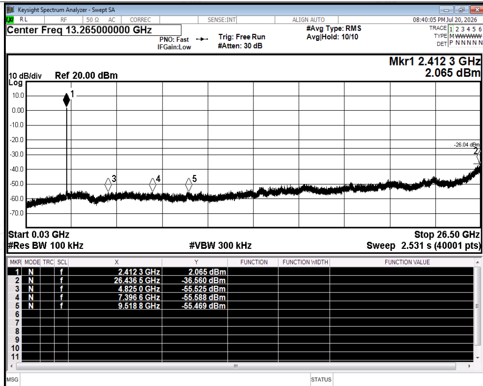
Tx. Spurious NVNT b 2412MHz Ant2 Emission
