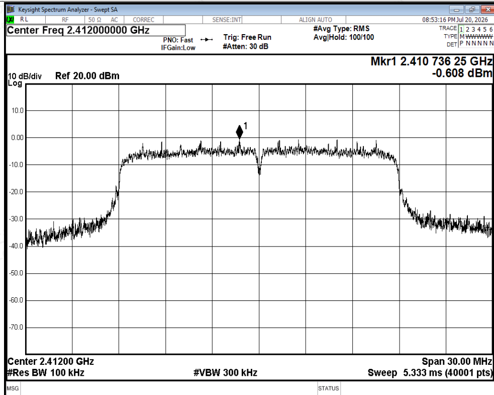
Tx. Spurious NVNT n20 2412MHz Ant2 Ref
