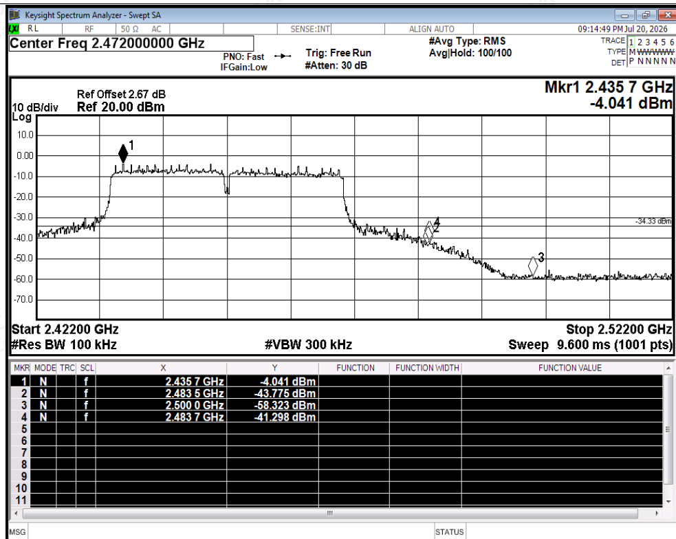
Band Edge NVNT ax40 2452MHz Ant2 Emission
