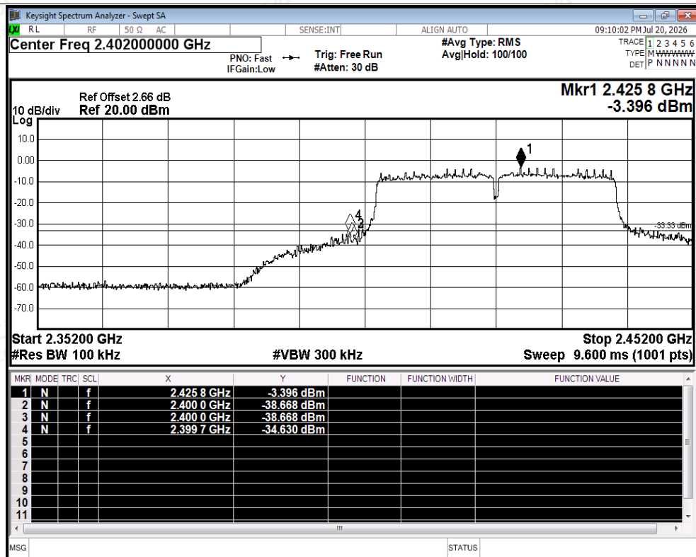
Band Edge NVNT ax40 2422MHz Ant2 Emission
