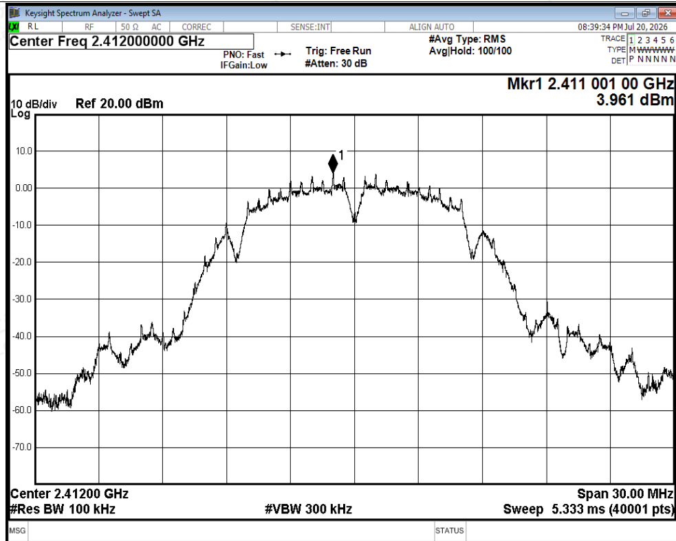
Tx. Spurious NVNT b 2412MHz Ant2 Ref
