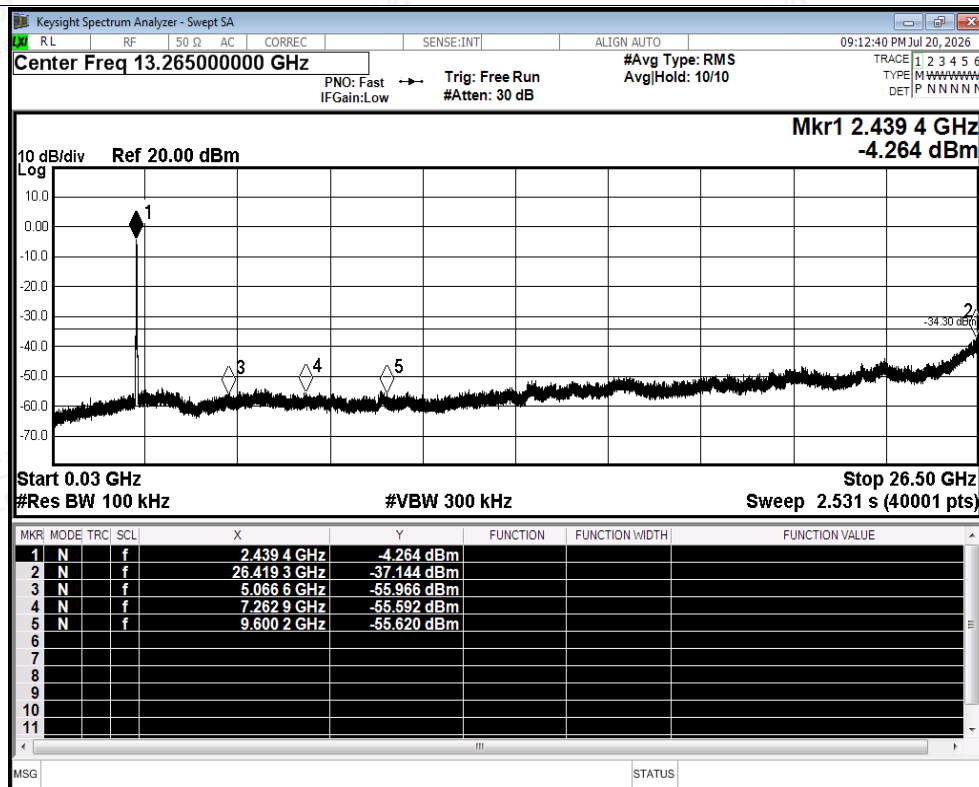
Tx. Spurious NVNT ax40 2437MHz Ant2 Emission
