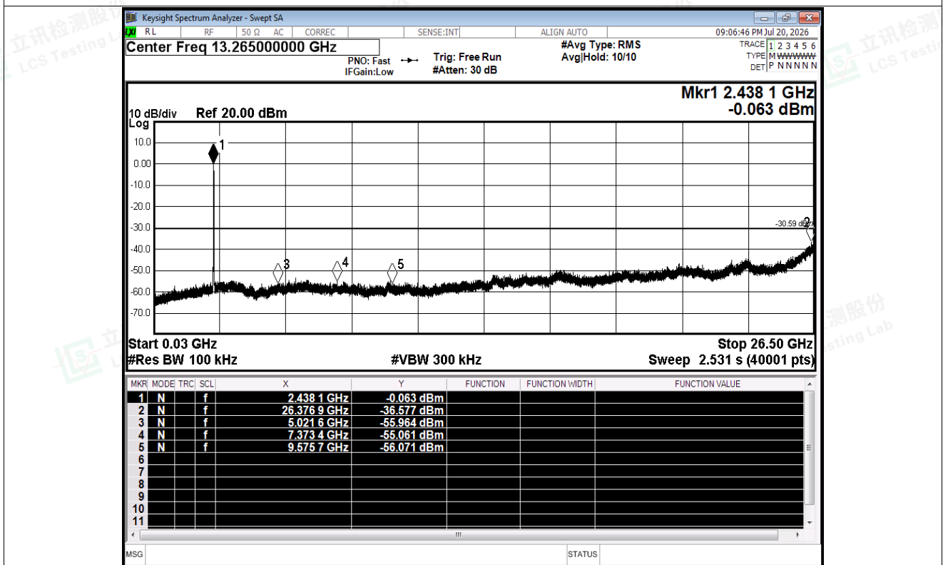
Tx. Spurious NVNT ax20 2437MHz Ant2 Emission
