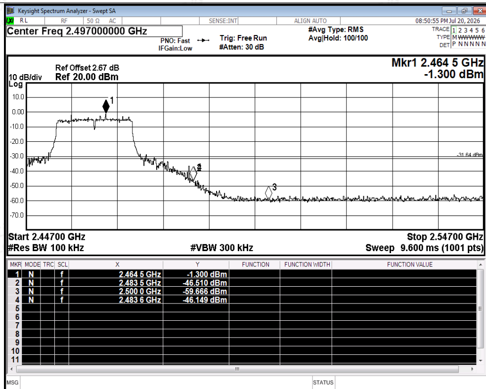
Band Edge NVNT g 2462MHz Ant2 Emission
