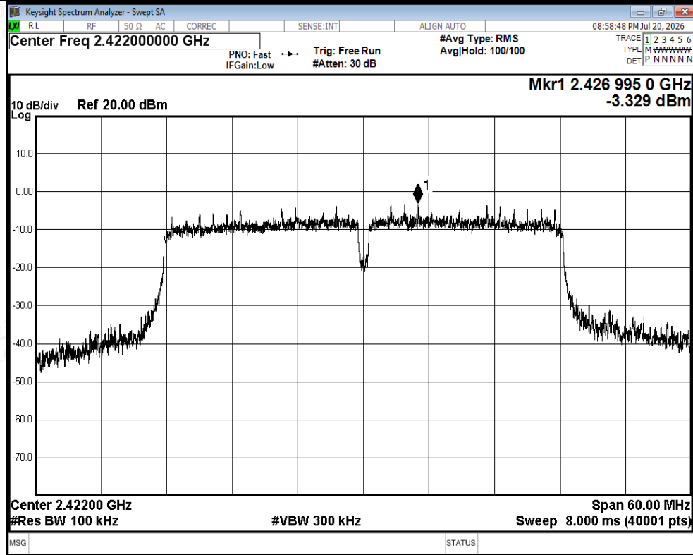
Tx. Spurious NVNT n40 2422MHz Ant2 Ref
