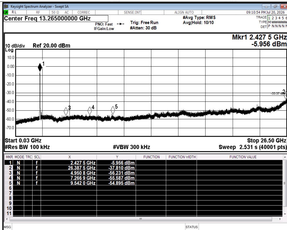
Tx. Spurious NVNT ax40 2422MHz Ant2 Emission
