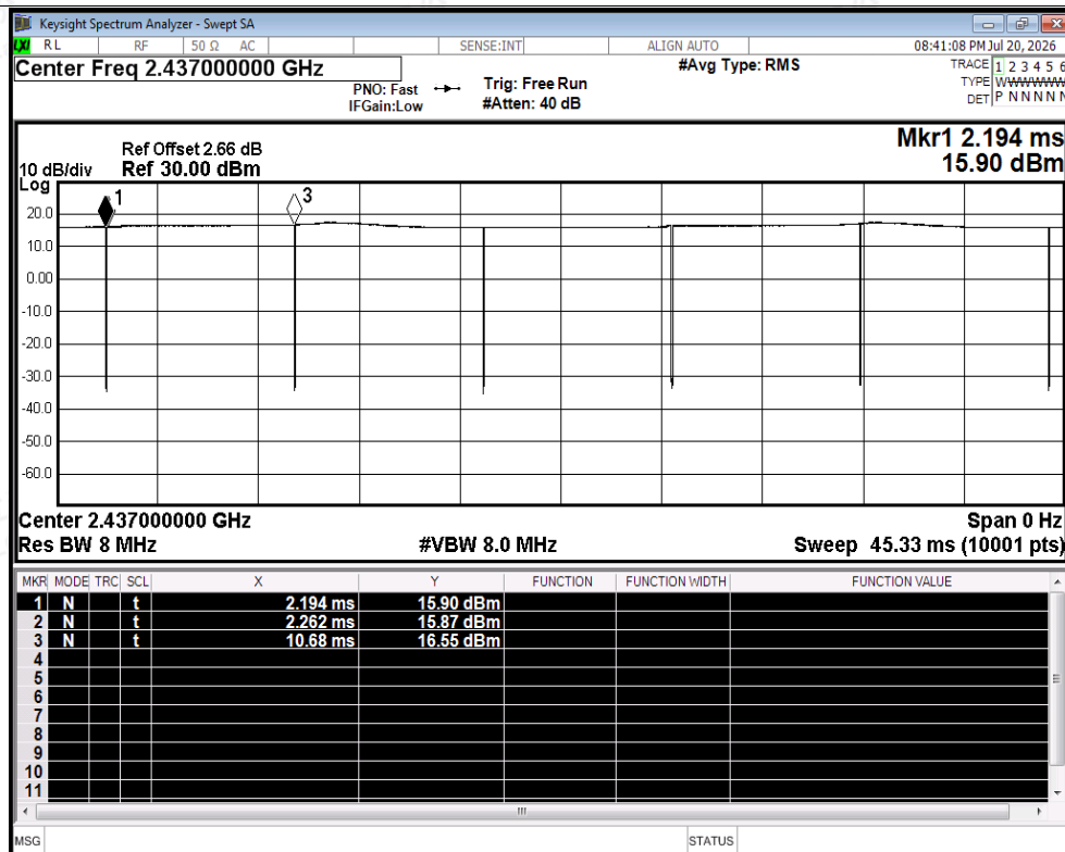
Duty Cycle NVNT b 2437MHz Ant2
