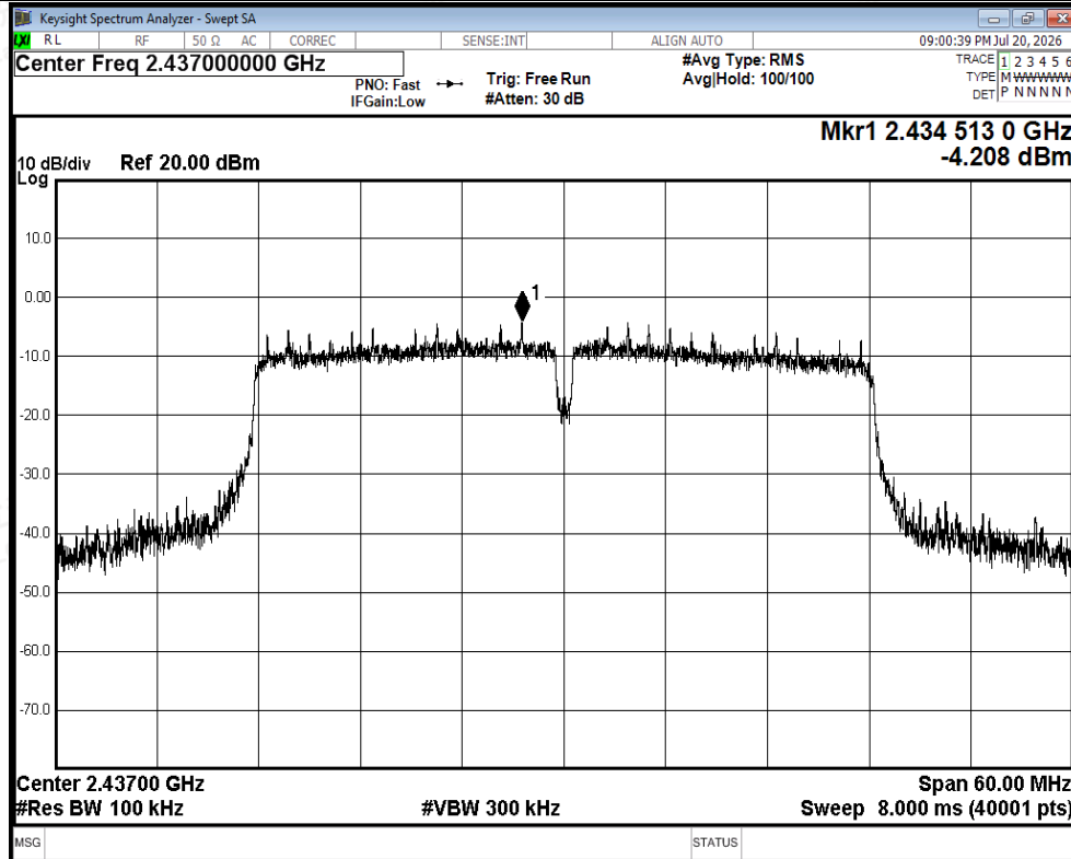
Tx. Spurious NVNT n40 2437MHz Ant2 Ref
