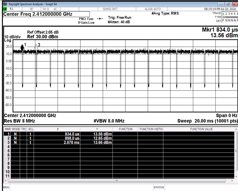
Duty Cycle NVNT ax20 2412MHz Ant1
