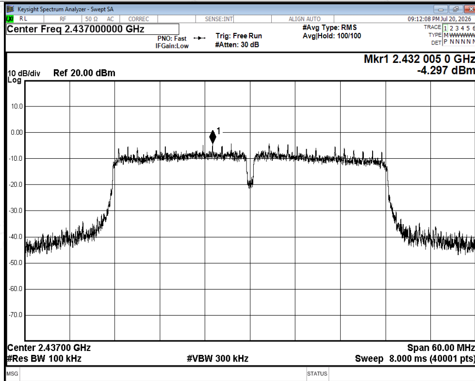
Tx. Spurious NVNT ax40 2437MHz Ant2 Ref
