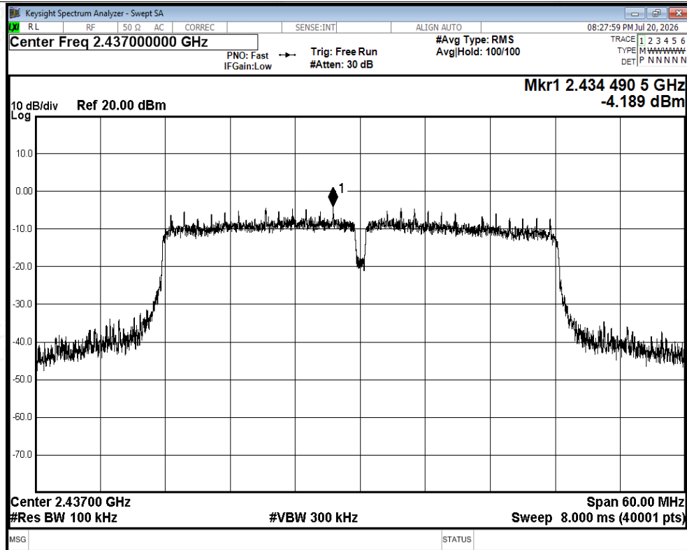
Tx. Spurious NVNT ax40 2437MHz Ant1 Ref
