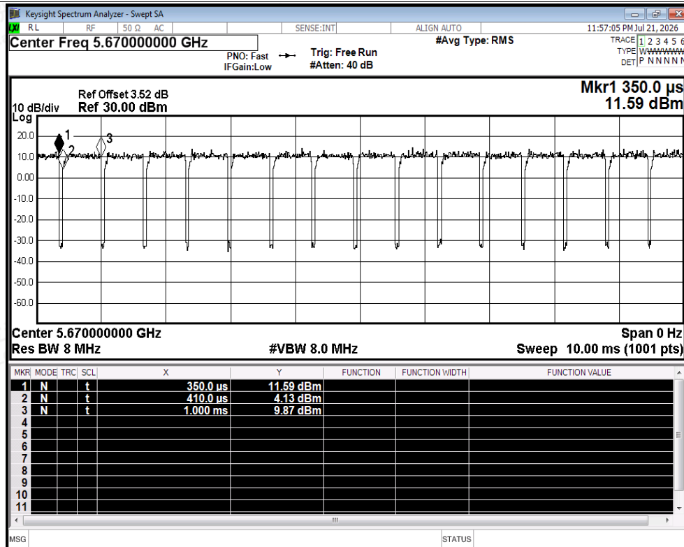
Duty Cycle NVNT n40 5670MHz Ant2
