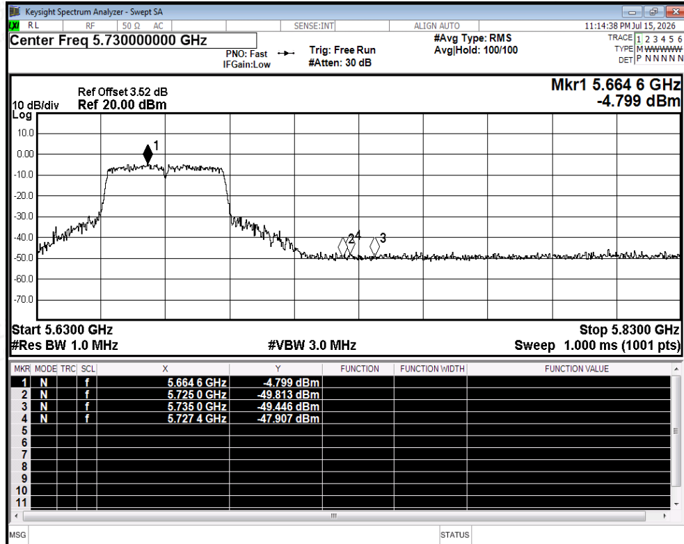
Restrict Band NVNT ax40 5670MHz Ant2 Peak
