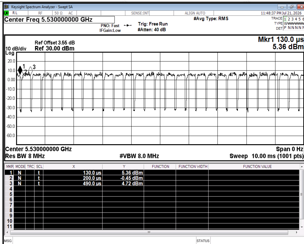
Duty Cycle NVNT ax80 5530MHz Ant2
