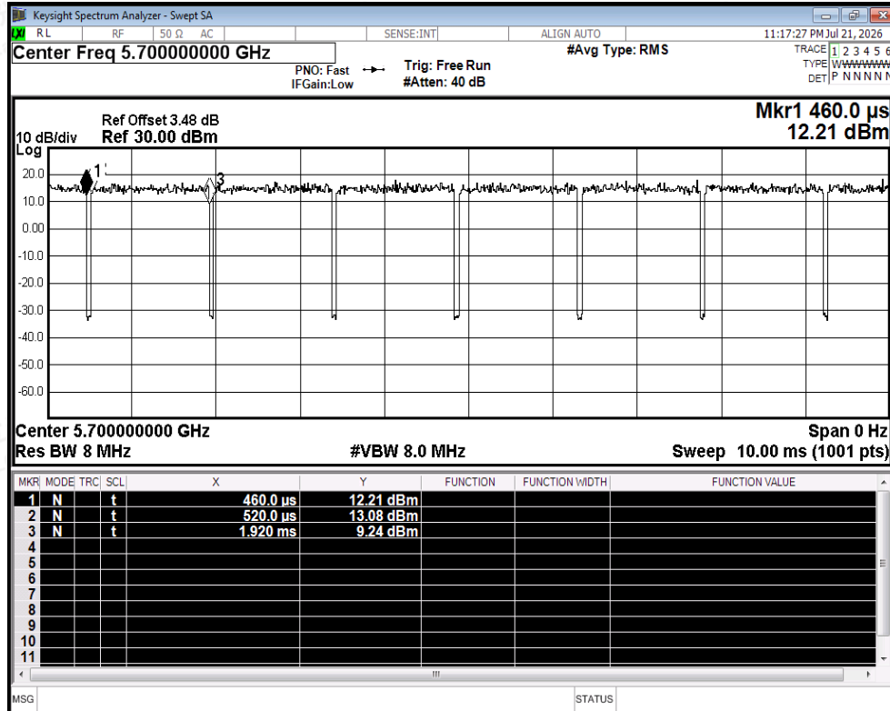
Duty Cycle NVNT a 5700MHz Ant2
