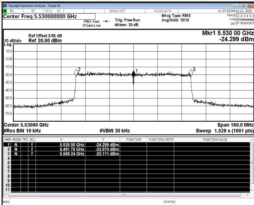
Freq. Stability NVNT ac80 5530MHz Ant2
