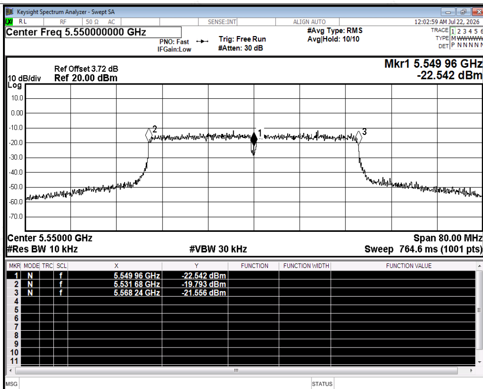
Freq. Stability NVNT ac40 5550MHz Ant2
