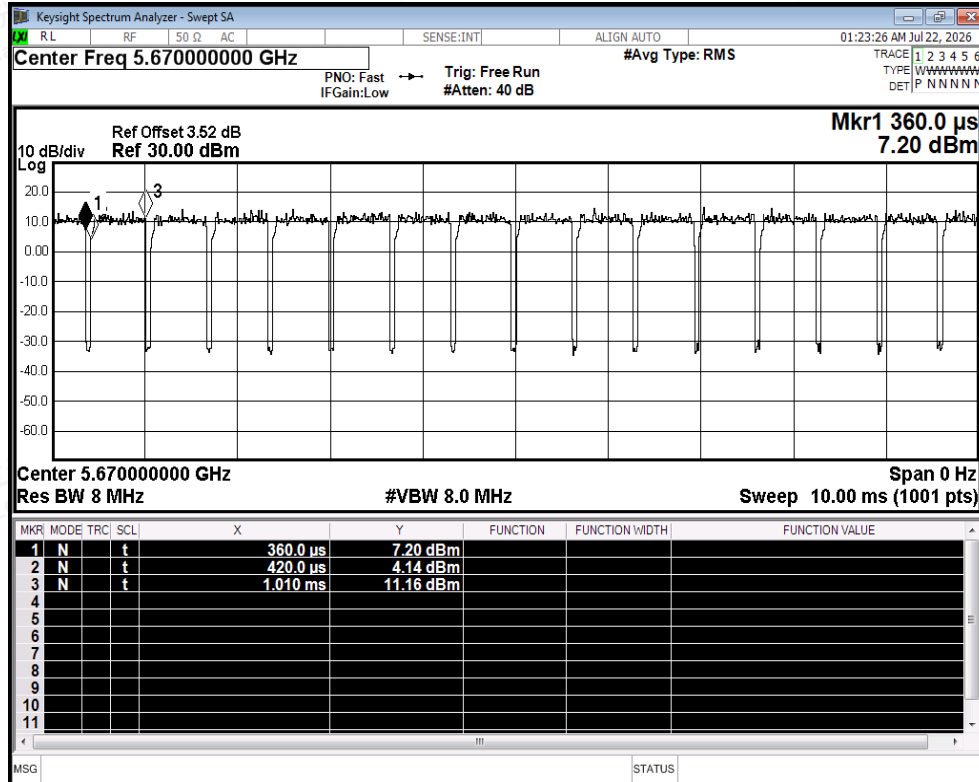
Duty Cycle NVNT ax40 5670MHz Ant2
