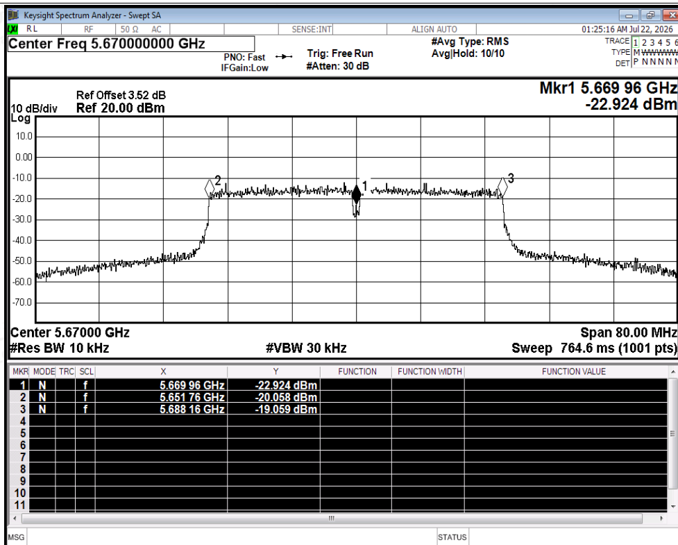
Freq. Stability NVNT ax40 5670MHz Ant2
