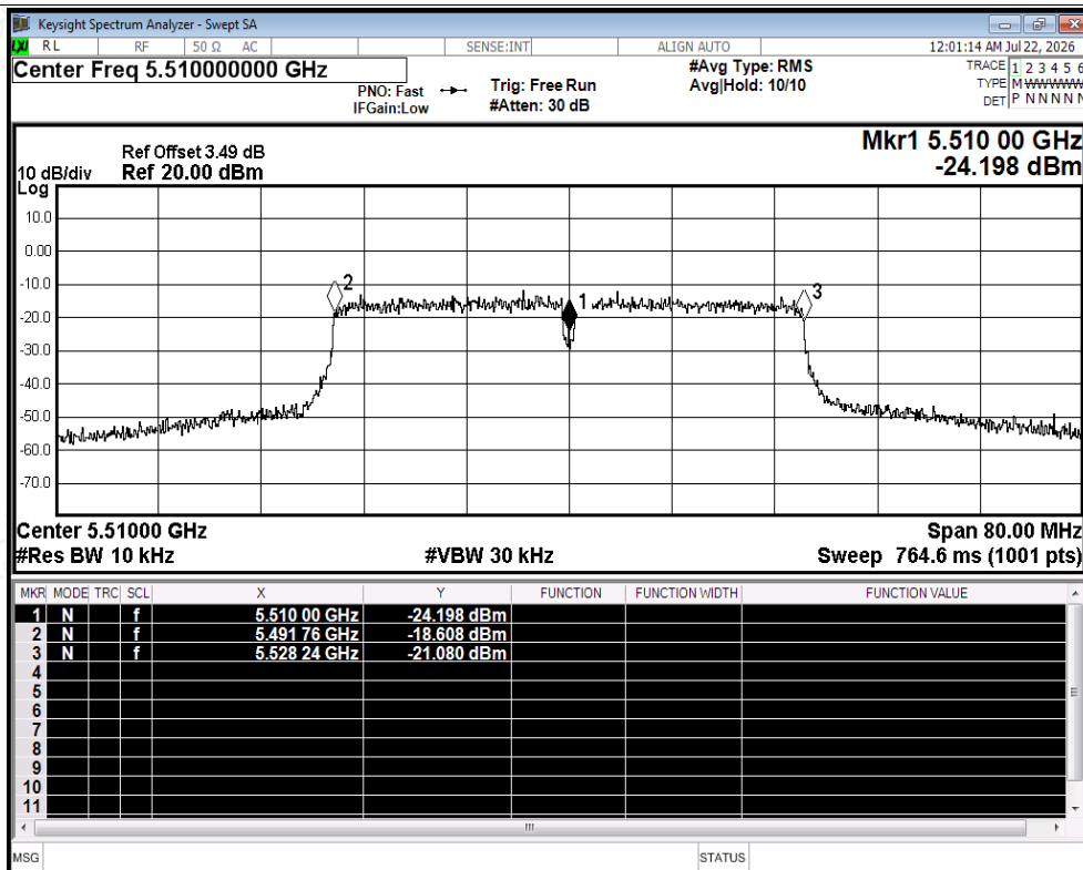
Freq. Stability NVNT ac40 5510MHz Ant2
