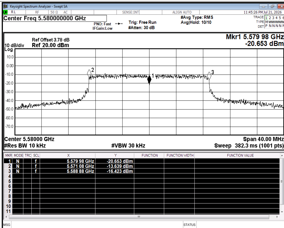
Freq. Stability NVNT ax20 5580MHz Ant2
