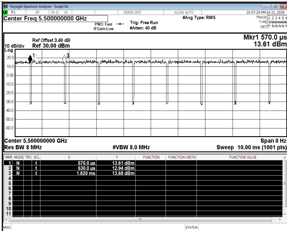
Duty Cycle NVNT ax20 5500MHz Ant1
