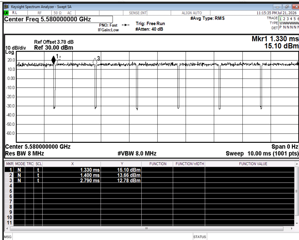
Duty Cycle NVNT a 5580MHz Ant2
