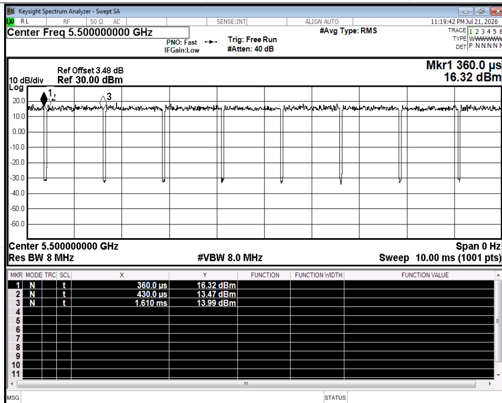
Duty Cycle NVNT n20 5500MHz Ant2
