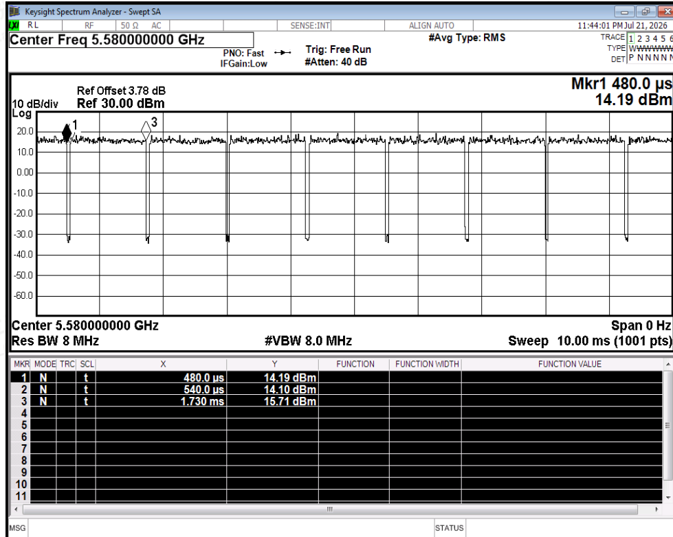
Duty Cycle NVNT ax20 5580MHz Ant2
