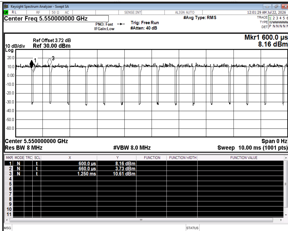
Duty Cycle NVNT ac40 5550MHz Ant2
