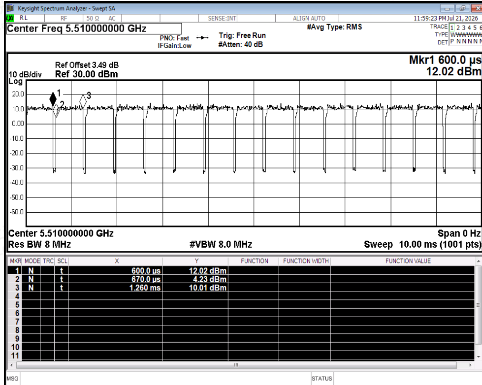
Duty Cycle NVNT ac40 5510MHz Ant2
