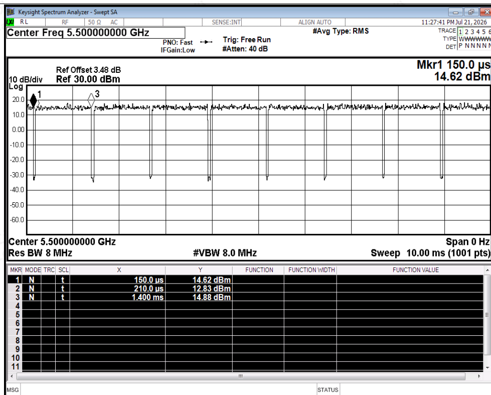
Duty Cycle NVNT ac20 5500MHz Ant2
