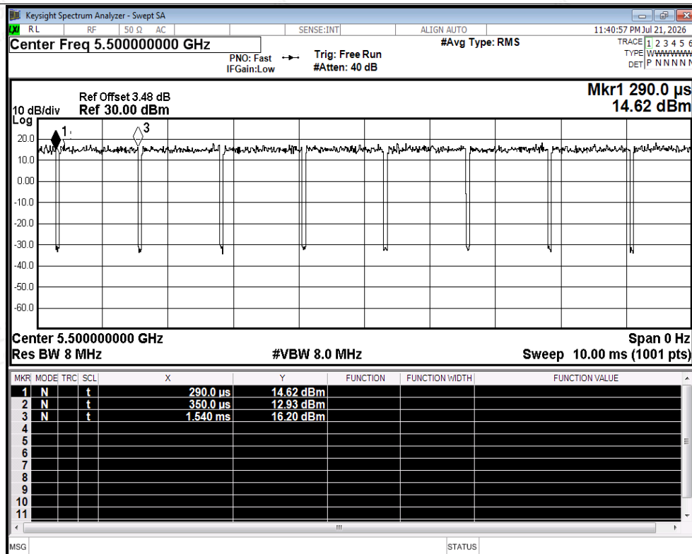
Duty Cycle NVNT ax20 5500MHz Ant2
