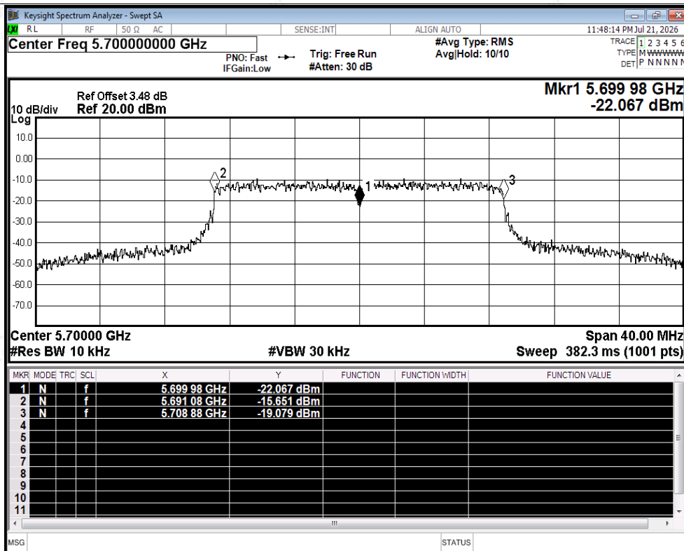
Freq. Stability NVNT ax20 5700MHz Ant2
