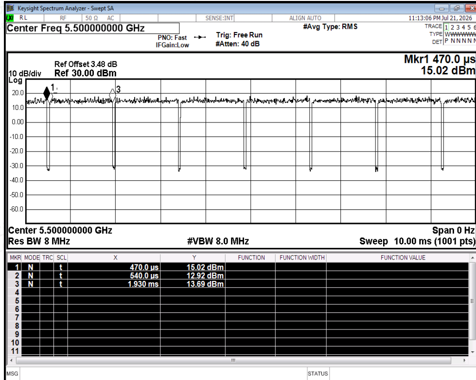
Duty Cycle NVNT a 5500MHz Ant2
