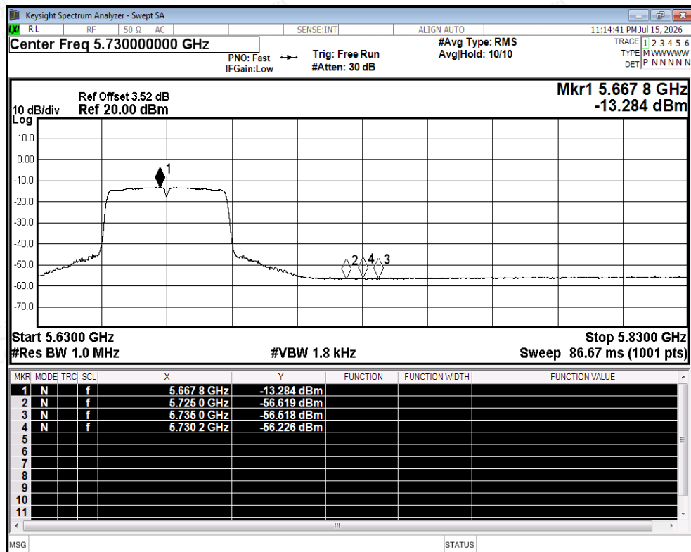
Restrict Band NVNT ax40 5670MHz Ant2 Average
