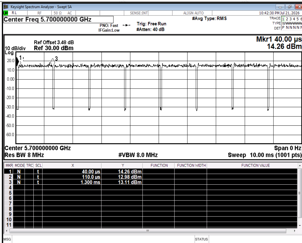
Duty Cycle NVNT ax20 5700MHz Ant1
