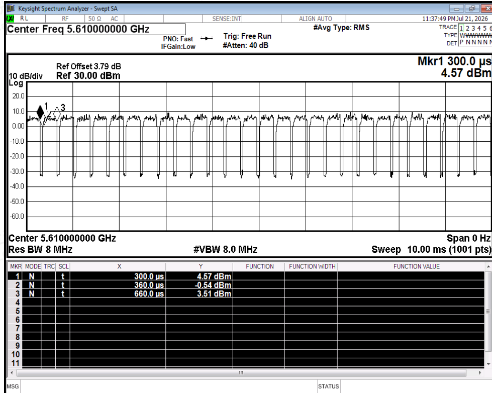
Duty Cycle NVNT ac80 5610MHz Ant2
