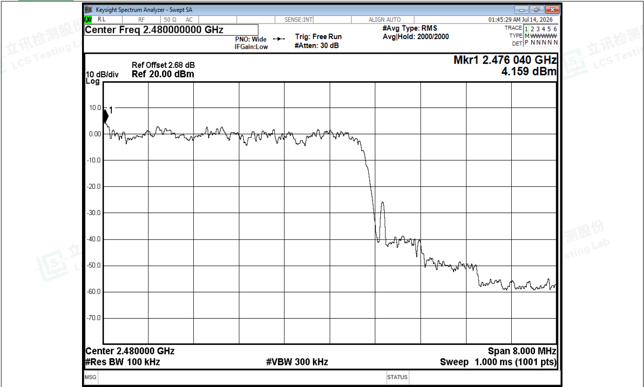
Band Edge (Hopping) NVNT 2-DH5 2480MHz Ant1 Hopping Ref
