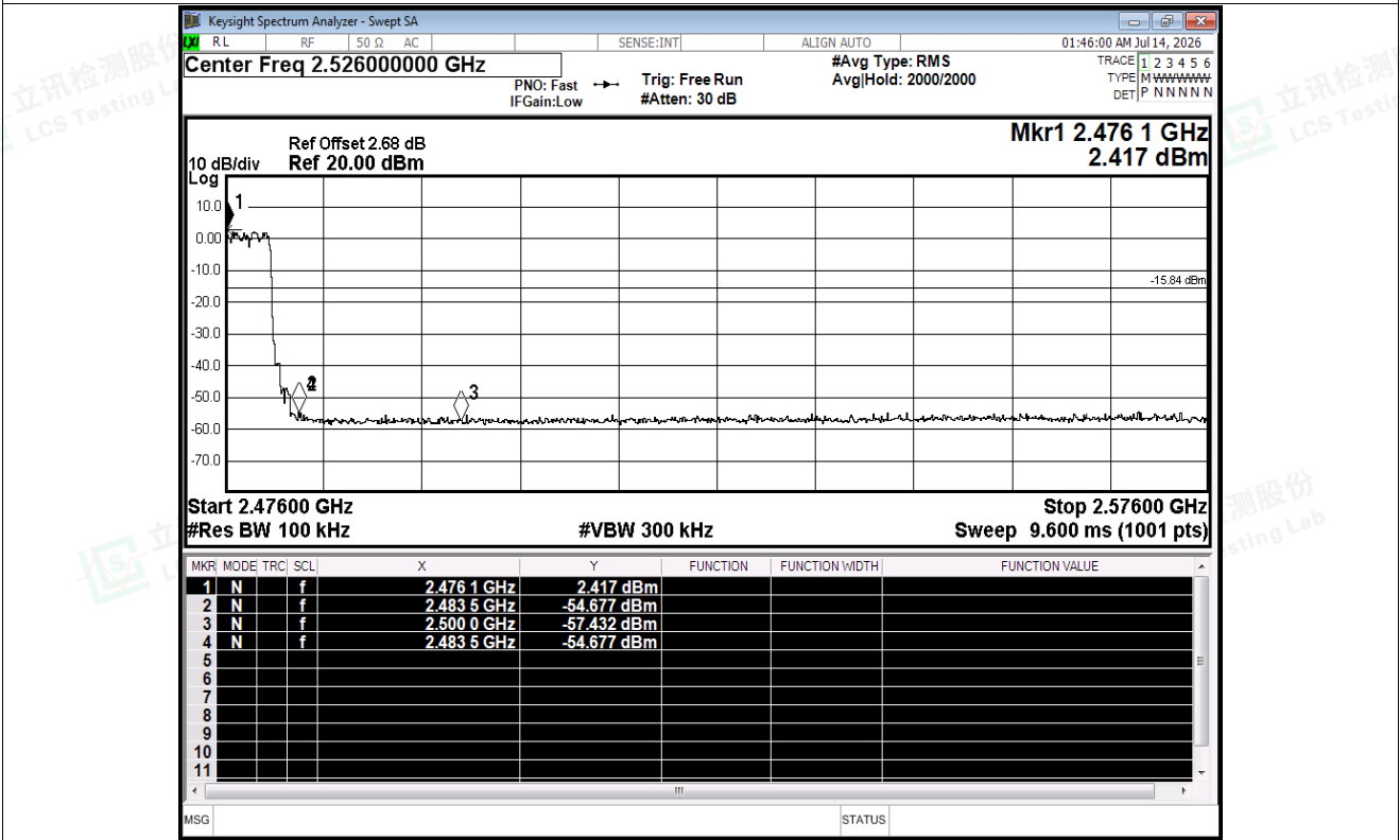
Band Edge (Hopping) NVNT 2-DH5 2480MHz Ant1 Hopping Emission
