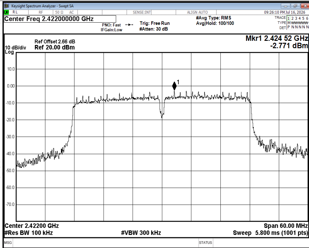
Band Edge NVNT ax40 2422MHz Ant2 Ref
