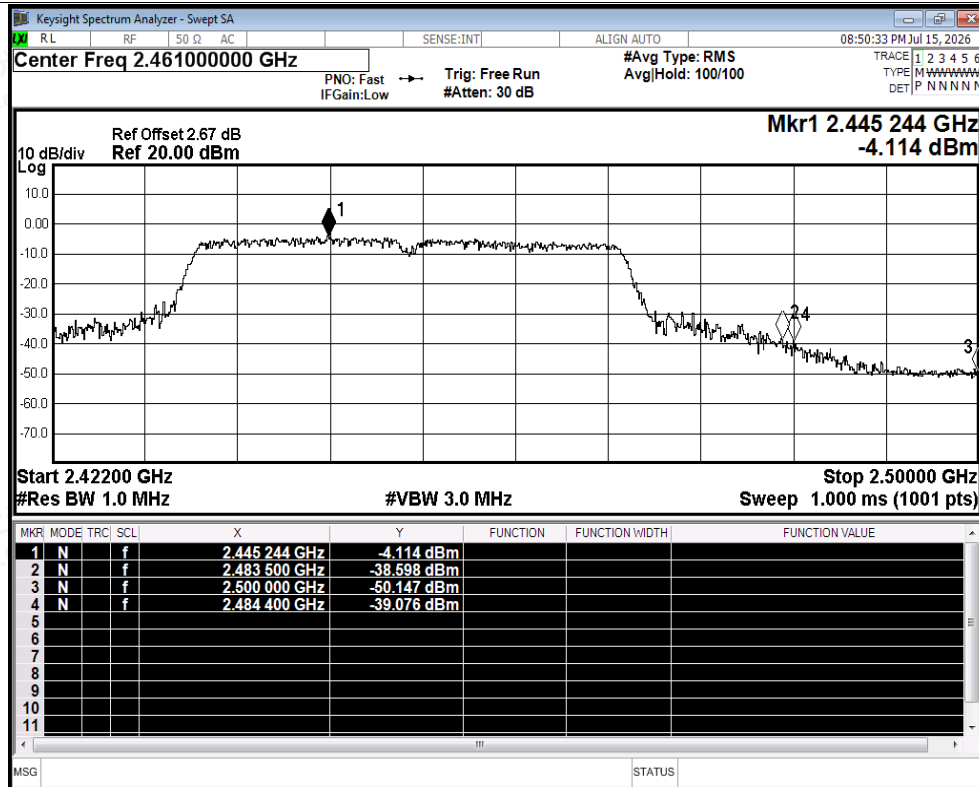
Restrict Band NVNT ax40 2452MHz Ant2 Peak
