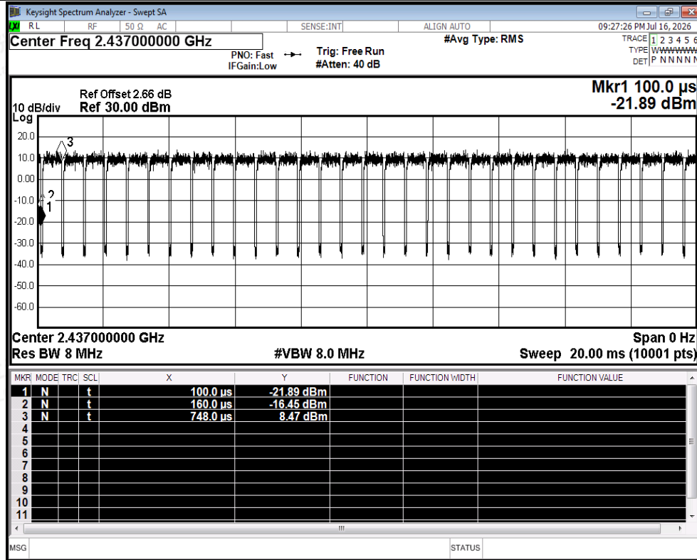
Duty Cycle NVNT ax40 2437MHz Ant2
