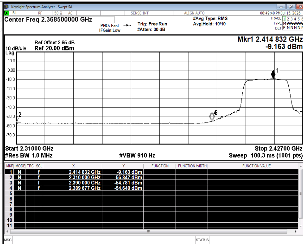
Restrict Band NVNT ax20 2412MHz Ant2 Average
