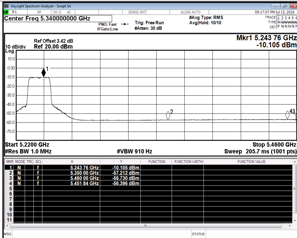
Restrict Band NVNT ax20 5240MHz Ant2 Average
