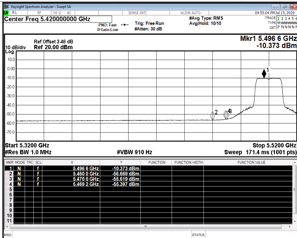
Restrict Band NVNT ax20 5500MHz Ant2 Average
