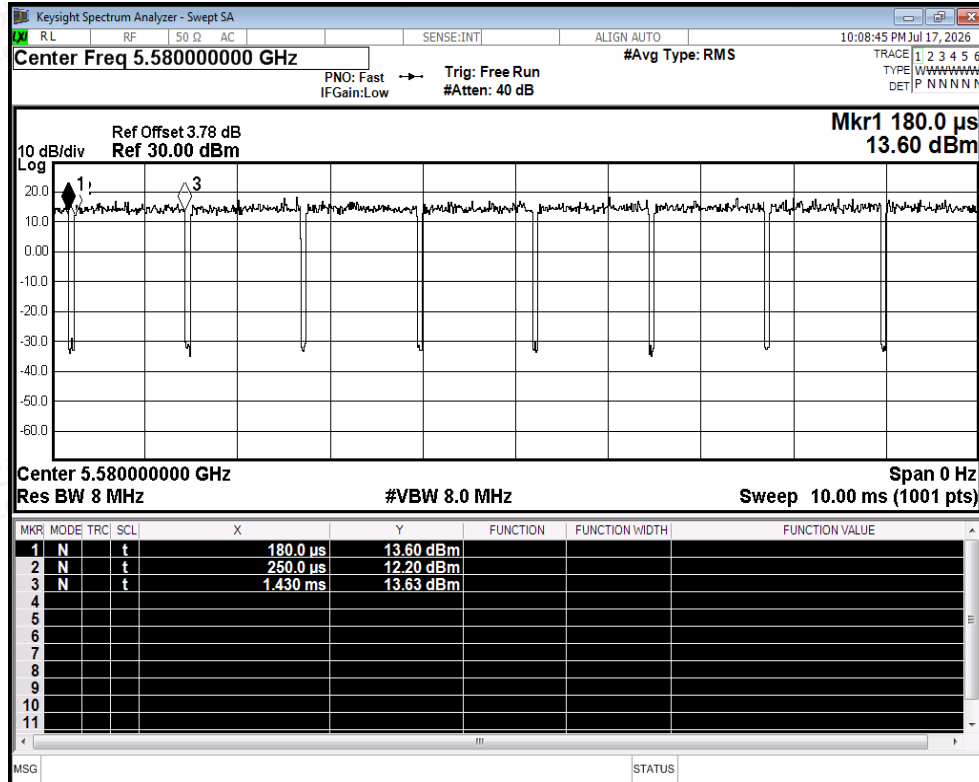
Duty Cycle NVNT ac20 5580MHz Ant1
