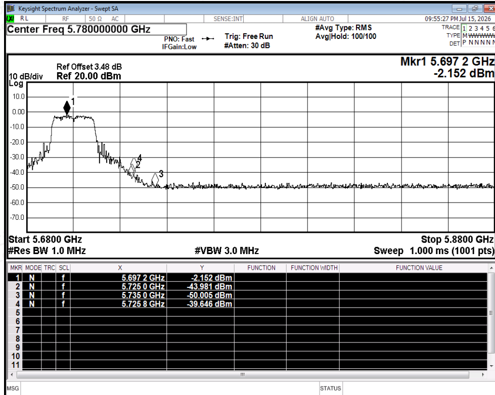
Restrict Band NVNT ax20 5700MHz Ant2 Peak
