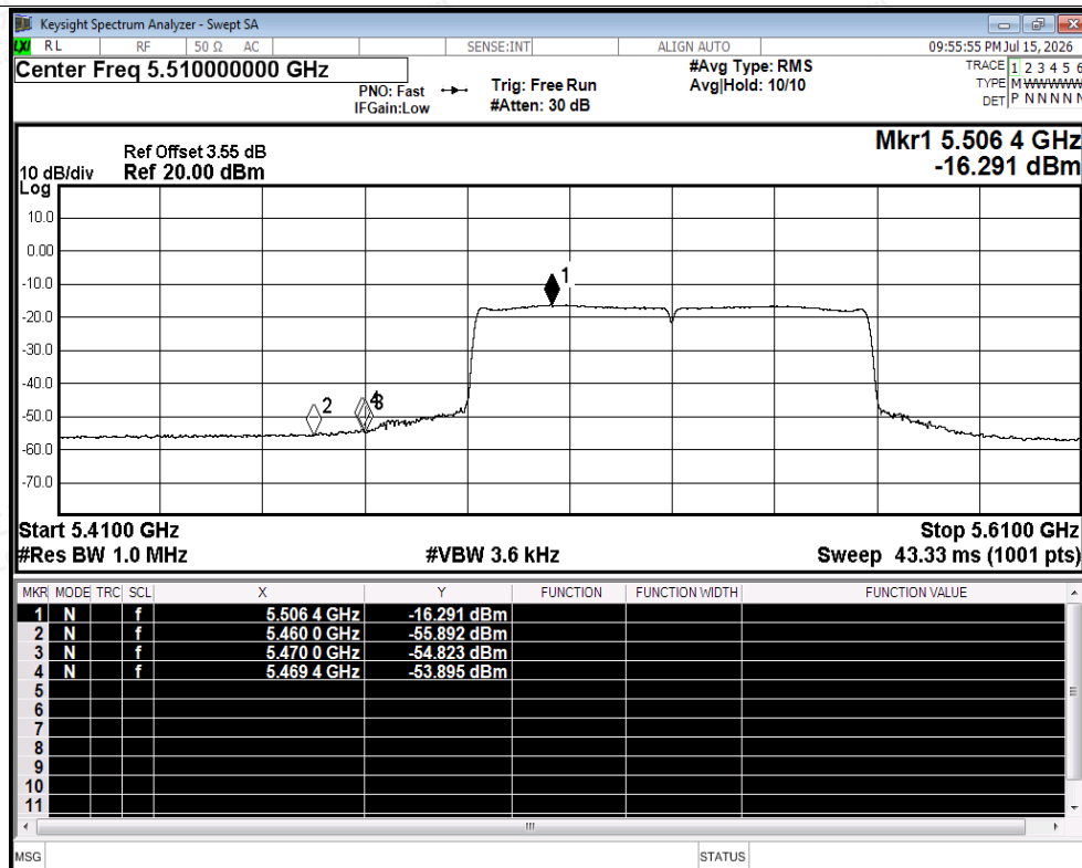
Restrict Band NVNT ax80 5530MHz Ant2 Average
