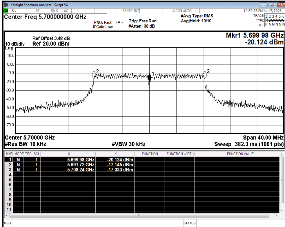
Freq. Stability NVNT a 5700MHz Ant2
