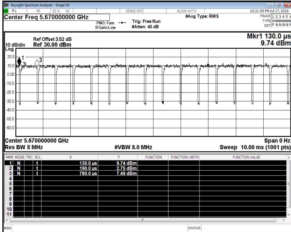
Duty Cycle NVNT n40 5670MHz Ant1
