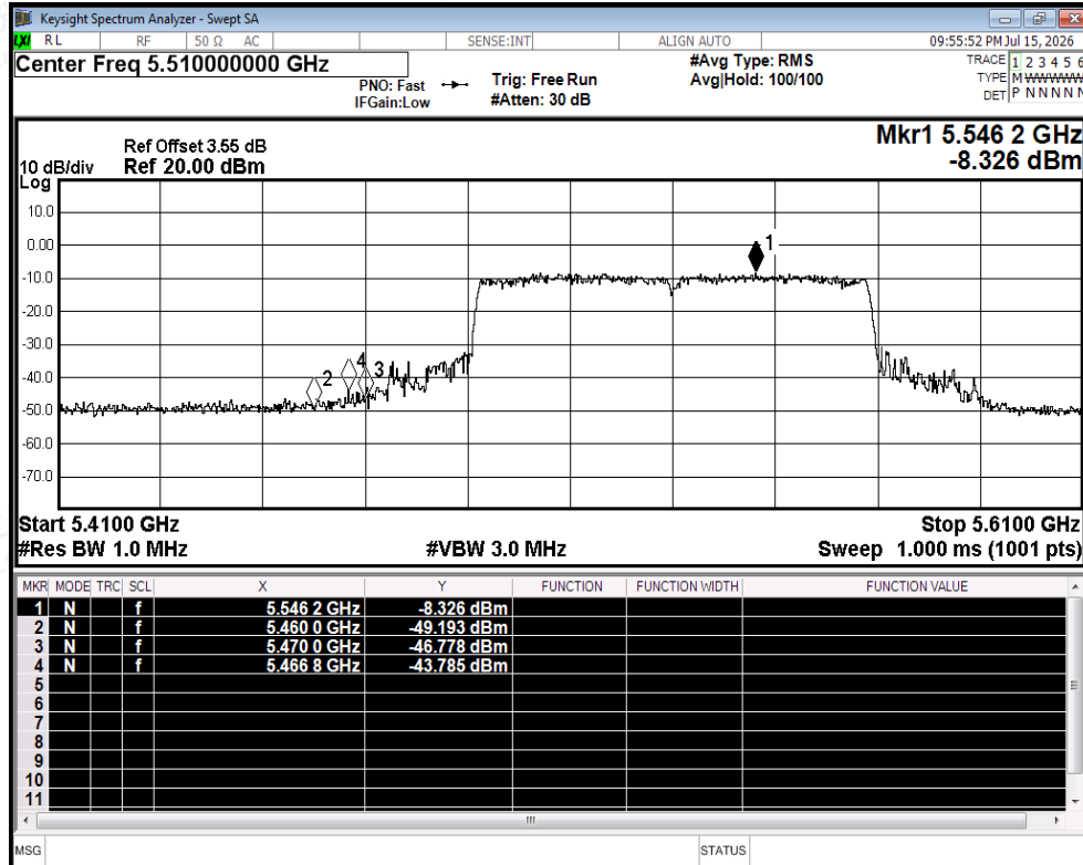
Restrict Band NVNT ax80 5530MHz Ant2 Peak
