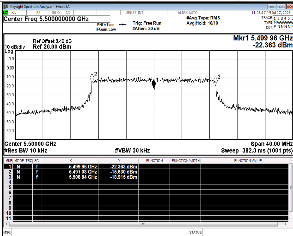
Freq. Stability NVNT ac20 5500MHz Ant2
