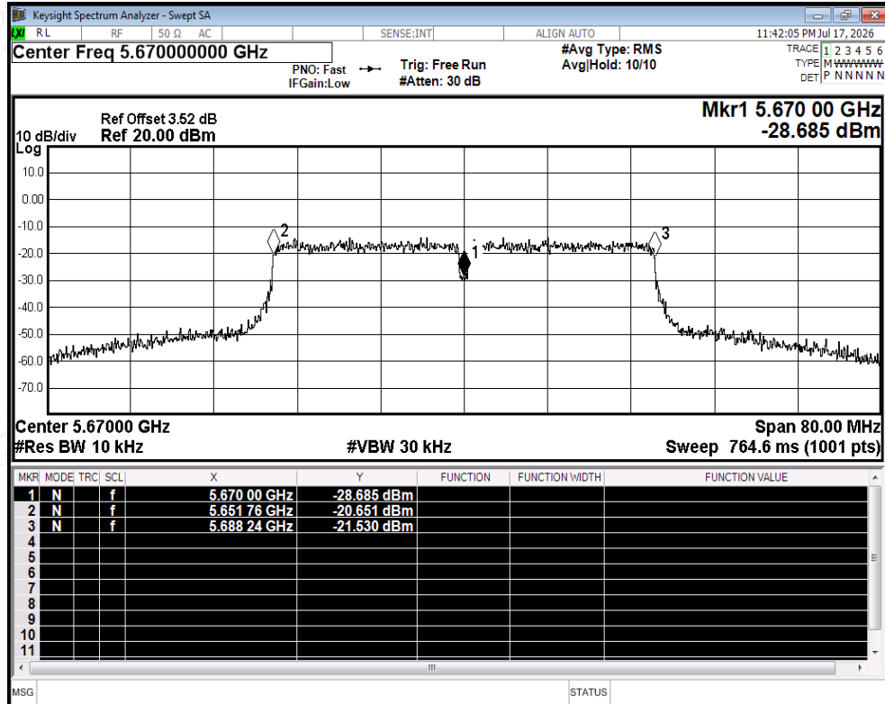
Freq. Stability NVNT ac40 5670MHz Ant2
