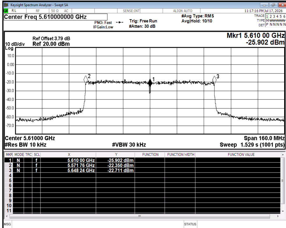
Freq. Stability NVNT ac80 5610MHz Ant2
