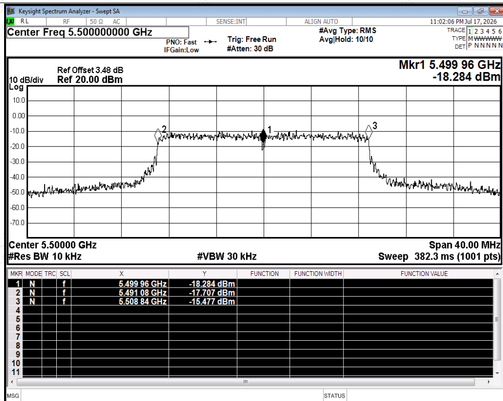
Freq. Stability NVNT n20 5500MHz Ant2
