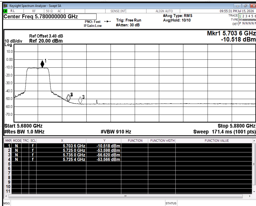
Restrict Band NVNT ax20 5700MHz Ant2 Average
