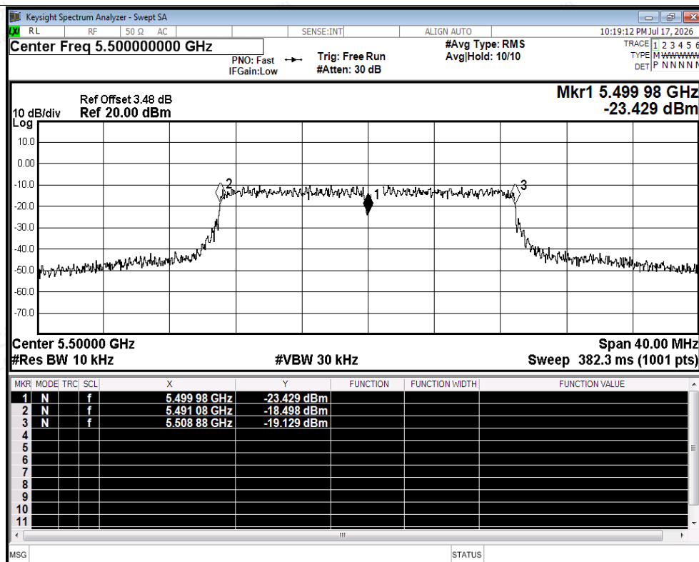
Freq. Stability NVNT ax20 5500MHz Ant1
