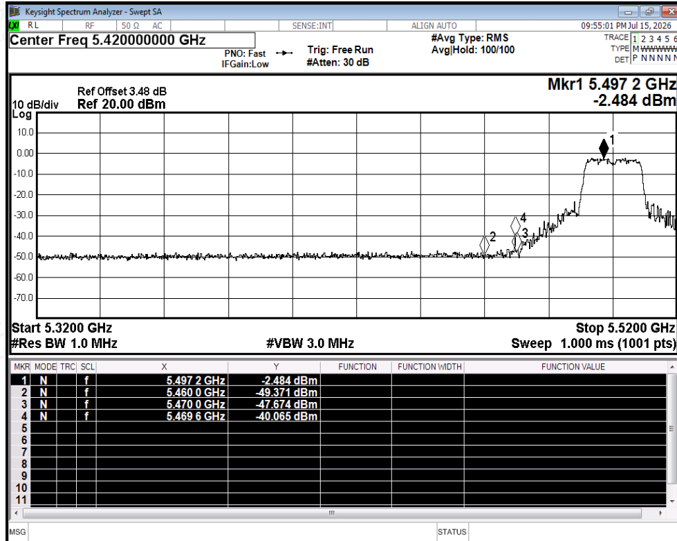
Restrict Band NVNT ax20 5500MHz Ant2 Peak
