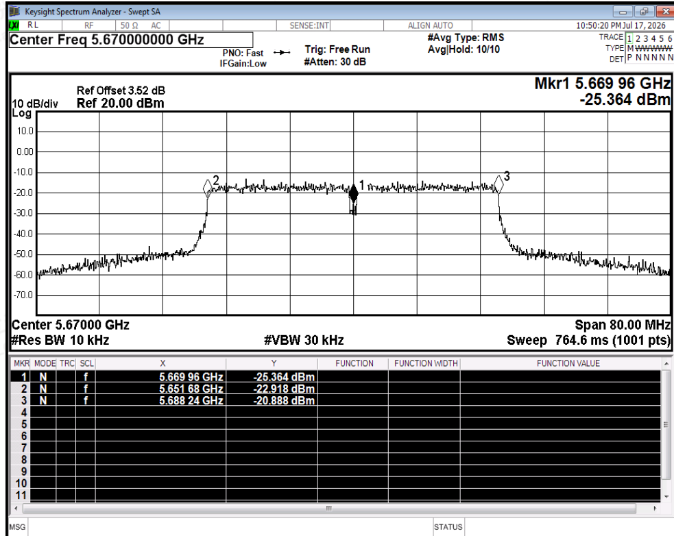
Freq. Stability NVNT ax40 5670MHz Ant1
