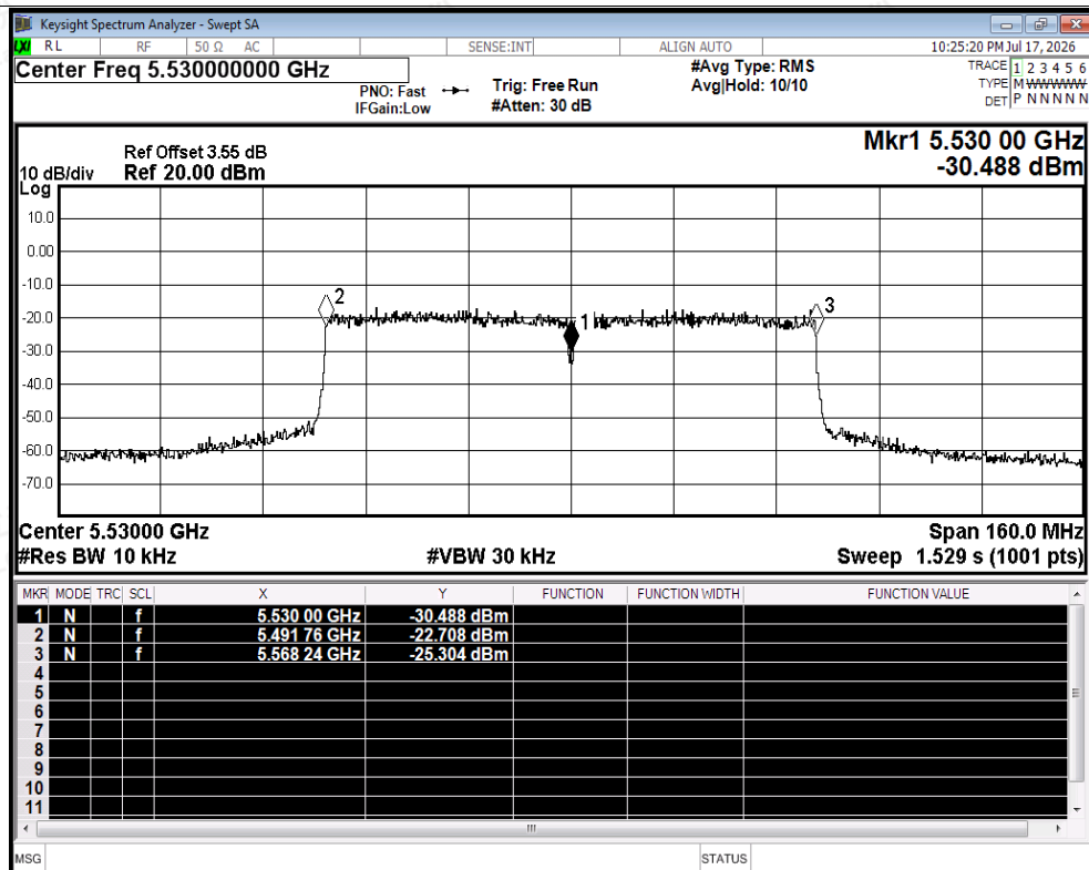
Freq. Stability NVNT ax80 5530MHz Ant1
