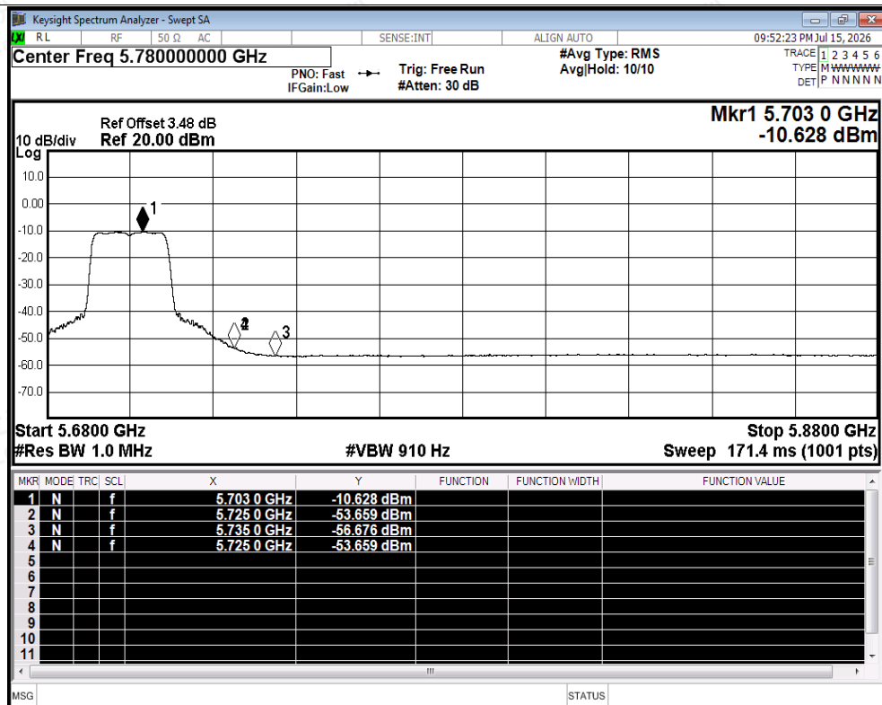
Restrict Band NVNT n20 5700MHz Ant2 Average
