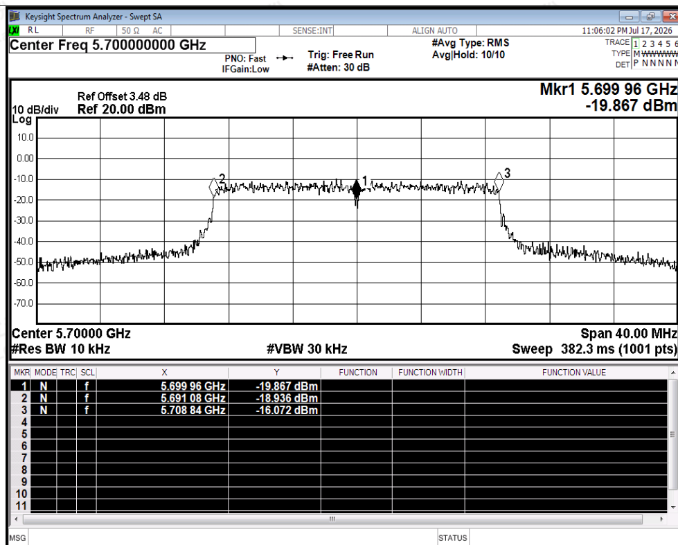
Freq. Stability NVNT n20 5700MHz Ant2
