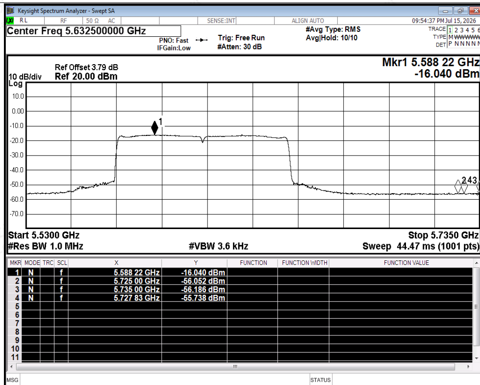
Restrict Band NVNT ac80 5610MHz Ant2 Average
