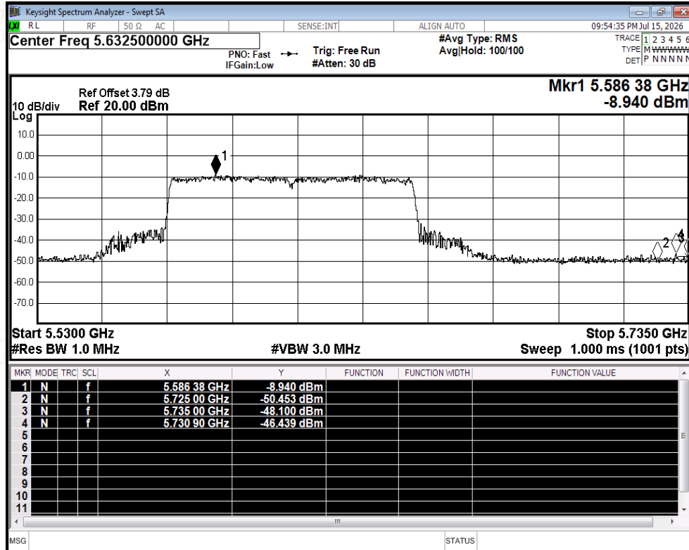
Restrict Band NVNT ac80 5610MHz Ant2 Peak
