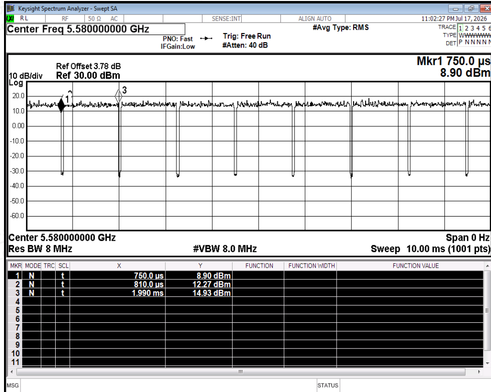
Duty Cycle NVNT n20 5580MHz Ant2
