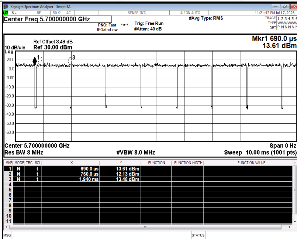
Duty Cycle NVNT ax20 5700MHz Ant2
