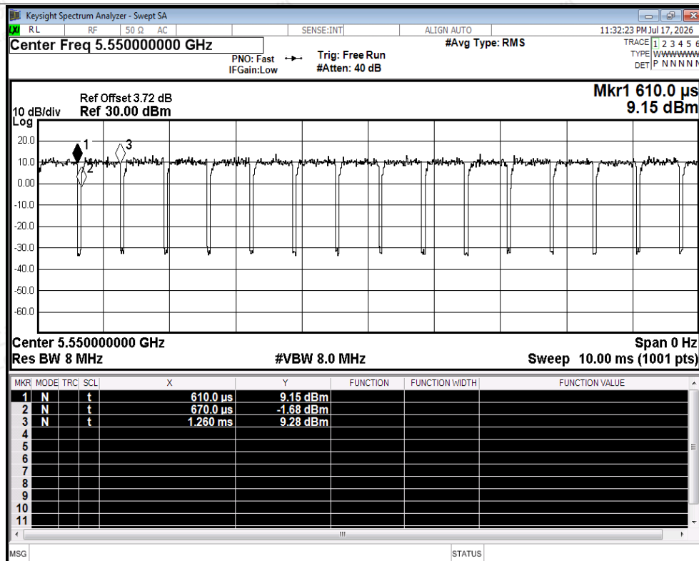
Duty Cycle NVNT n40 5550MHz Ant2
