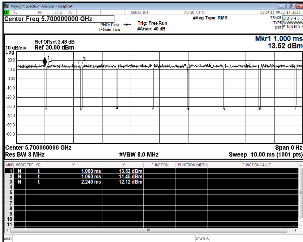
Duty Cycle NVNT n20 5700MHz Ant2
