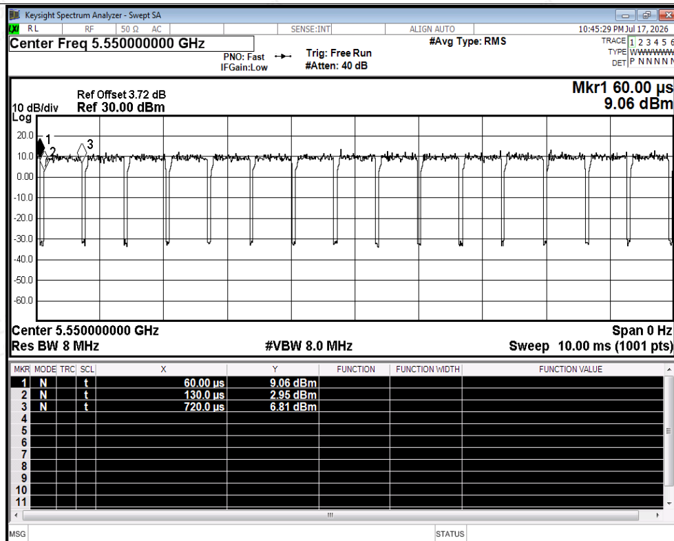
Duty Cycle NVNT ax40 5550MHz Ant1
