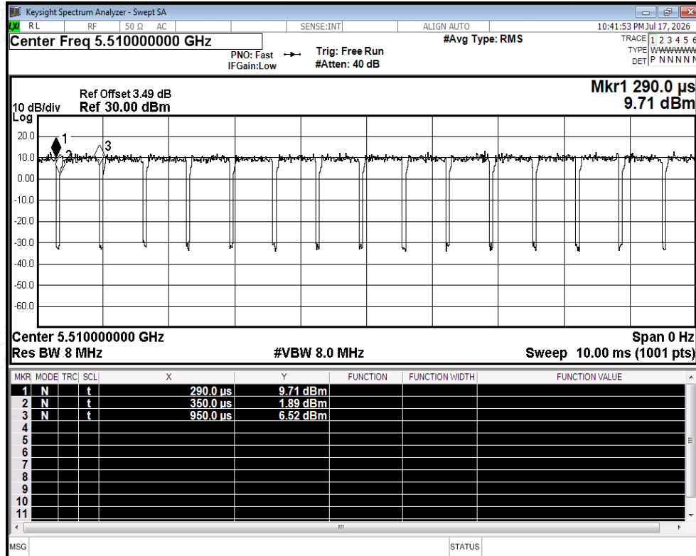
Duty Cycle NVNT ax40 5510MHz Ant1
