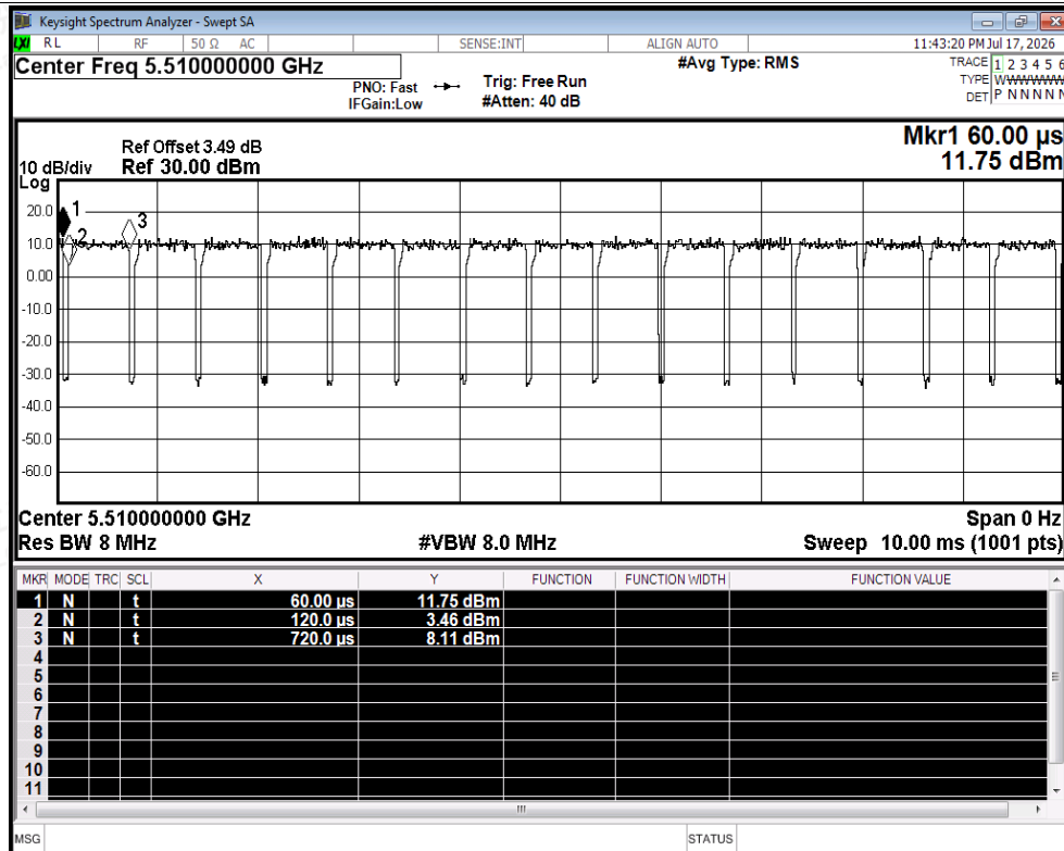
Duty Cycle NVNT ax40 5510MHz Ant2
