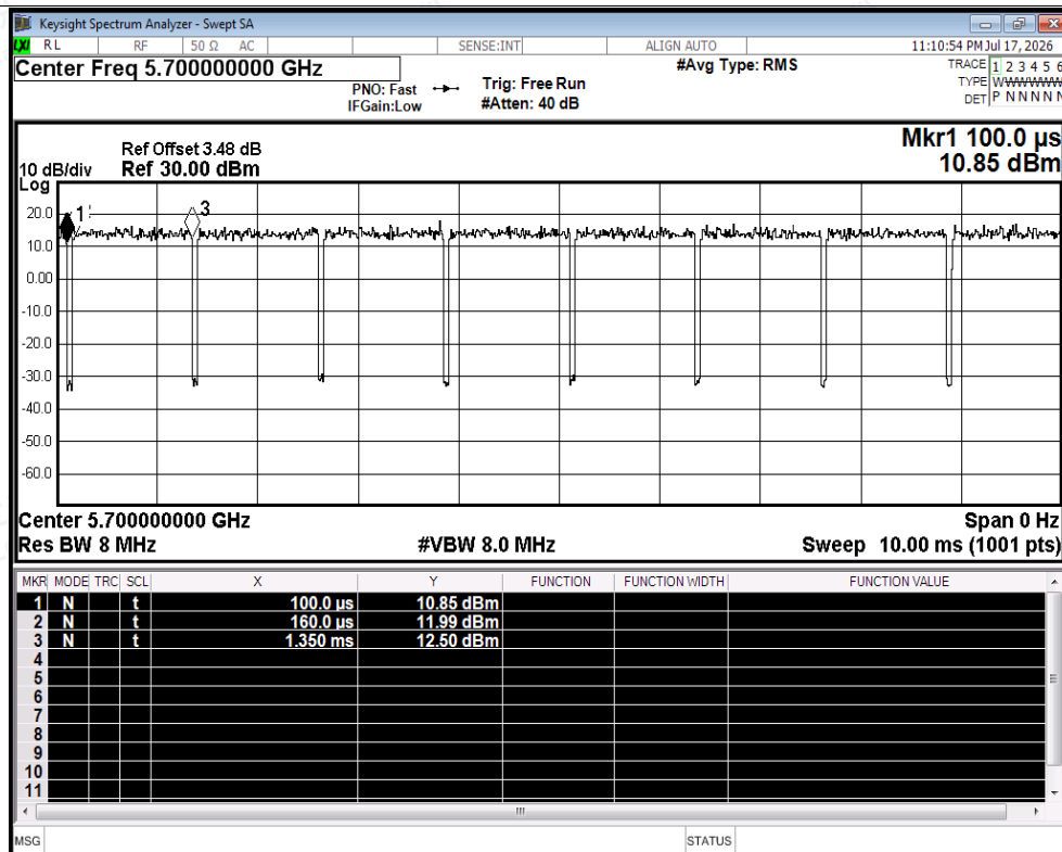
Duty Cycle NVNT ac20 5700MHz Ant2
