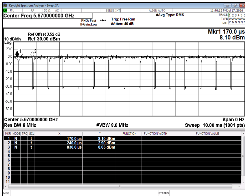
Duty Cycle NVNT ac40 5670MHz Ant2
