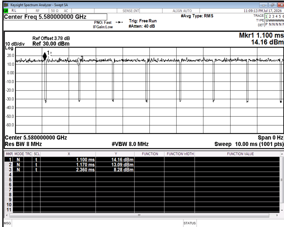
Duty Cycle NVNT ac20 5580MHz Ant2
