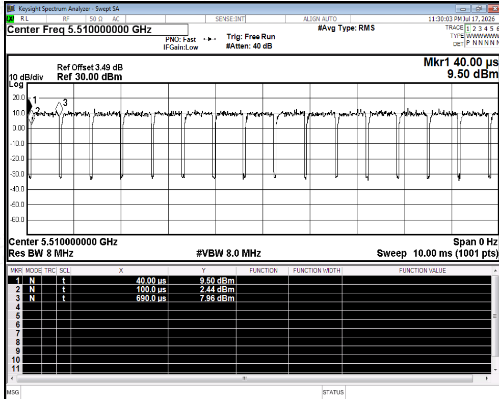
Duty Cycle NVNT n40 5510MHz Ant2
