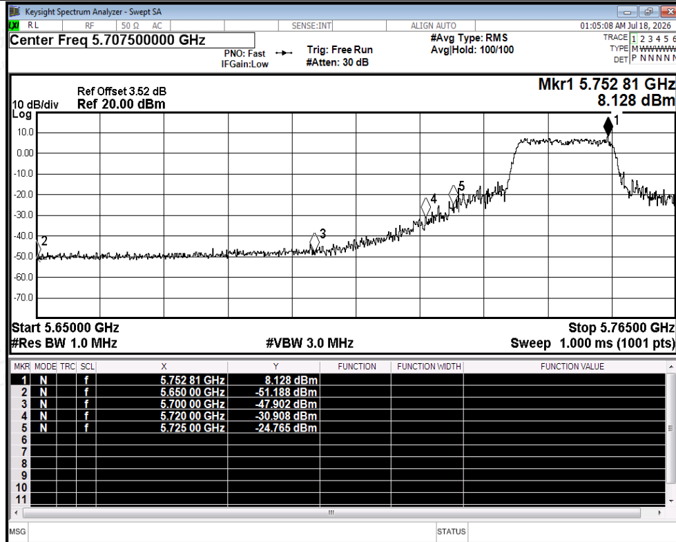
Restrict Band NVNT ax20 5745MHz Ant2 Peak
