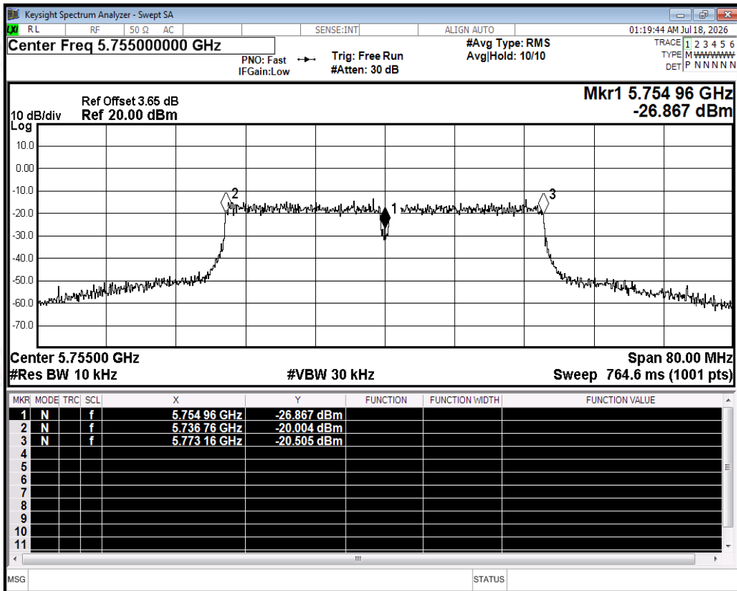
Freq. Stability NVNT ax40 5755MHz Ant2
