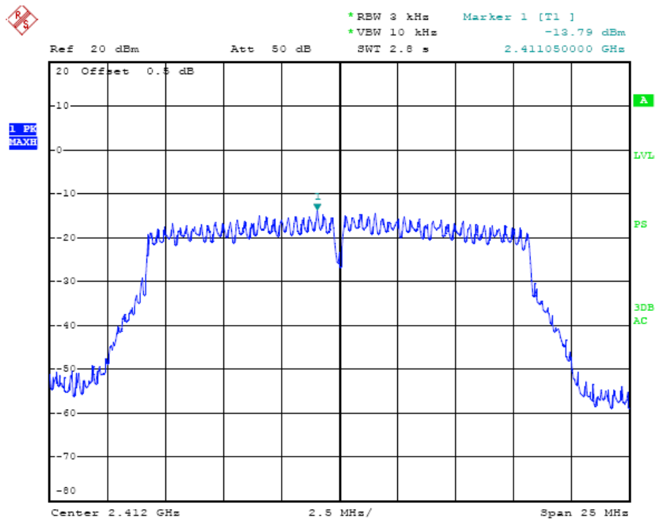
Channel 01 (2412MHz)
