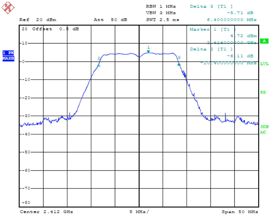
Channel 01 (2412MHz)
