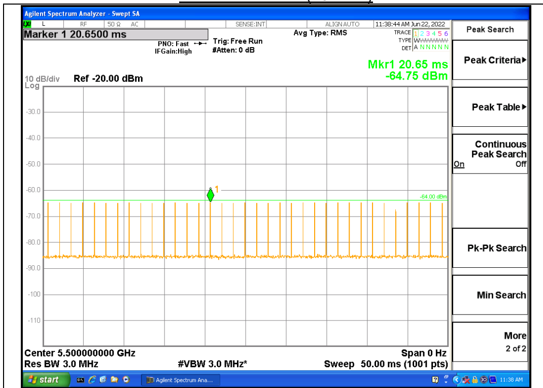
Radar Waveform (20 MHz)
