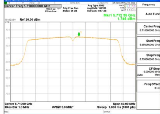
ANT1_802.11ac_VHT40_UNI1 2C
