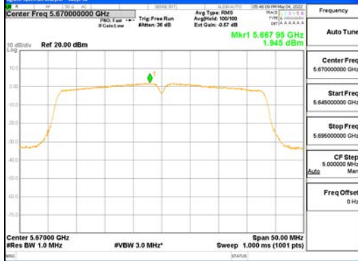
ANT1_802.11ac_VHT40_UNI1 2C
