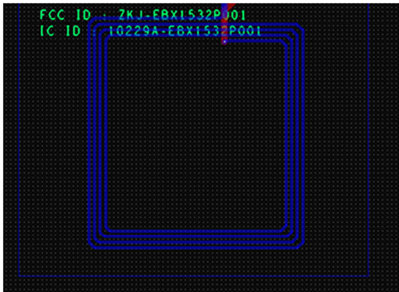
FCC and IC identifiers on Silkscreen of the PCB
