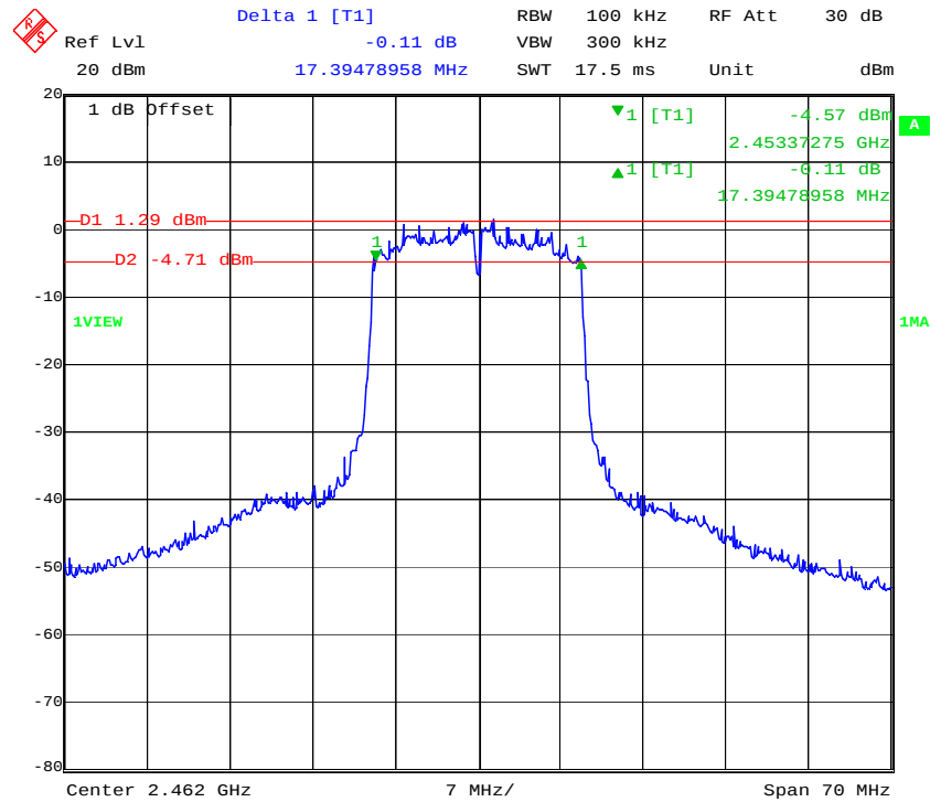
6dB Bandwidth Plot (Channel 11) - 802.11n mode
