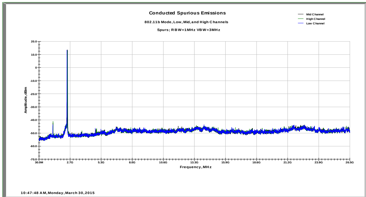
Conducted Spurious Emissions - 802.11b Mode
