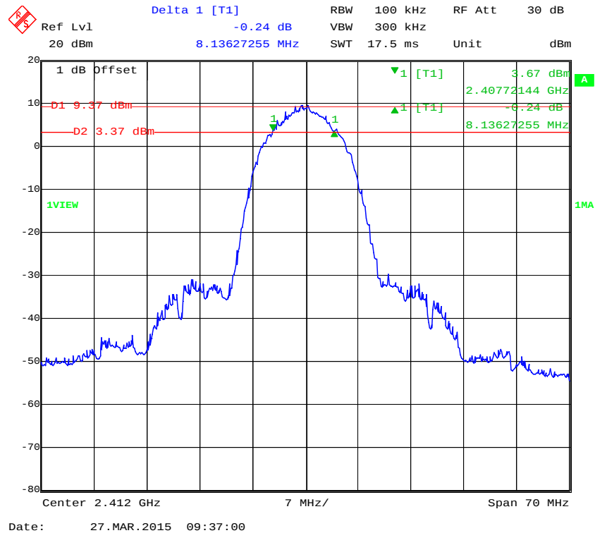
6dB Bandwidth Plot (Channel 1) – 802.11b mode
