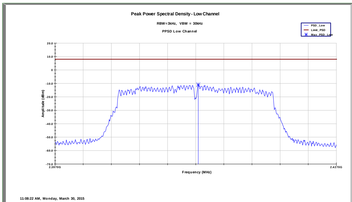
Power Spectral Density – Channel 1 802.11g mode
