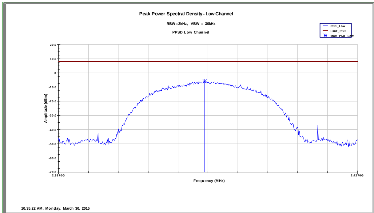
Power Spectral Density – Channel 1 802.11b mode
