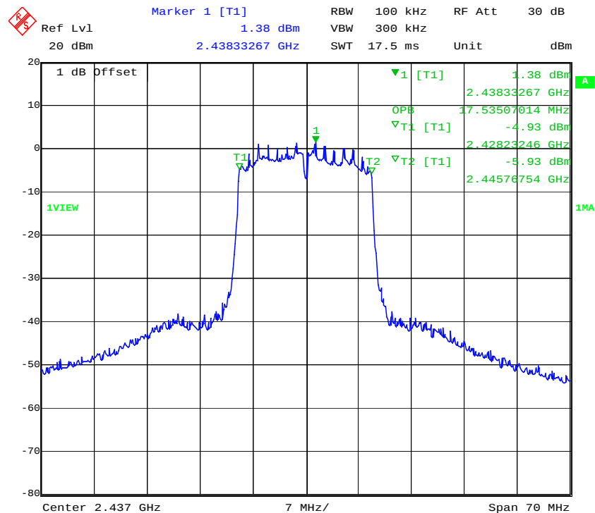
99% Power Bandwidth Plot (Channel 6) - 802.11n mode
