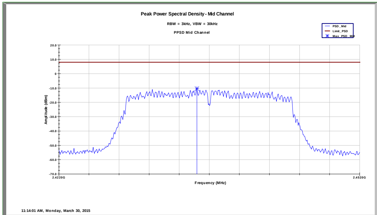
Power Spectral Density – Channel 6 802.11g mode
