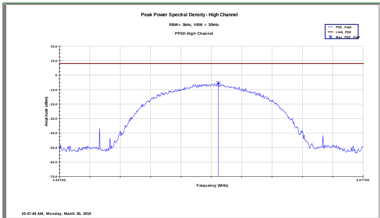
Power Spectral Density – Channel 11 802.11b mode
