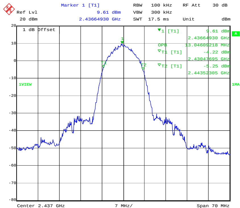
99% Power Bandwidth Plot (Channel 6) – 802.11b mode
