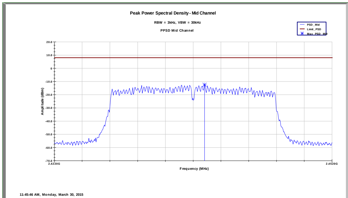
Power Spectral Density – Channel 6 802.11n mode
