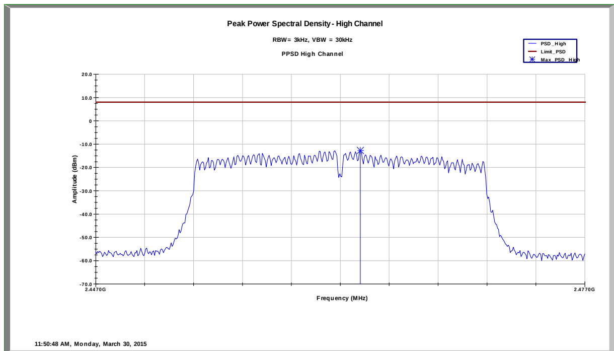
Power Spectral Density – Channel 11 802.11n mode
