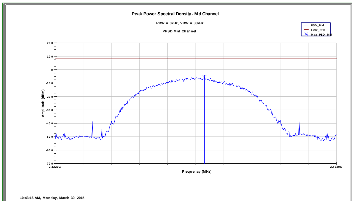
Power Spectral Density – Channel 6 802.11b mode
