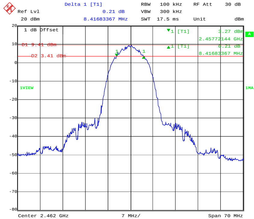
6dB Bandwidth Plot (Channel 11) – 802.11b mode
