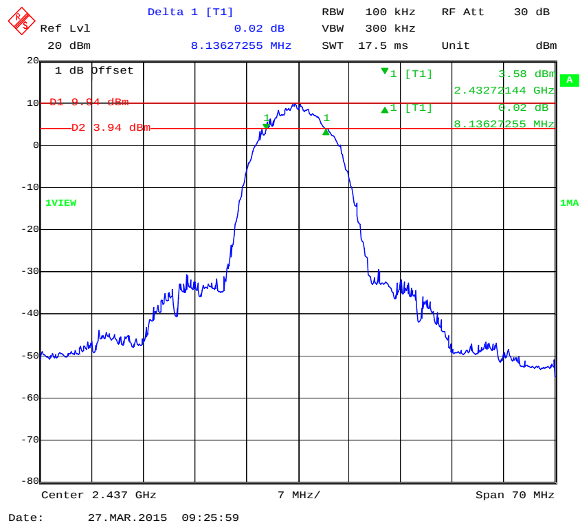
6dB Bandwidth Plot (Channel 6) – 802.11b mode
