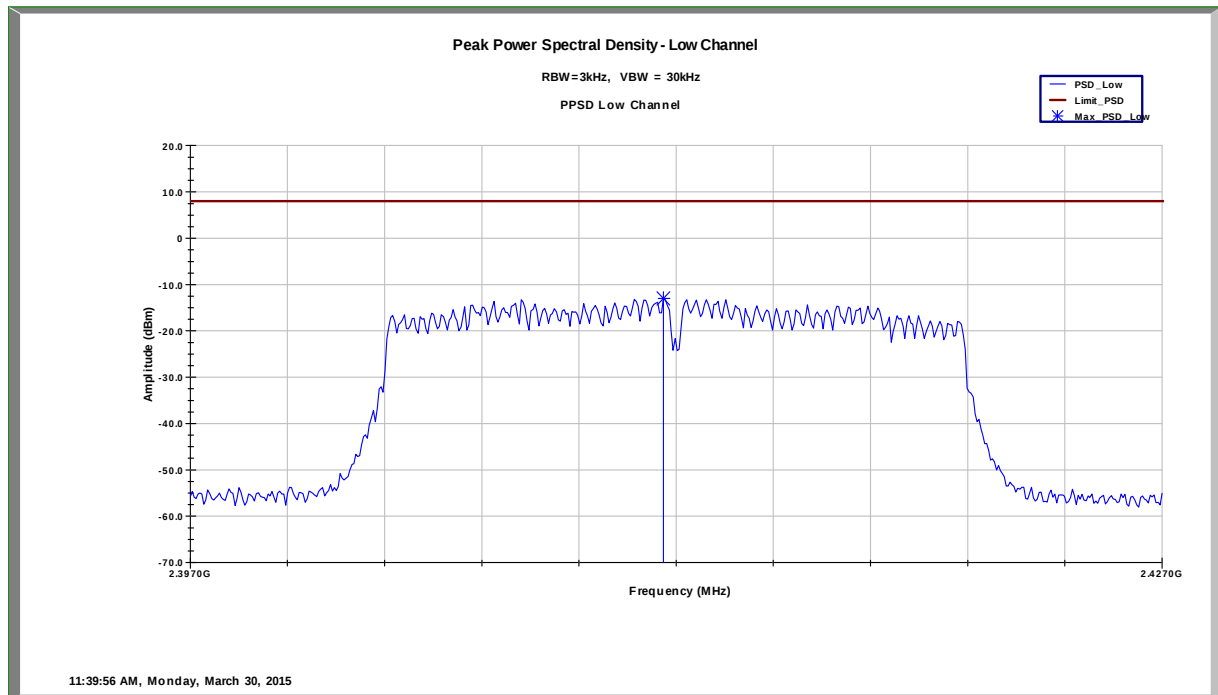
Power Spectral Density – Channel 1 802.11n mode
