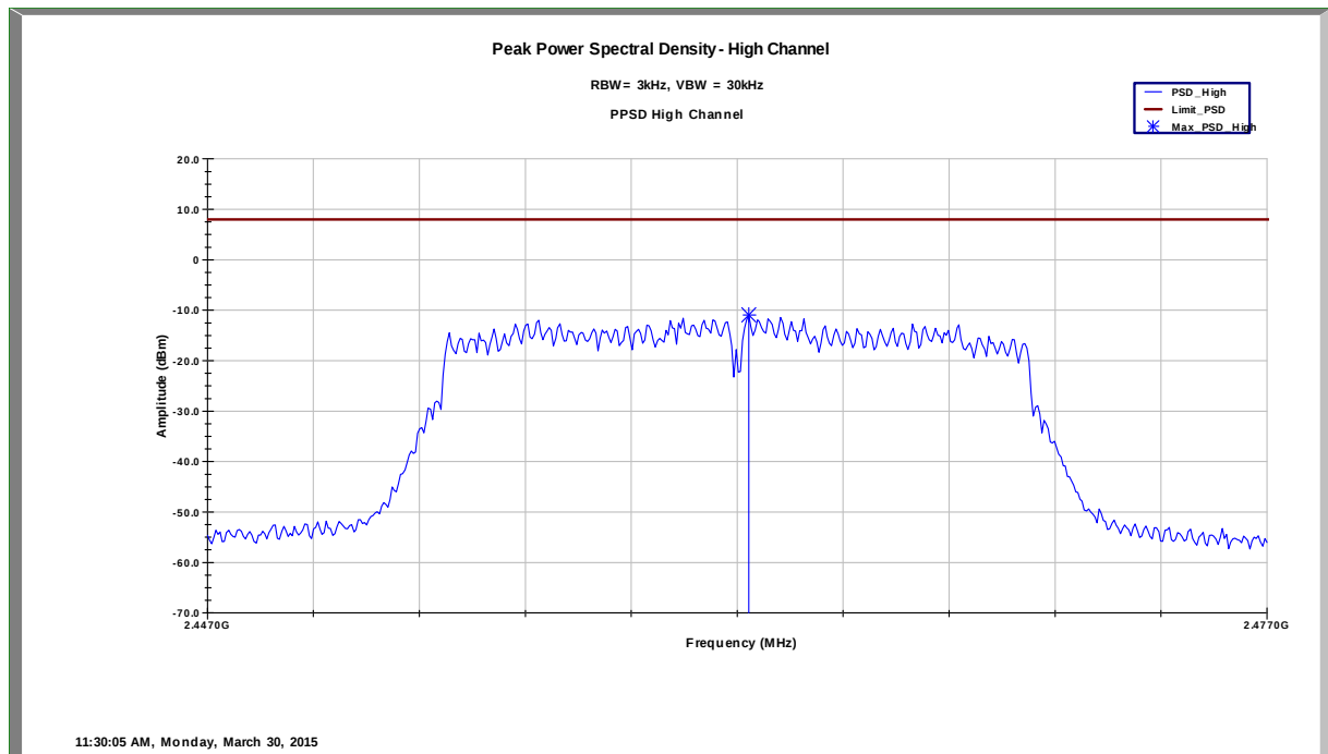
Power Spectral Density – Channel 11 802.11g mode
