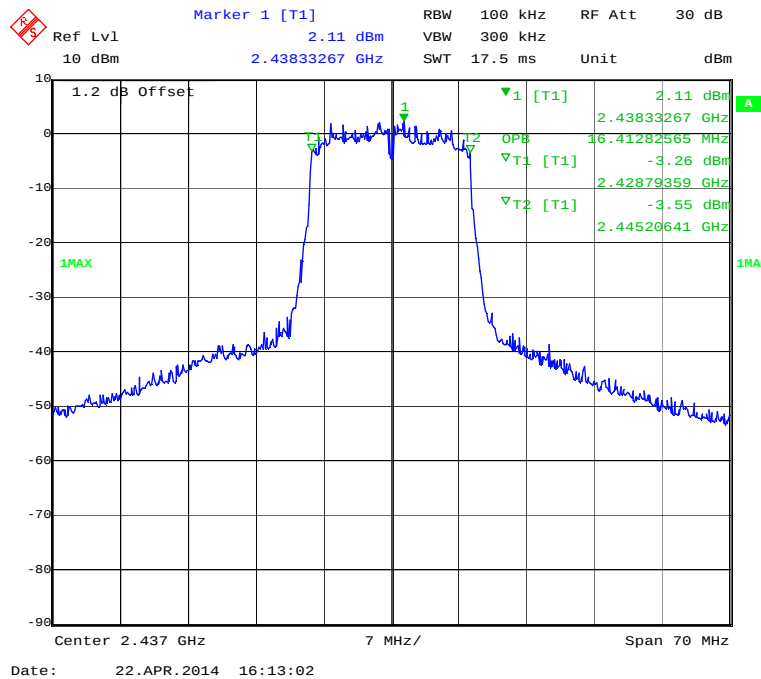
99% Power Bandwidth Plot (Channel 6) – 802.11g mode
