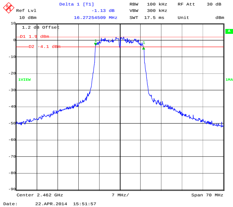
6dB Bandwidth Plot (Channel 11) – 802.11g mode
