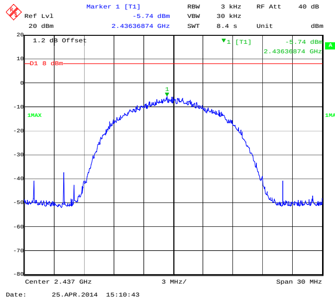
Power Spectral Density – Channel 6 802.11b mode
