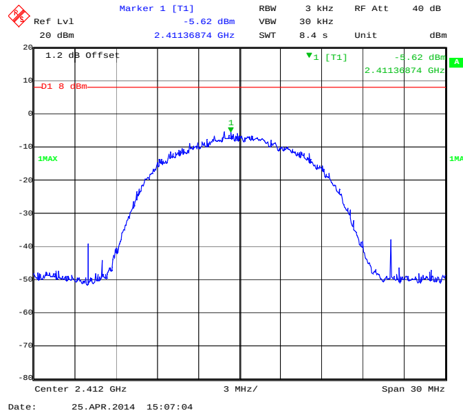
Power Spectral Density – Channel 1 802.11b mode
