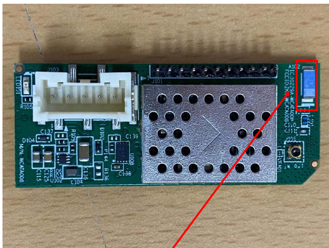
TX Antenna
