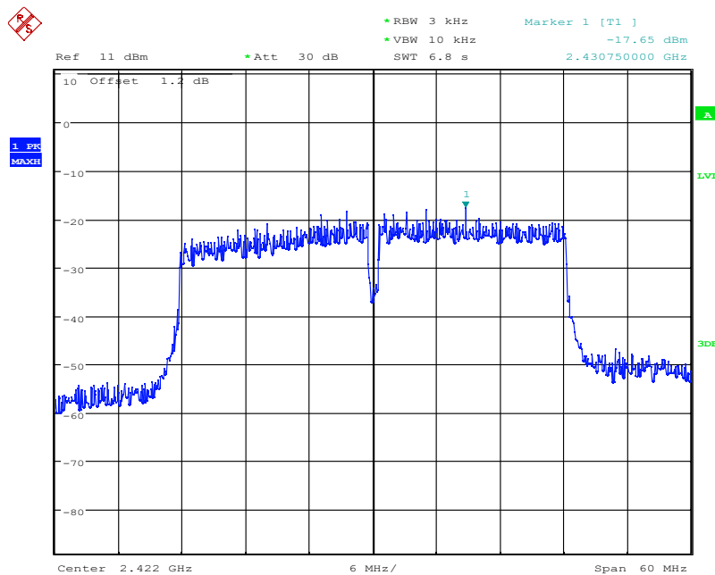
Fig.63 Power spectral density: CH1,11n
