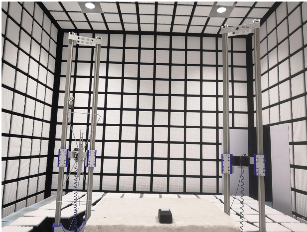
Pic1. Radiated spurious emission (Above 1GHz)
