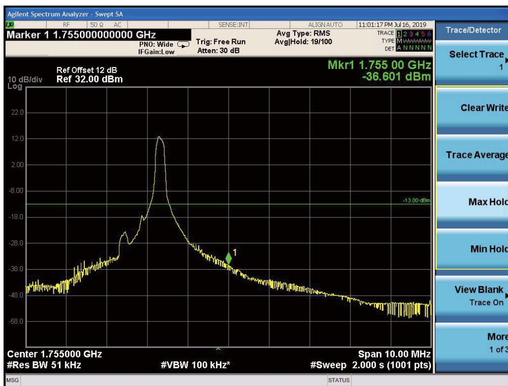
Band4-High Channel-3MHz Bandwidth-1RB-16QAM
