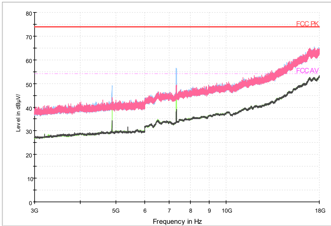
Fig.22 Radiated emission: Ch19, 1M 3GHz-18GHz
