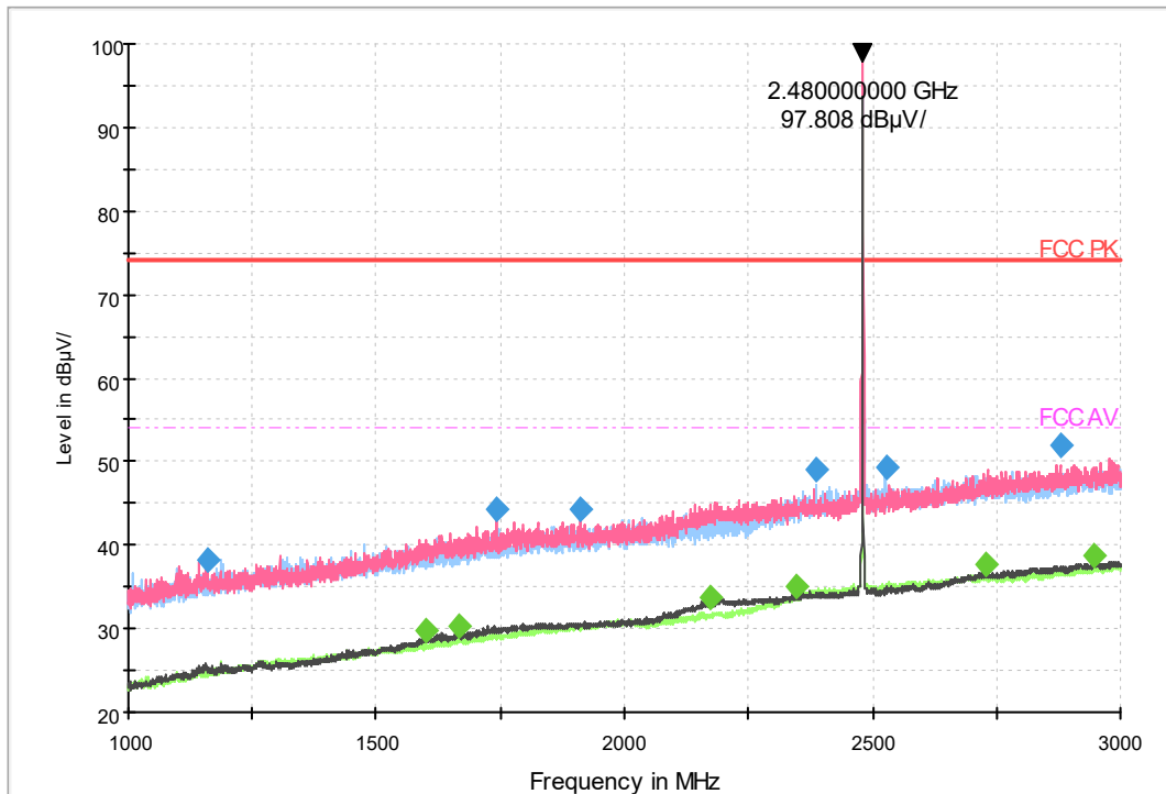
Fig.23 Radiated emission: 1M Ch39, 1GHz-3GHz
