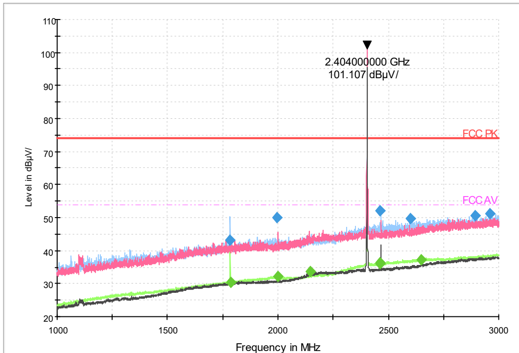
Fig.19 Radiated emission: Ch0, 1M 1GHz-3GHz
