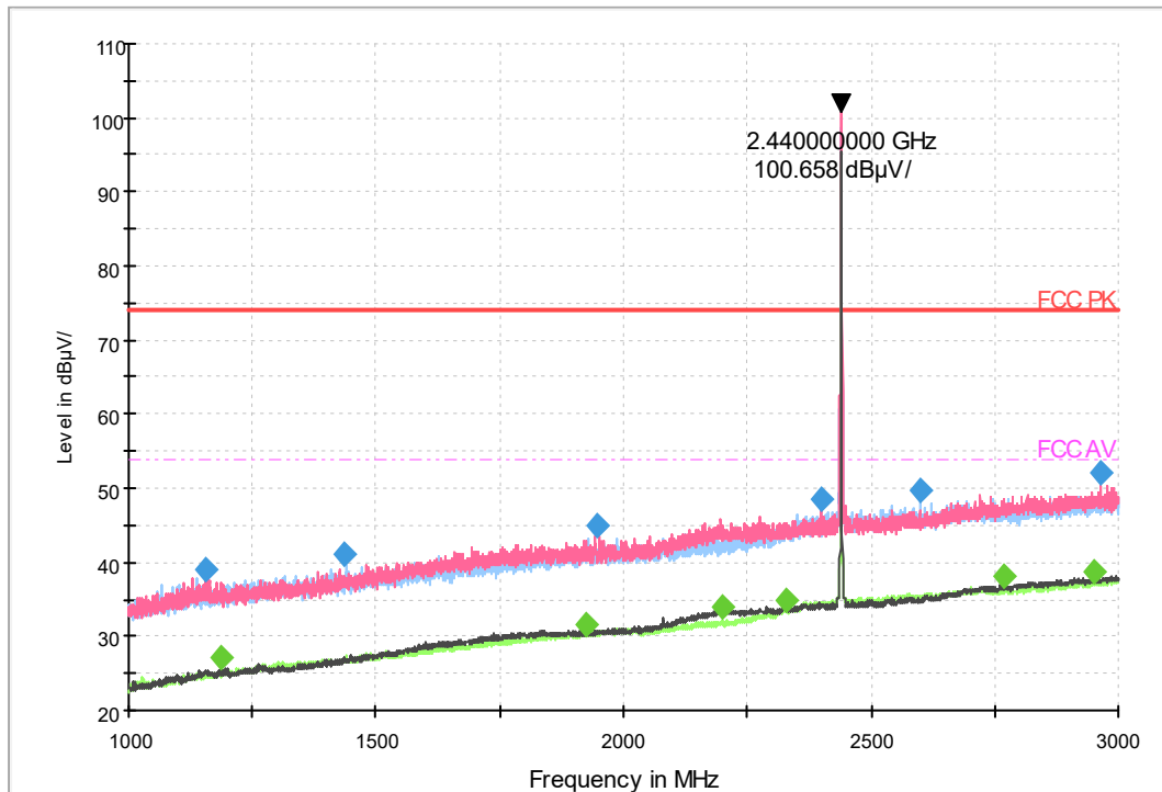
Fig.21 Radiated emission: Ch19,1M 1GHz-3GHz
