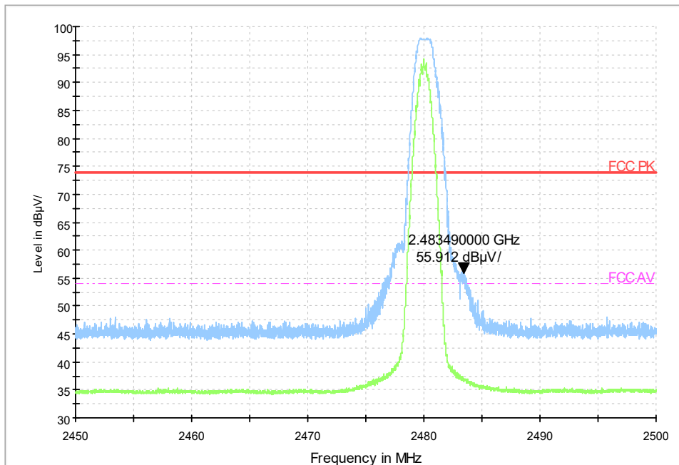
BAND EDGERE 1GHz-3GHz 2.45-2.5G
