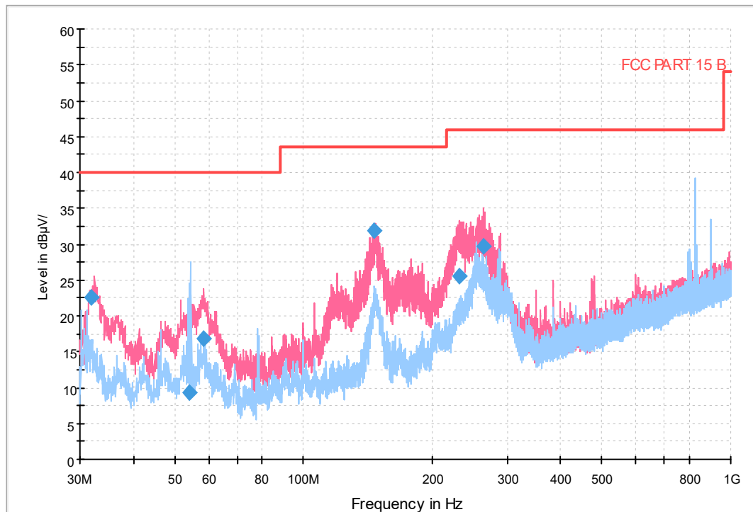
Fig.18 Radiated emission: Ch19, 1M, 30MHz-1GHz
