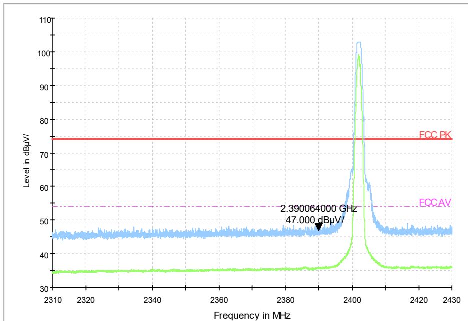
BAND EDGERE 1GHz-3GHz 2.31-2.43G
