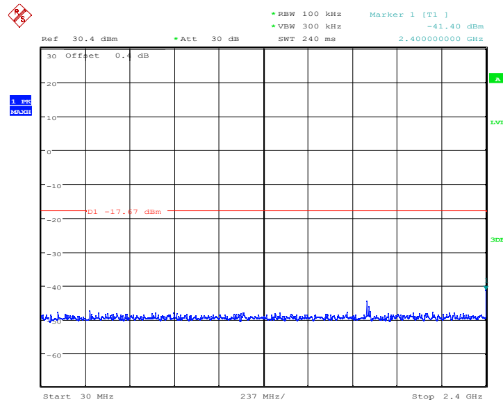
Fig.9 Conducted spurious emission: 1M Ch0
