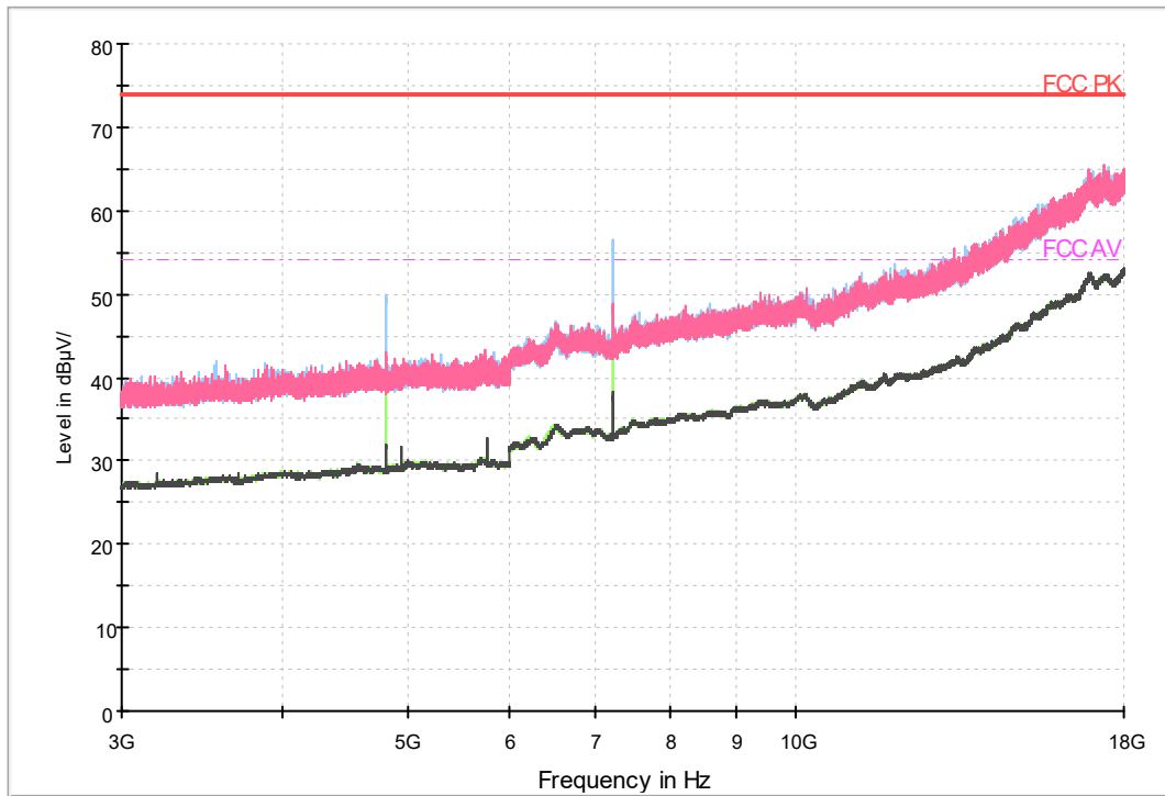
Fig.20 Radiated emission: Ch0, 1M, 3GHz-18GHz
