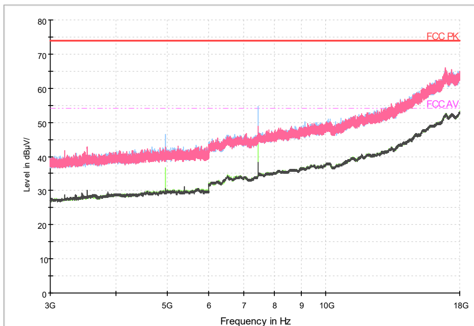
Fig.24 Radiated emission: Ch39, 1M 3GHz-18GHz
