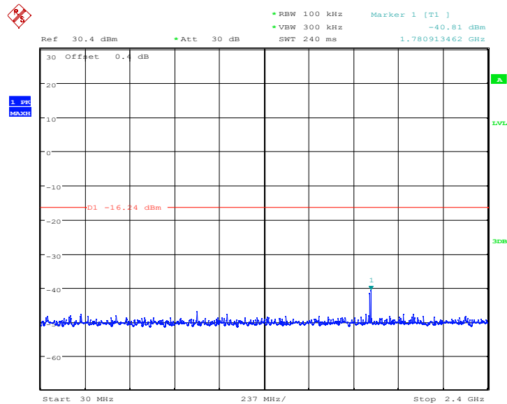
Fig.15 Conducted spurious emission: 1M Ch39
