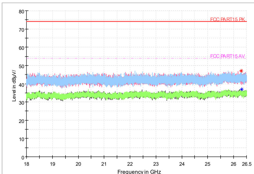
Fig.25 Radiated emission: 18 GHz - 26.5 GHz
