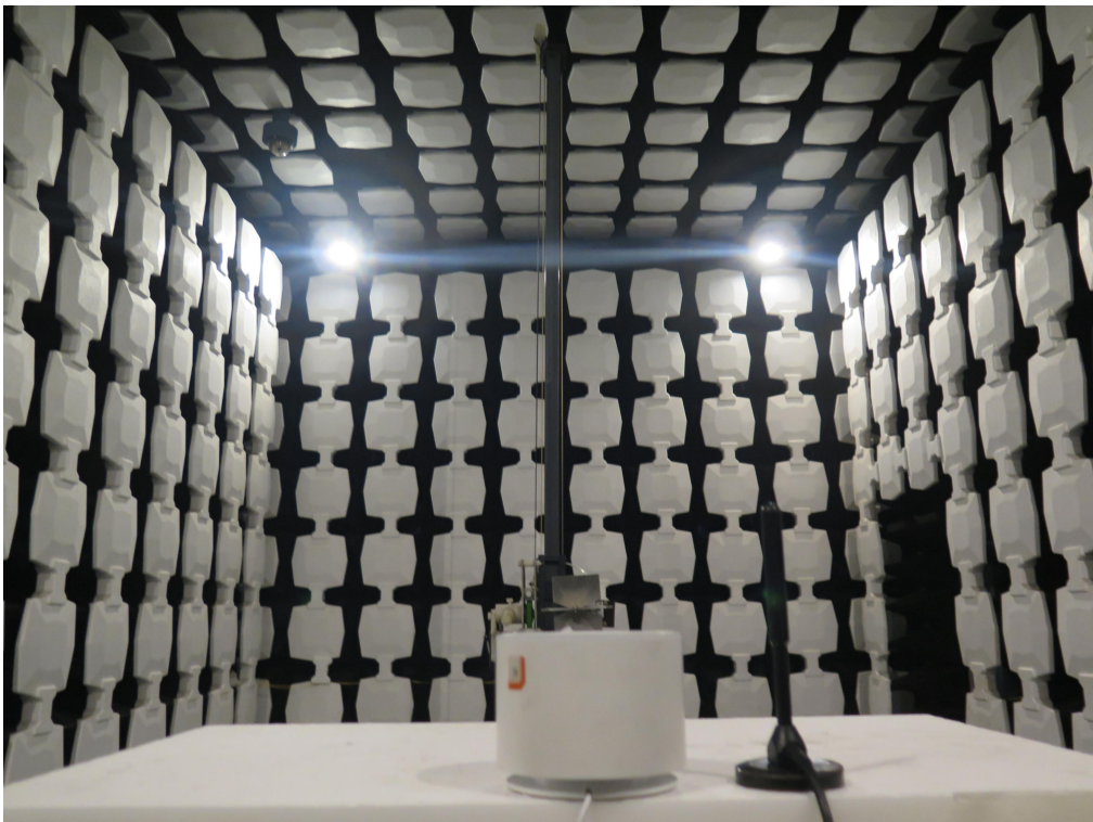
Pic4. Radiated spurious emission (1GHz-18GHz)
