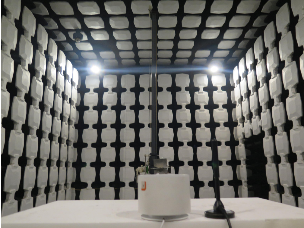
Pic2. Radiated spurious emission (1GHz-18GHz)
