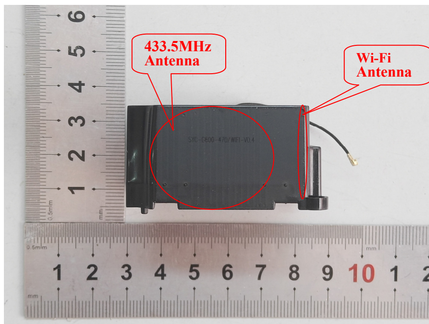
EUT – Wi-Fi&433.5MHz Antenna View
