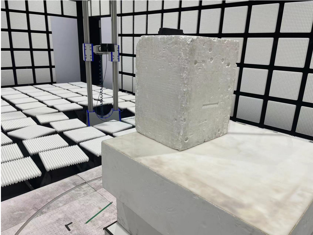
RSE_1GHz-20GHz
