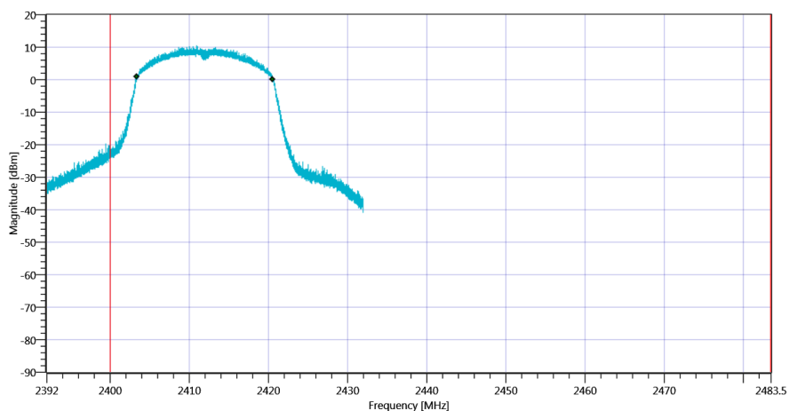
Plot_FCC Part 15.247 Bandwidth 99PCT-20dB ~ WLAN2G4 nHT20-mode_29092020_154504.png
