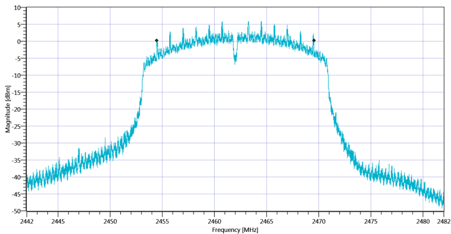
Plot_FCC Part 15.247 Bandwidth 6dB DTS ~ WLAN2G4 nHT20-mode_29092020_162005.png
