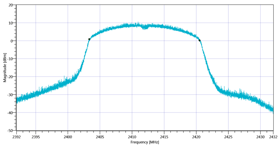
Plot_FCC Part 15.247 Bandwidth 99PCT-20dB ~ WLAN2G4 nHT20-mode 99PCT_29092020_154500.png
