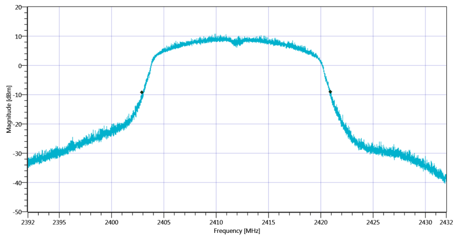
Plot_FCC Part 15.247 Bandwidth 99PCT-20dB ~ WLAN2G4 g-mode 20dB_29092020_151034.png
