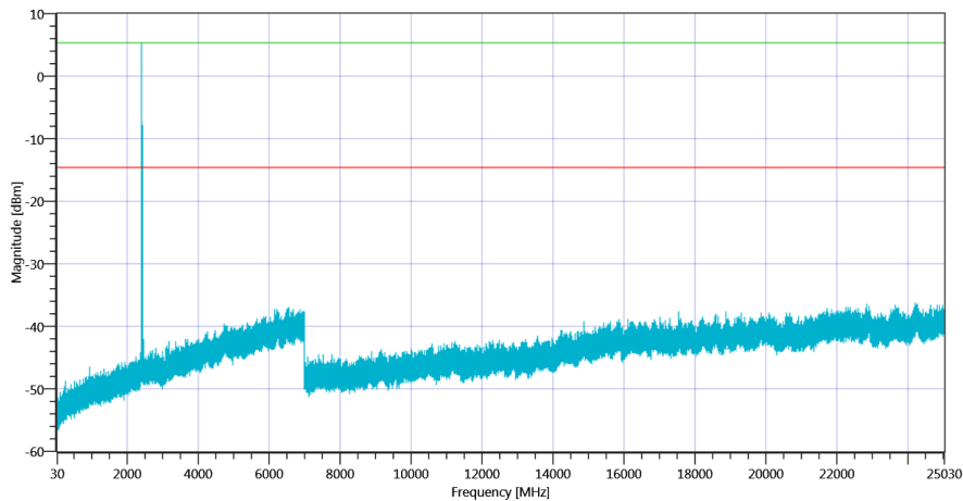
Plot_FCC Part 15.247 TX Spurious Conducted ~ WLAN2G4 b-mode 2412_29092020_141249.png
