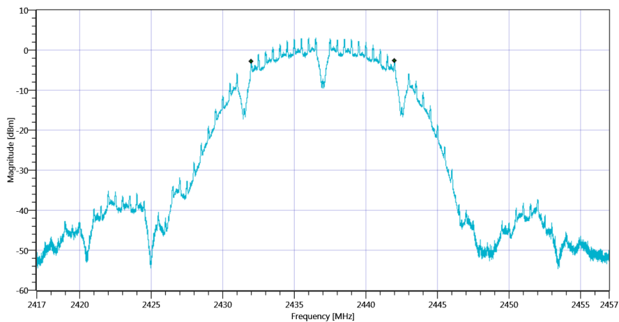
Plot_FCC Part 15.247 Bandwidth 6dB DTS ~ WLAN2G4 b-mode_29092020_144049.png
