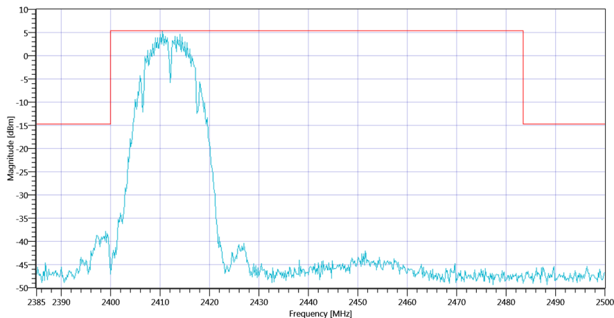
Plot_FCC Part 15.247 TX Spurious Conducted ~ WLAN2G4 b-mode 2412_29092020_141252.png
