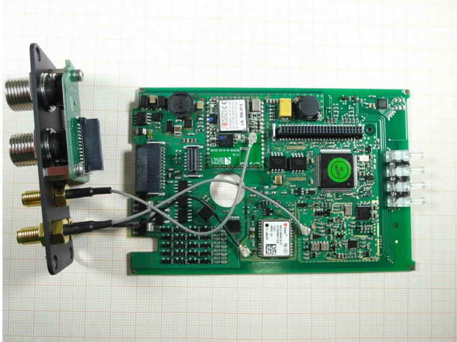
Photo 5: Top view PCB 2
