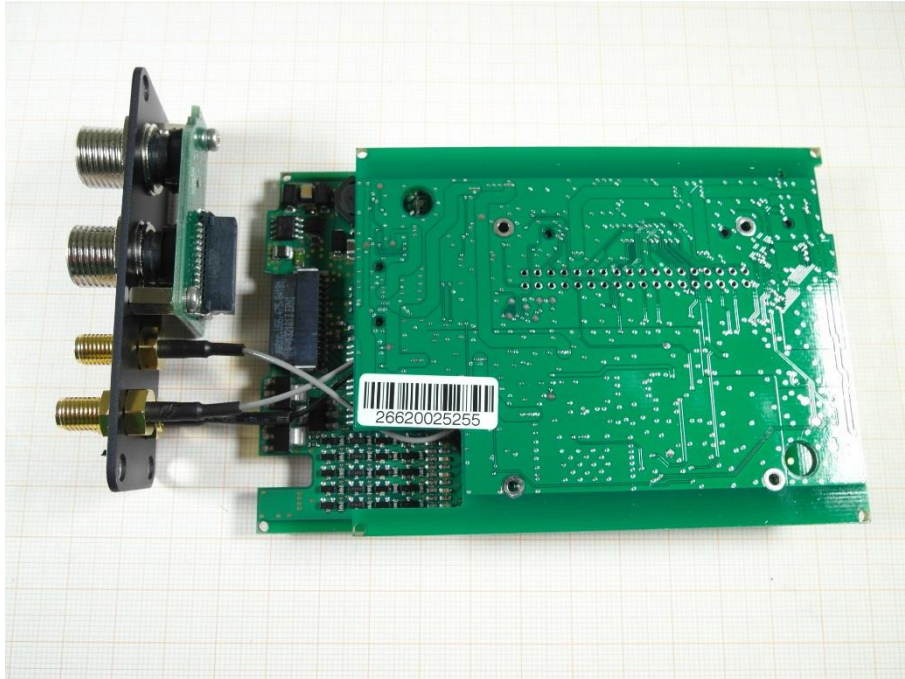
Photo 1: Bottom view PCB 1
