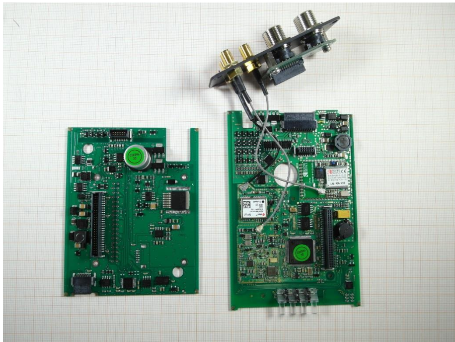
Photo 3: PCBs detached
