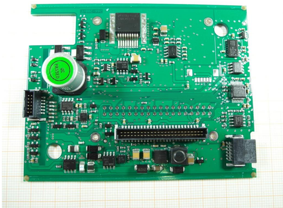
Photo 4: Top view PCB 1
