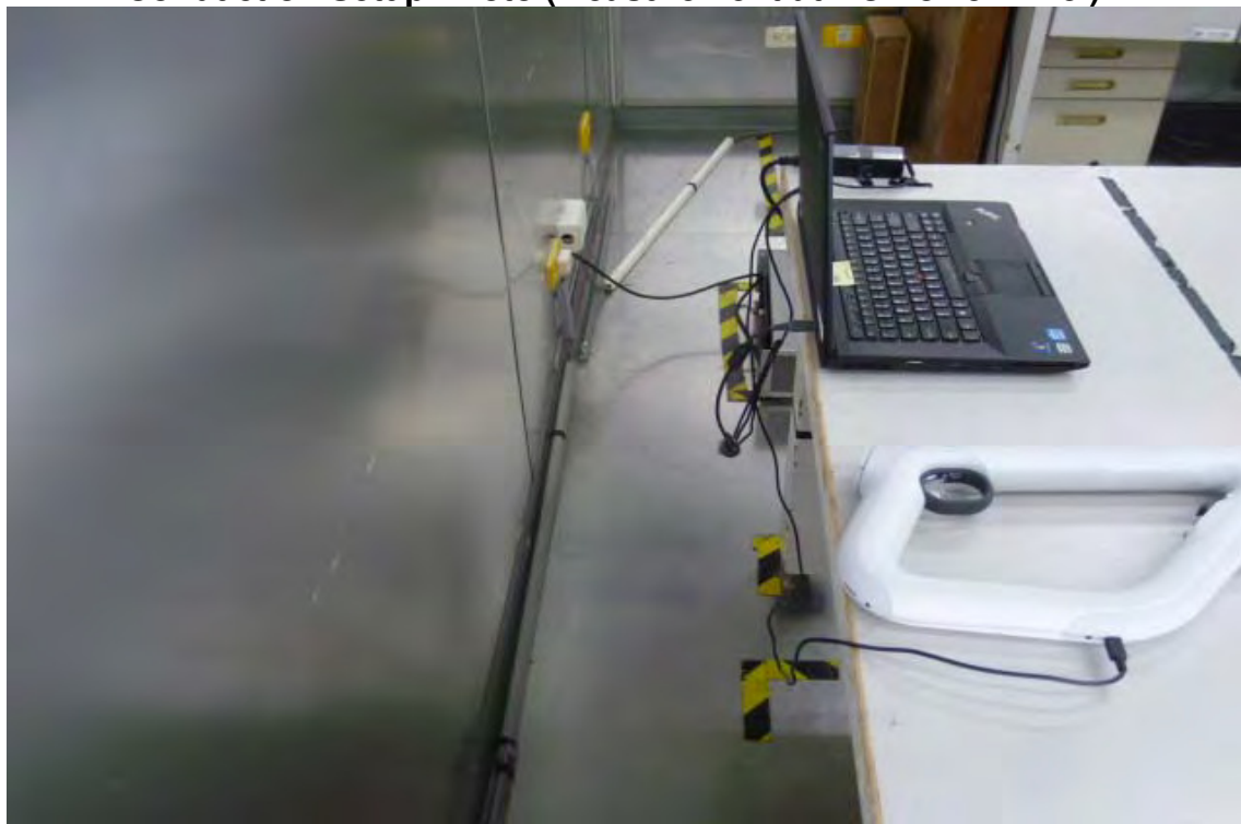
Conduction Setup Photo (Measurement at AC Power Line )-1
