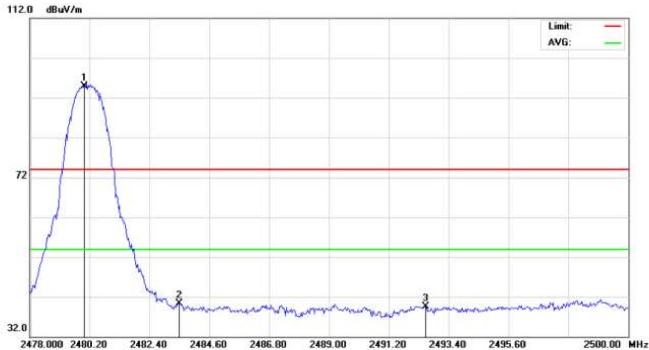
TEST PLOT OF BAND EDGE FOR HIGH CHANNEL (3Mbps)-Horizontal
