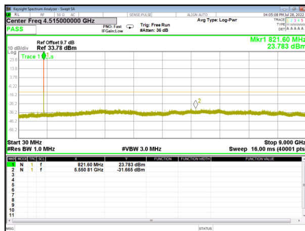
CDMA BC10 Middle Conducted Spurious
