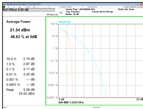
BC1_Lower
