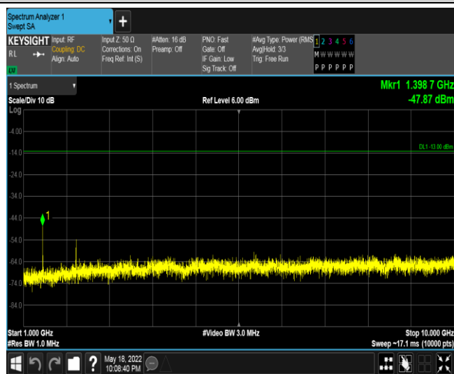
Band12-3MHz-16QAM-23025-1RB#0-Range3:1000~10000MHz
