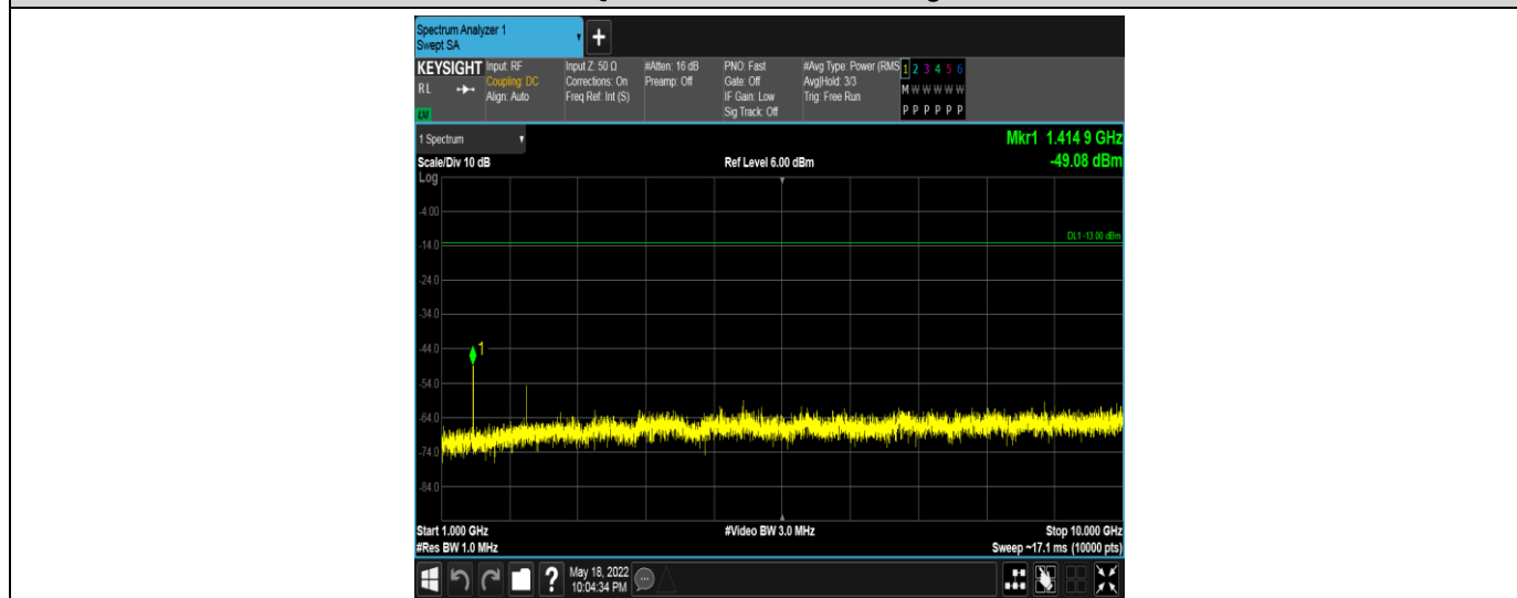
Band12-1.4MHz-16QAM-23095-1RB#0-Range3:1000~10000MHz
