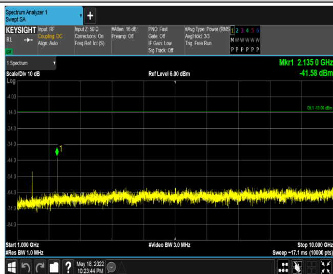
Band12-5MHz-QPSK-23155-1RB#0-Range3:1000~10000MHz
