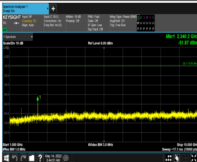
Band13-5MHz-16QAM-23230-1RB#0-Range3:1000~10000MHz
