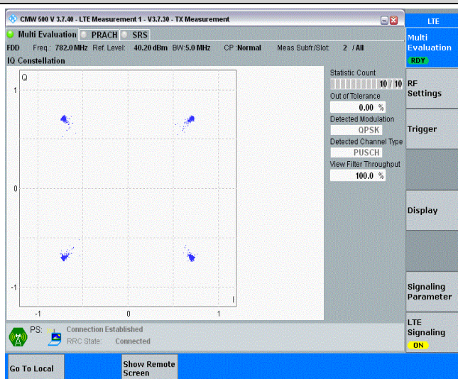
Band13-5MHz-QPSK-23230-25RB#0
