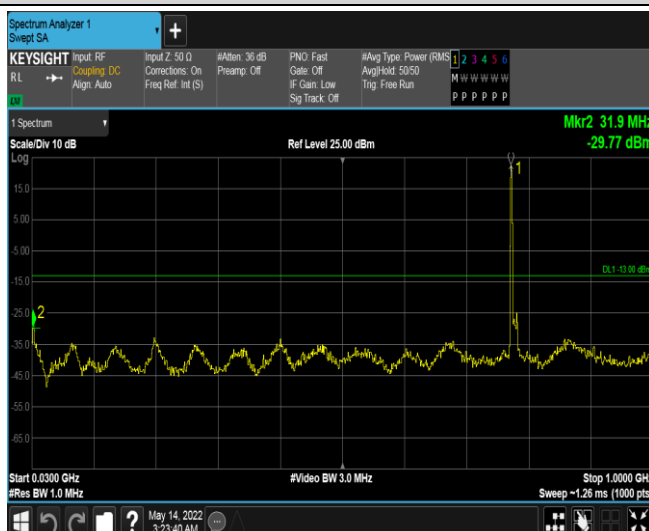
Band13-10MHz-QPSK-23230-1RB#0-Range2:30~1000MHz
