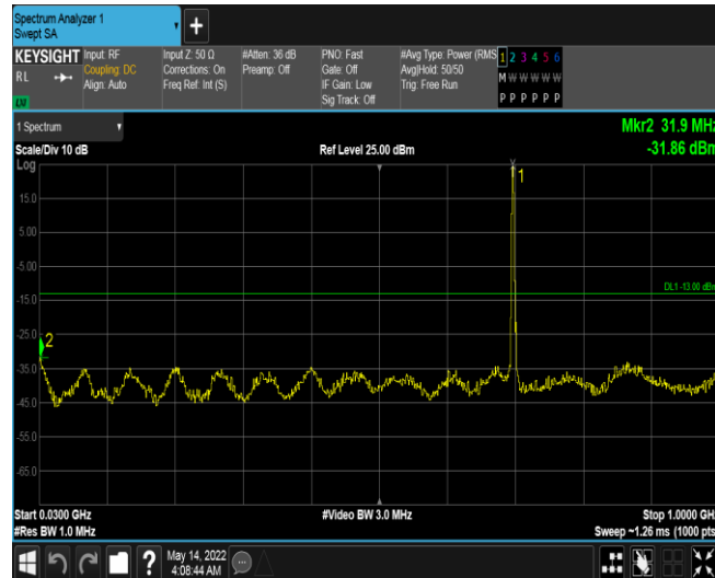
Band17-5MHz-QPSK-23755-1RB#0-Range1:30~1000MHz
