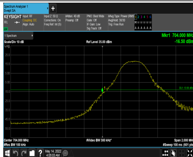
Band17-5MHz-16QAM-23755-1RB#24
