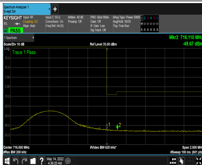
Band17-10MHz-QPSK-23800-1RB#49
