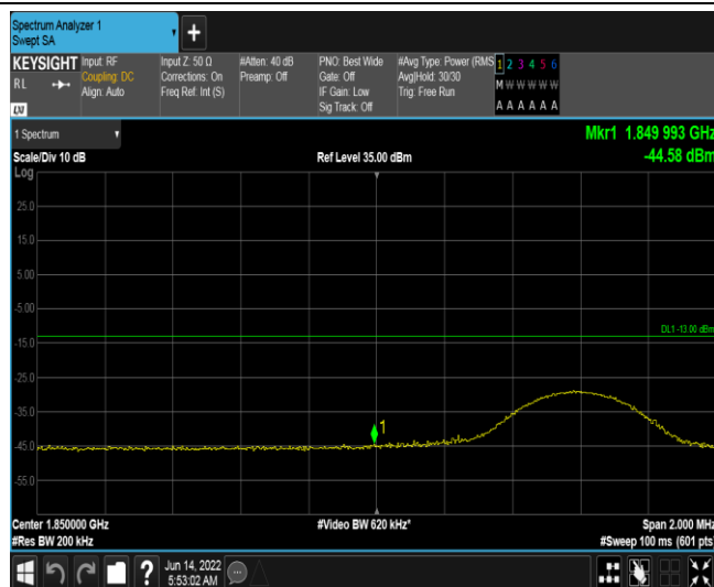
Band25-10MHz-QPSK-26090-50RB#0
