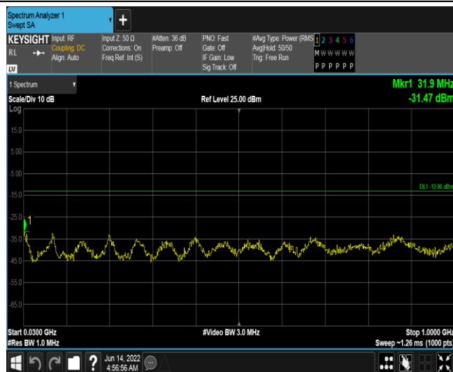
Band25-3MHz-16QAM-26055-1RB#0-Range1:30~1000MHz
