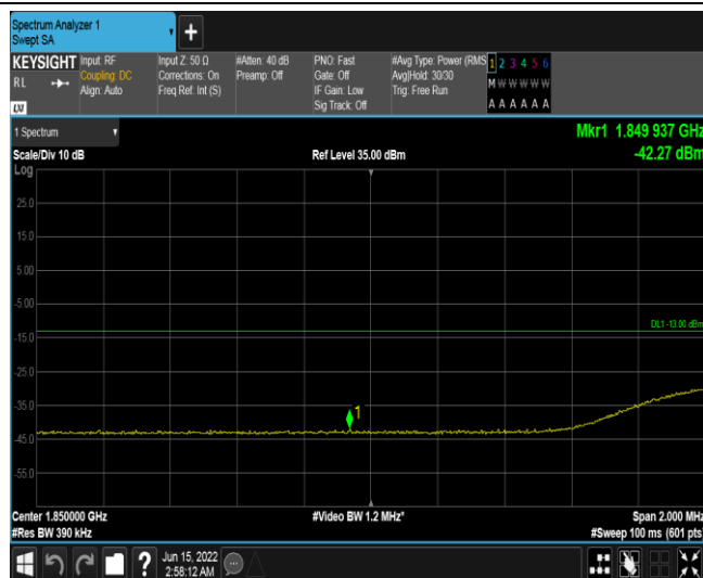
Band25-20MHz-16QAM-26140-100RB#0
