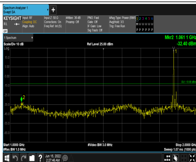
Band25-15MHz-16QAM-26365-1RB#0-Range3:2000~20000MHz
