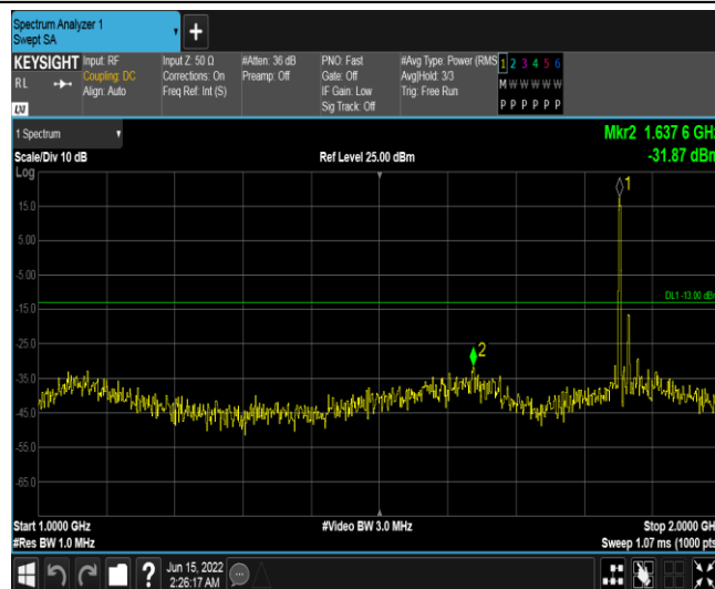
Band25-15MHz-16QAM-26115-1RB#0-Range2:1000~2000MHz
