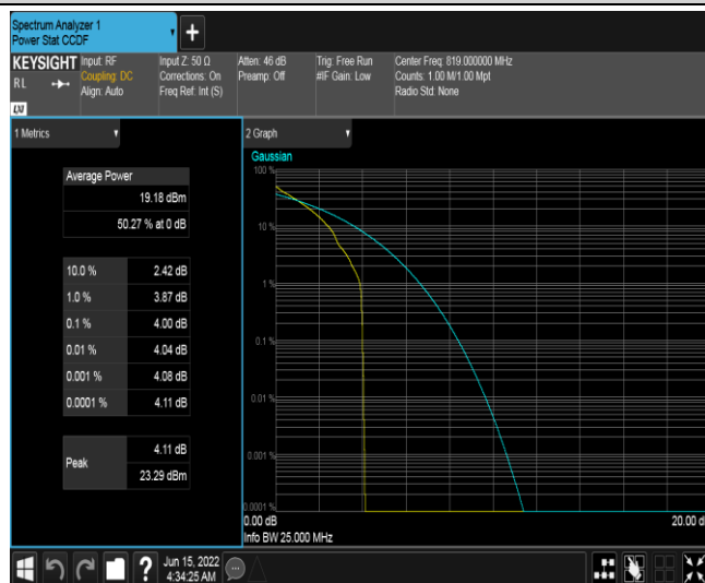
Band26-10MHz-QPSK-26740-1RB#0
