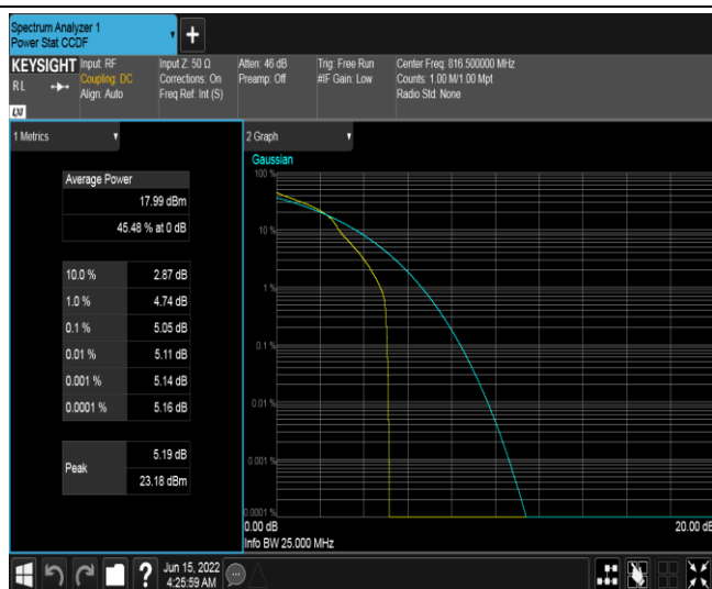
Band26-5MHz-16QAM-26715-25RB#0
