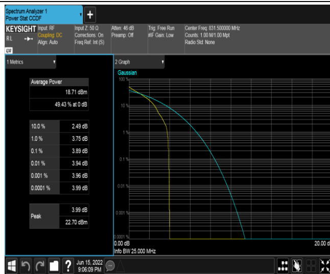
Band26-15MHz-QPSK-26865-75RB#0
