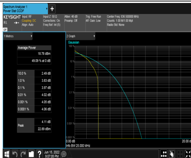
Band26-15MHz-QPSK-26915-1RB#0
