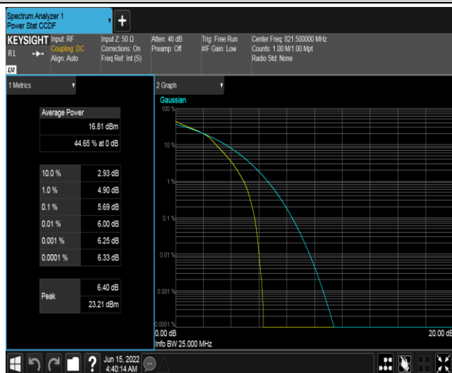
Band26-15MHz-16QAM-26765-75RB#0
