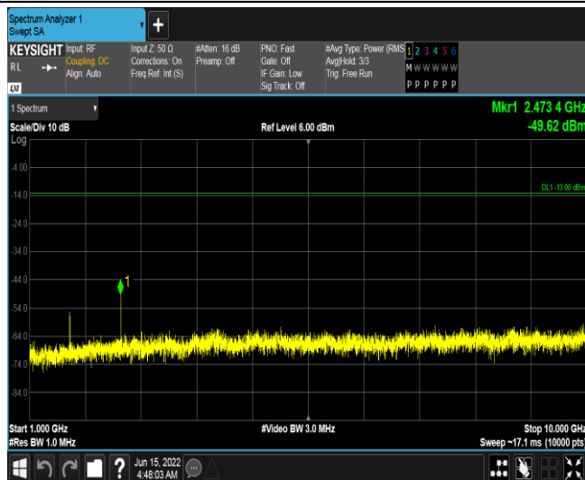
Band26-1.4MHz-16QAM-26797-1RB#0-Range3:1000~10000MHz
