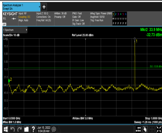
Band26-3MHz-16QAM-26805-1RB#0-Range2:30~1000MHz
