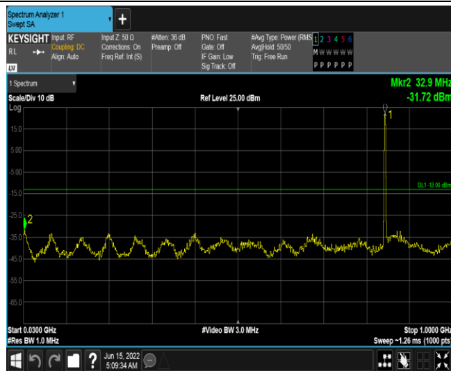
Band26-3MHz-16QAM-27025-1RB#0-Range2:30~1000MHz
