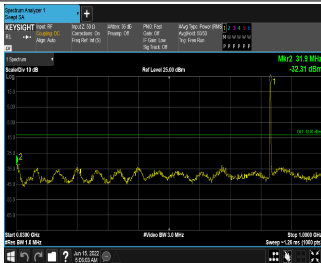
Band26-3MHz-QPSK-26915-1RB#0-Range2:30~1000MHz
